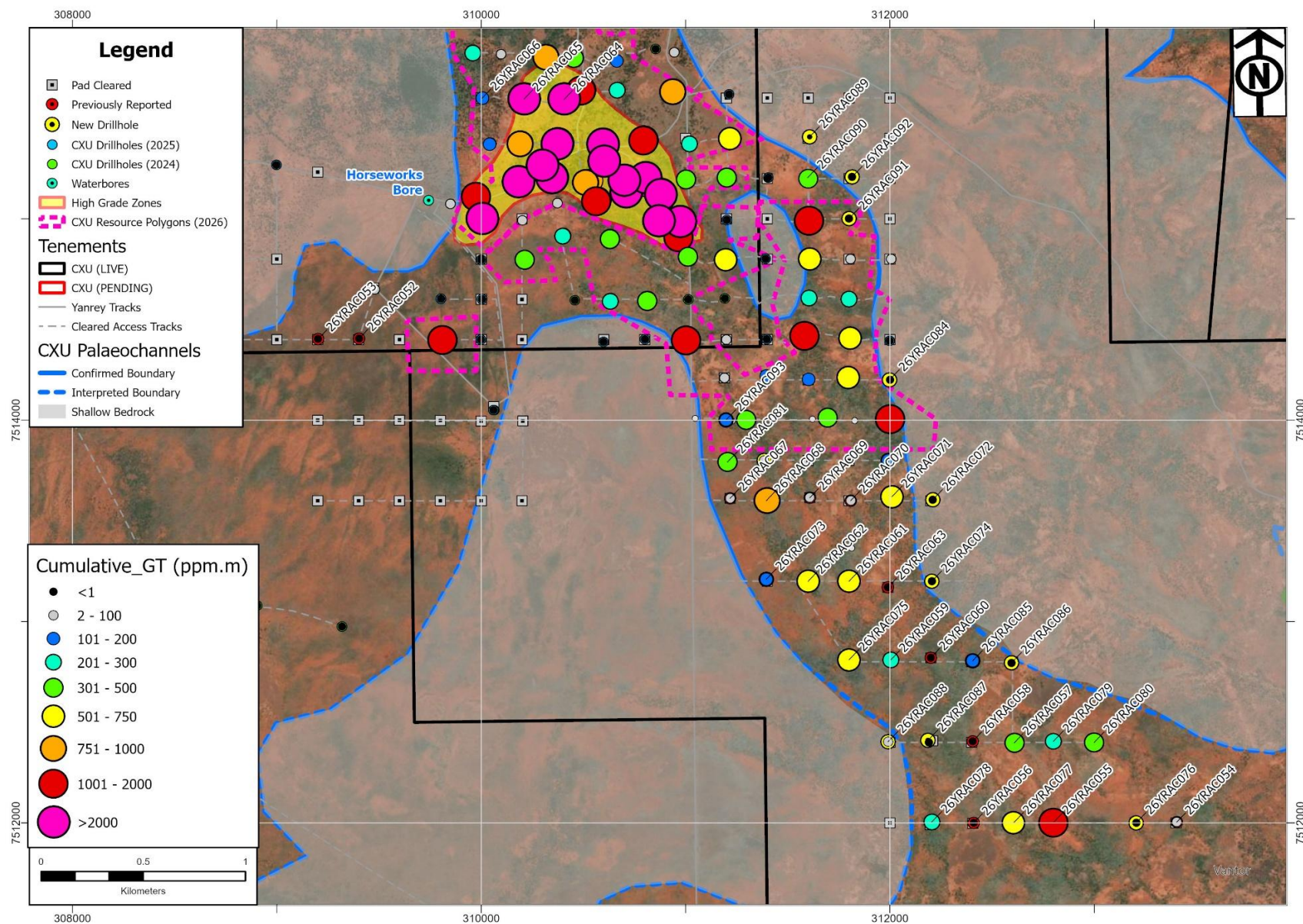
Figure 6. Manyingee South Cumulative GT (ppm*m) map.
