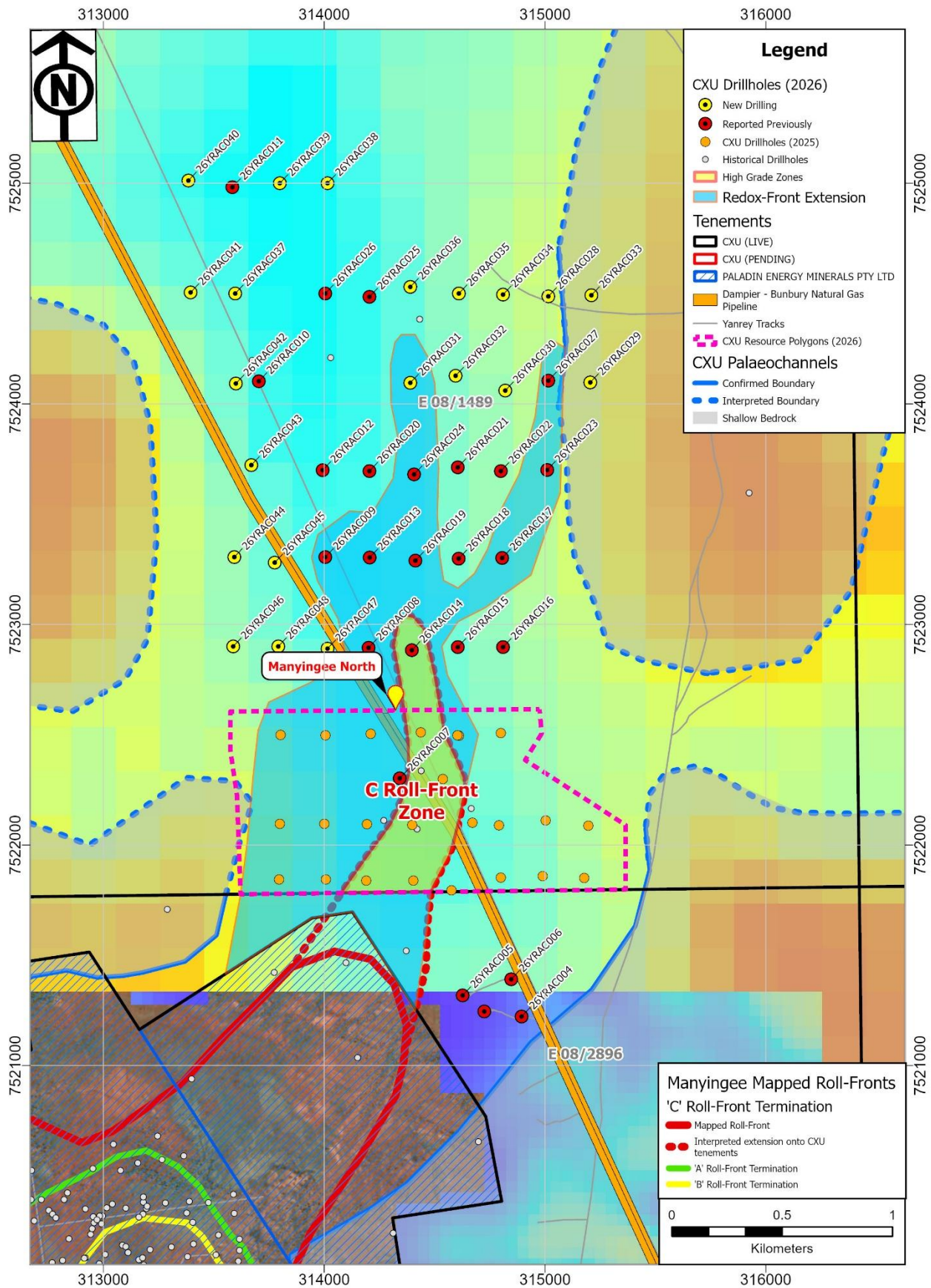
Figure 8. Manyingee North showing completed drillhole locations and passive seismic survey interpreted depth to bedrock surface.
