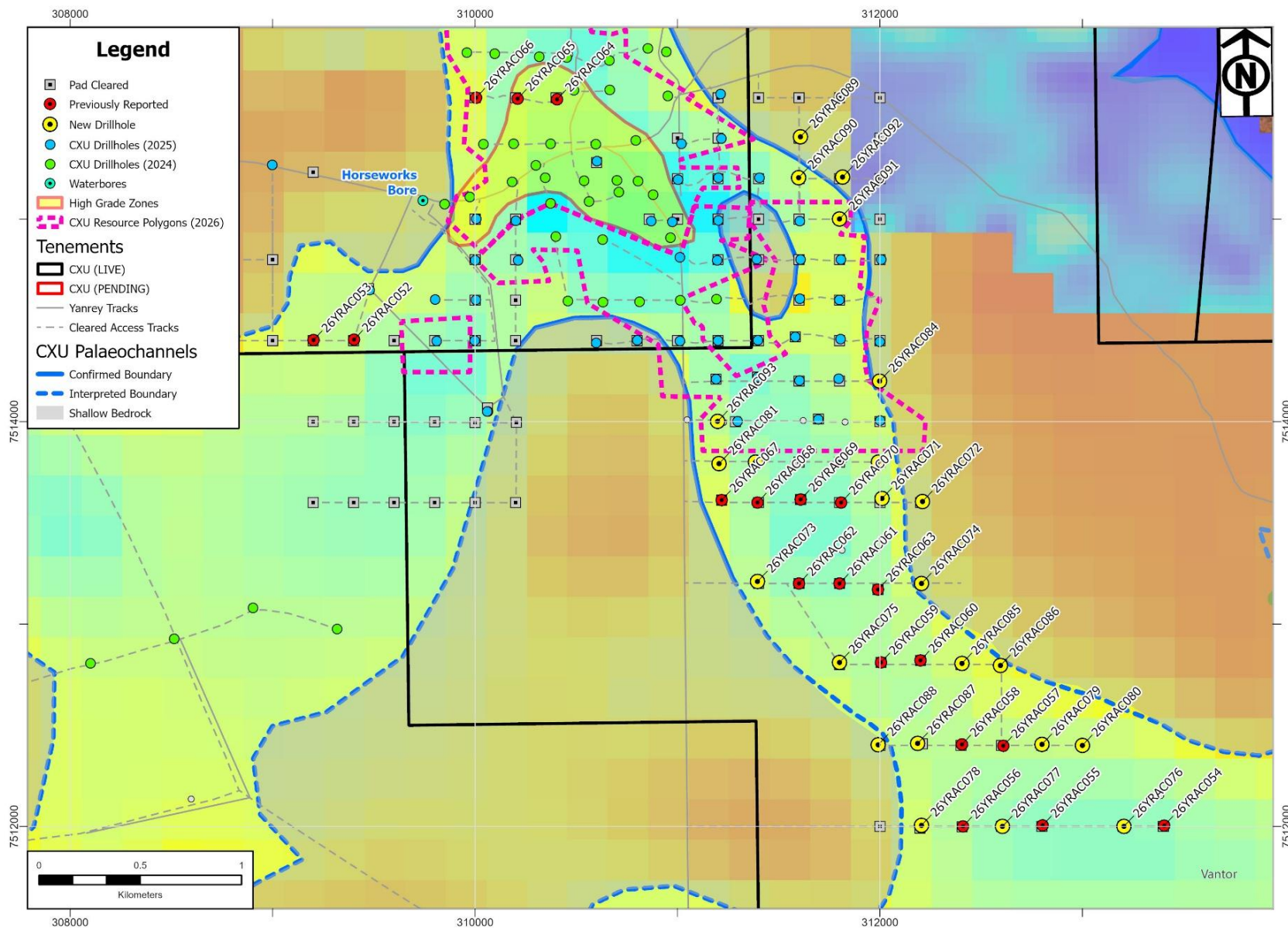
Figure 5. Manyingee South passive seismic interpreted depth to bedrock map showing drillhole locations.
