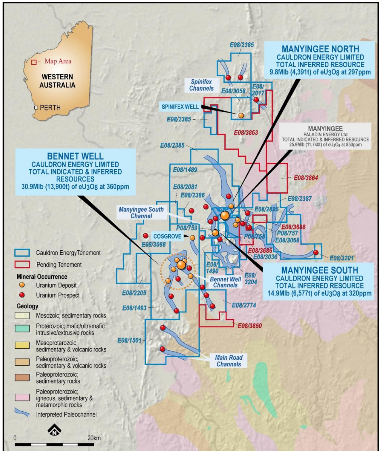
Figure 2. Yanrey Uranium Project regional geology.
