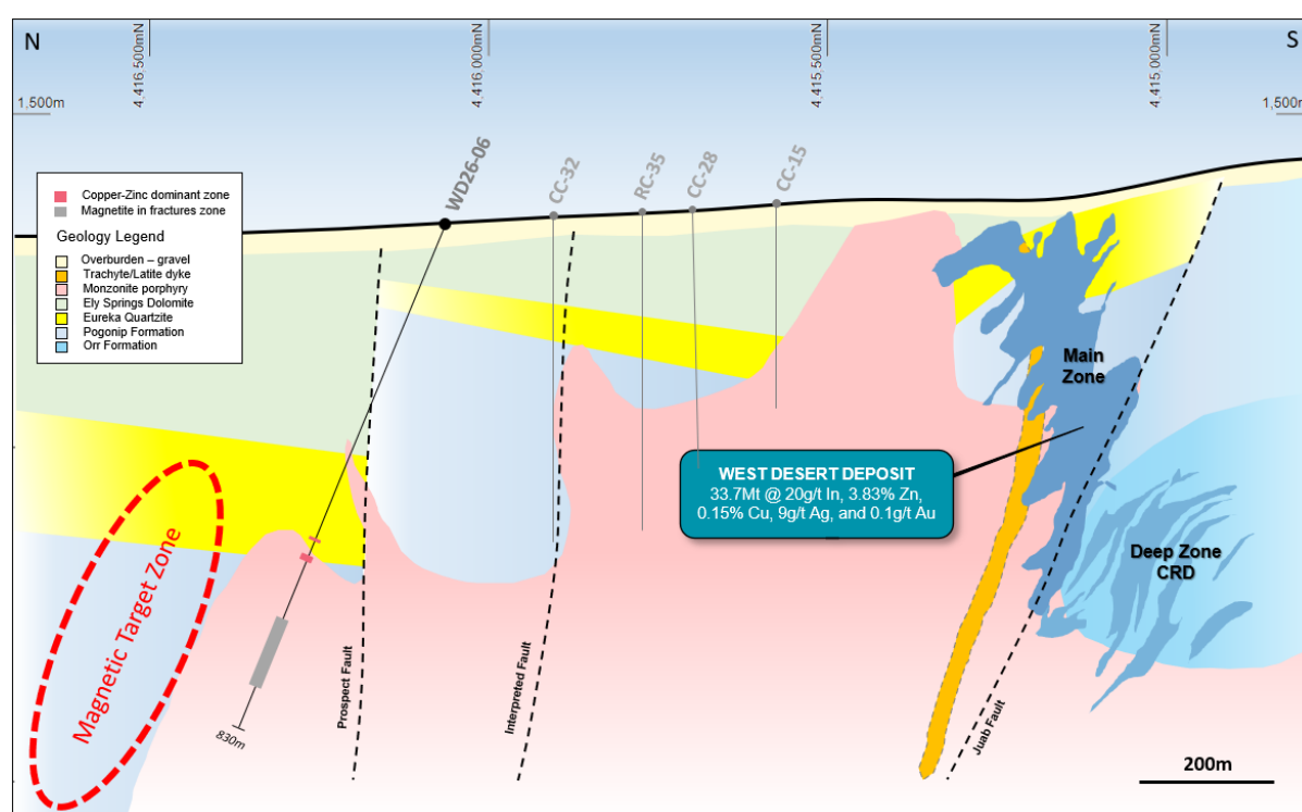
Figure 8: Schematic geological section at 289,025E (+/-200m) showing main geological units and WD26-06 drill trace.
