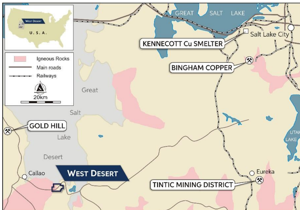
Figure 10: Location of the West Desert Project.
