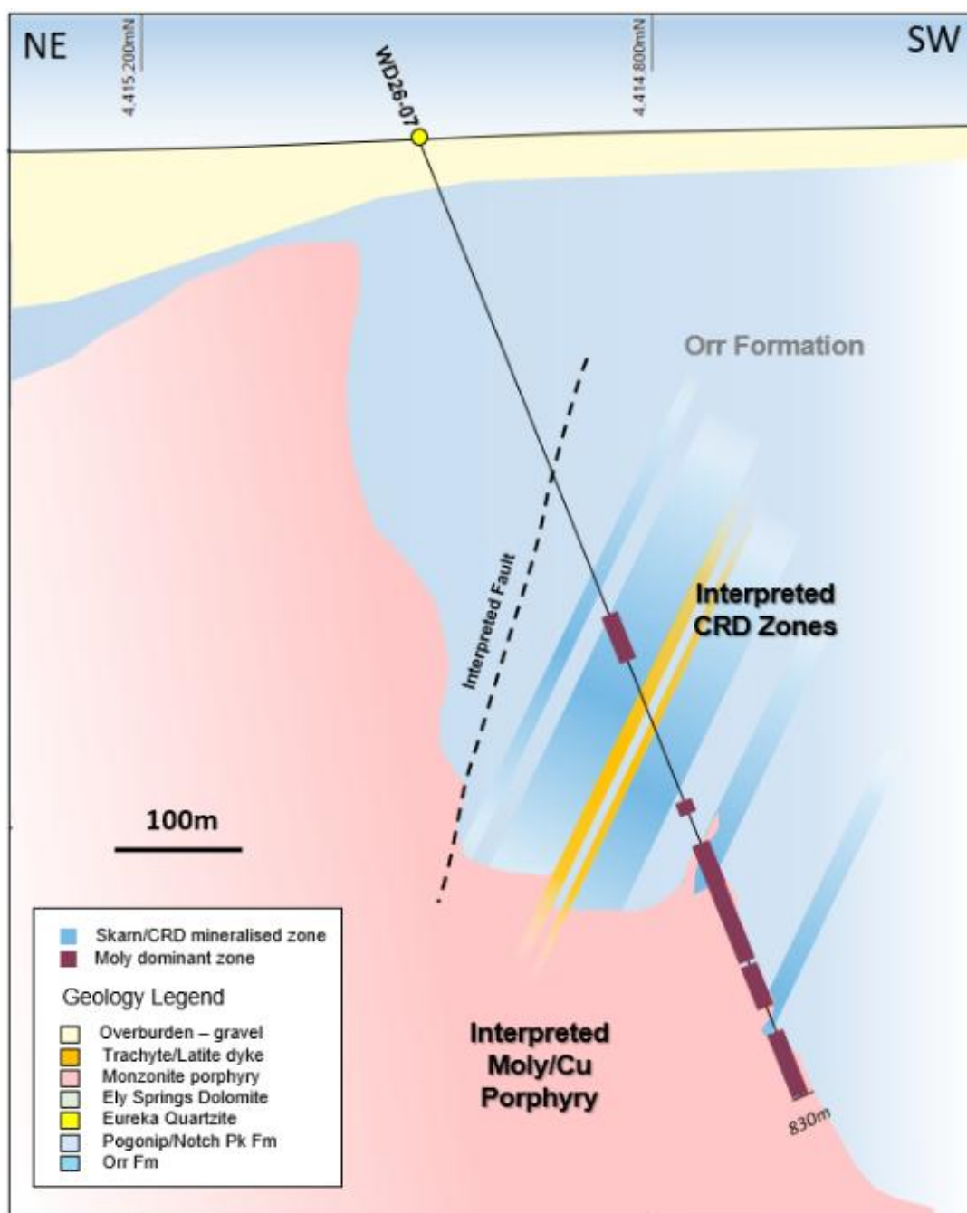
Figure 7: Schematic NE-SW geological section through drill hole WD26-07 (+/-100m) showing main geological units and drilling. A simplification of the mineralised intervals is shown.
