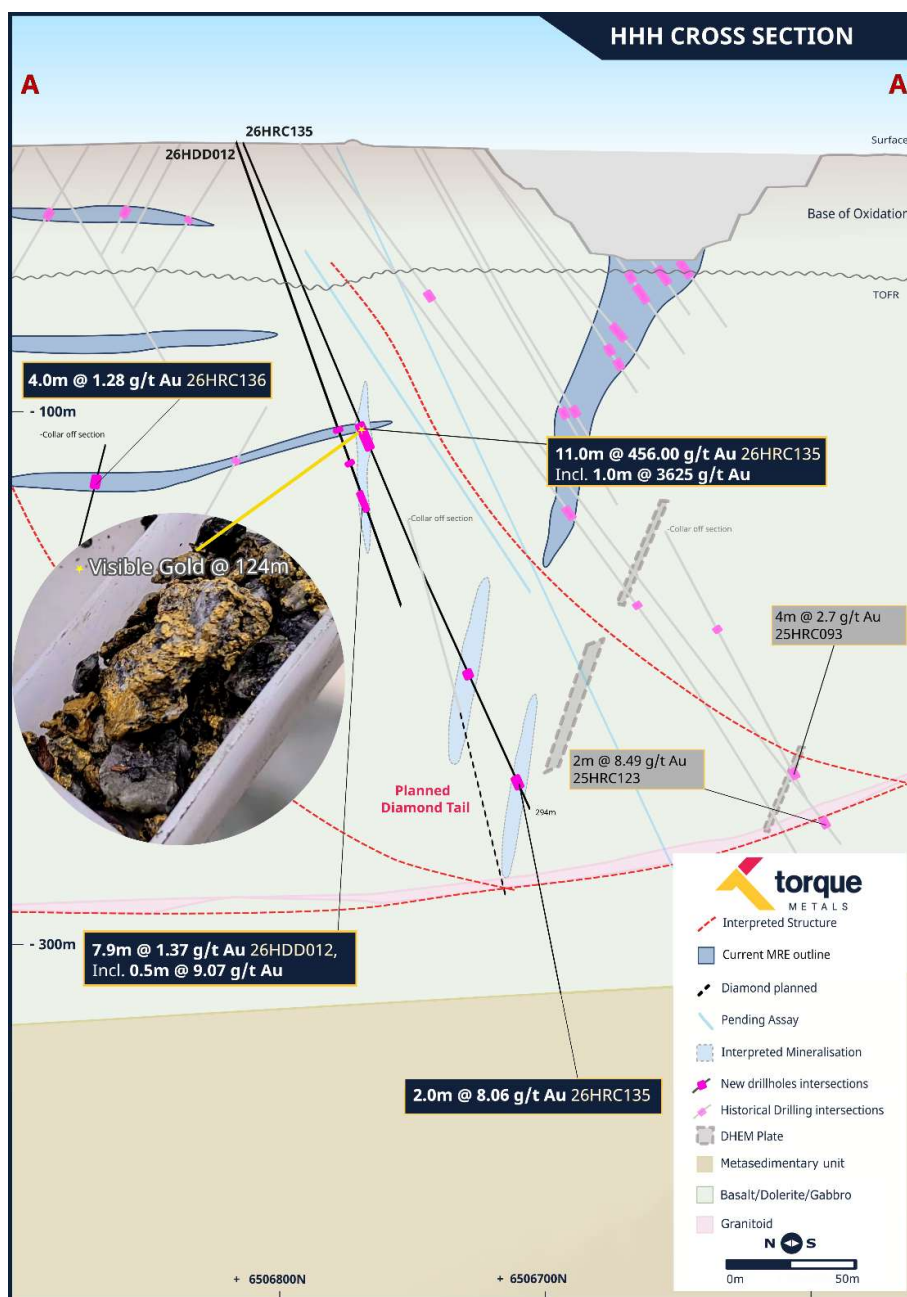
Figure 1: Cross-section of RC hole 26HRC135 showing the large visible gold "nuggets" in the chip tray. The hole intersected multiple interpreted structures.
