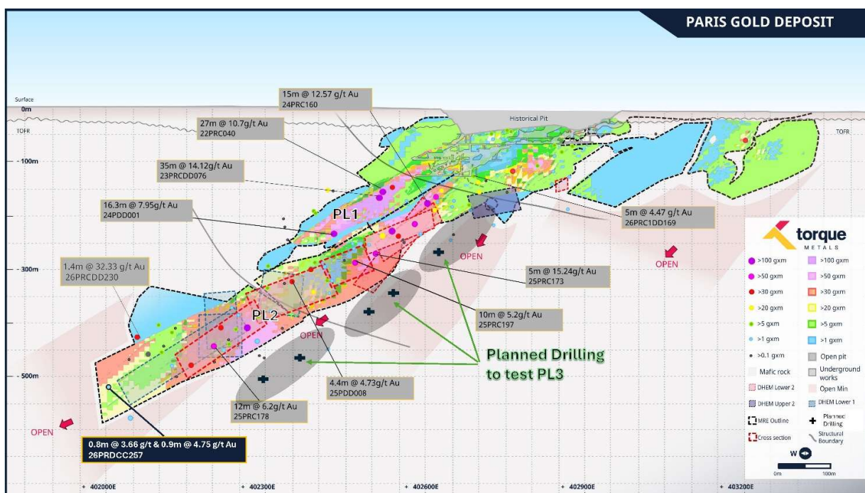
Figure 4: Long section of the Paris Deposit showing recently released results and interpreted PL3 position
