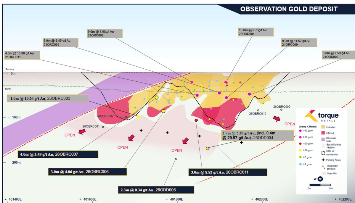
Figure 3: Long section of Observation Gold Deposit showing recent RC results
