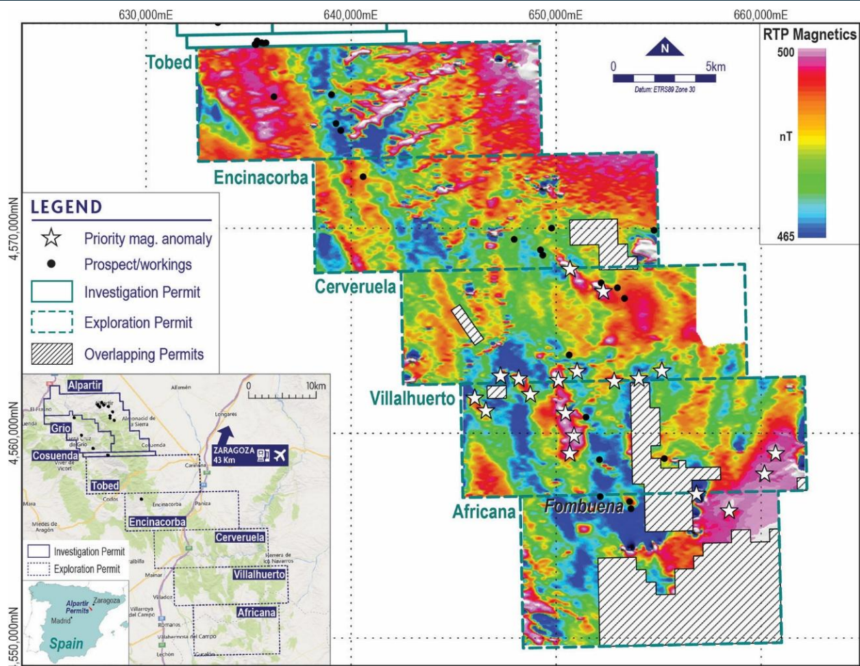
Figure 6 – Total Field Anomaly map with reduction-to-the-pole filter applied.
