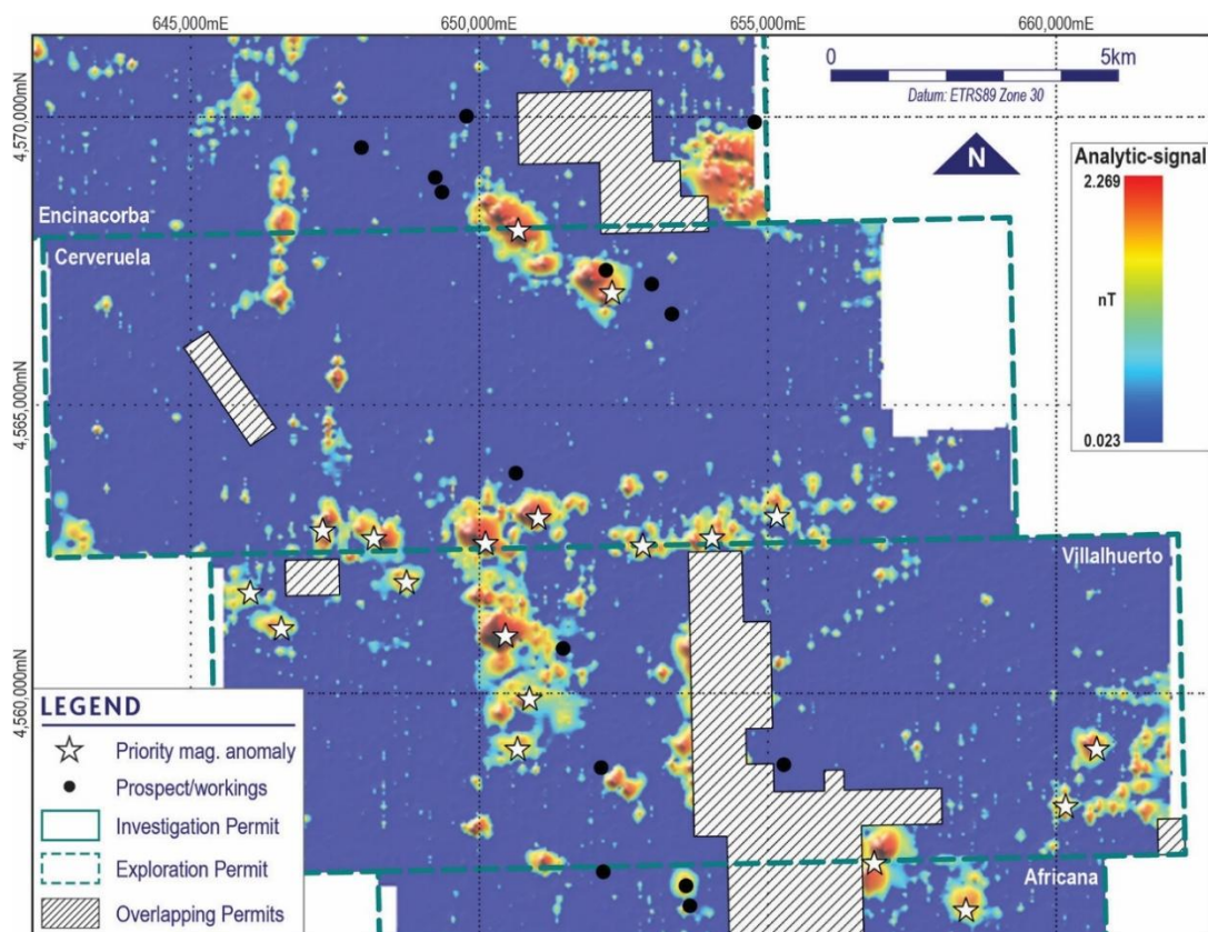
Figure 7 – Total Field Anomaly map with analytic-signal filter applied. Priority anomalies highlighted.
