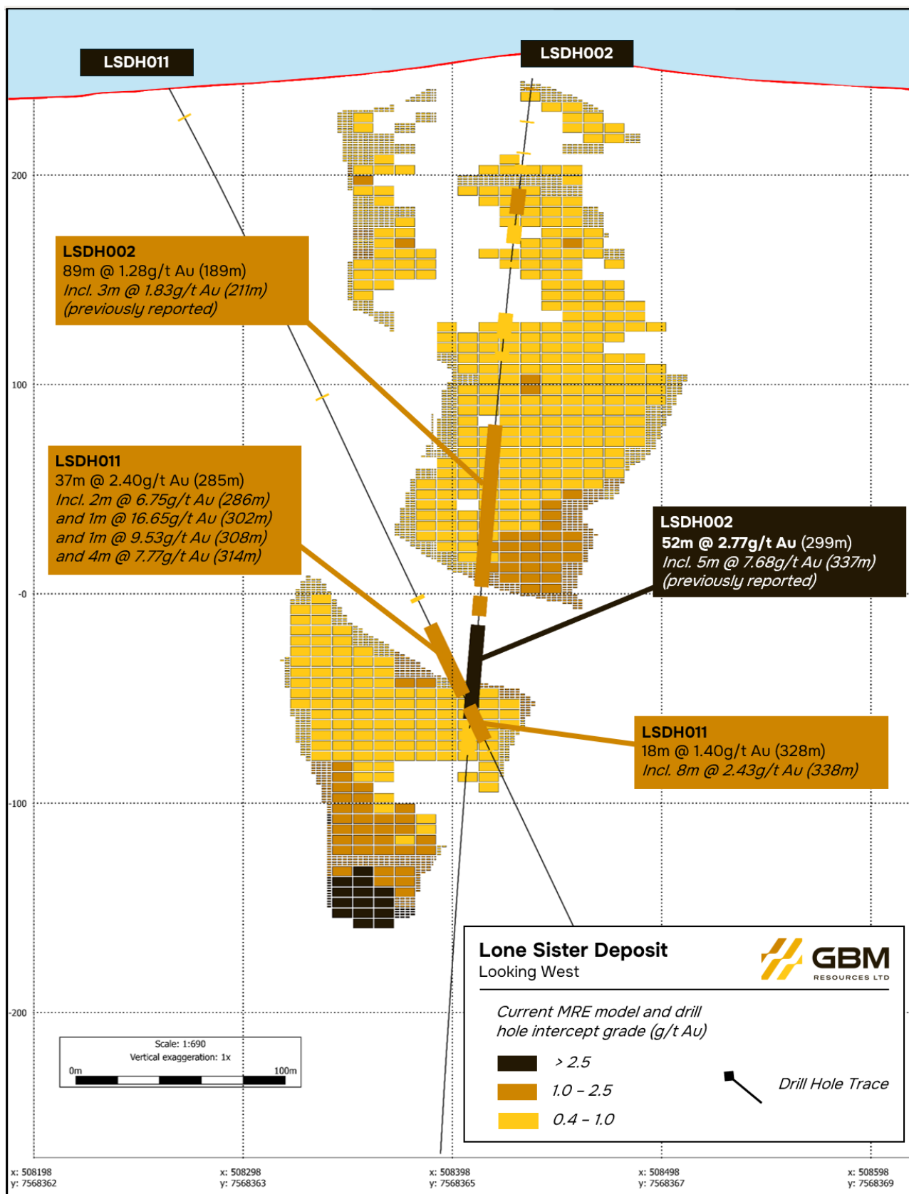
Figure 3 – Cross section of drill hole LSDH011 at the Lone Sister deposit.
