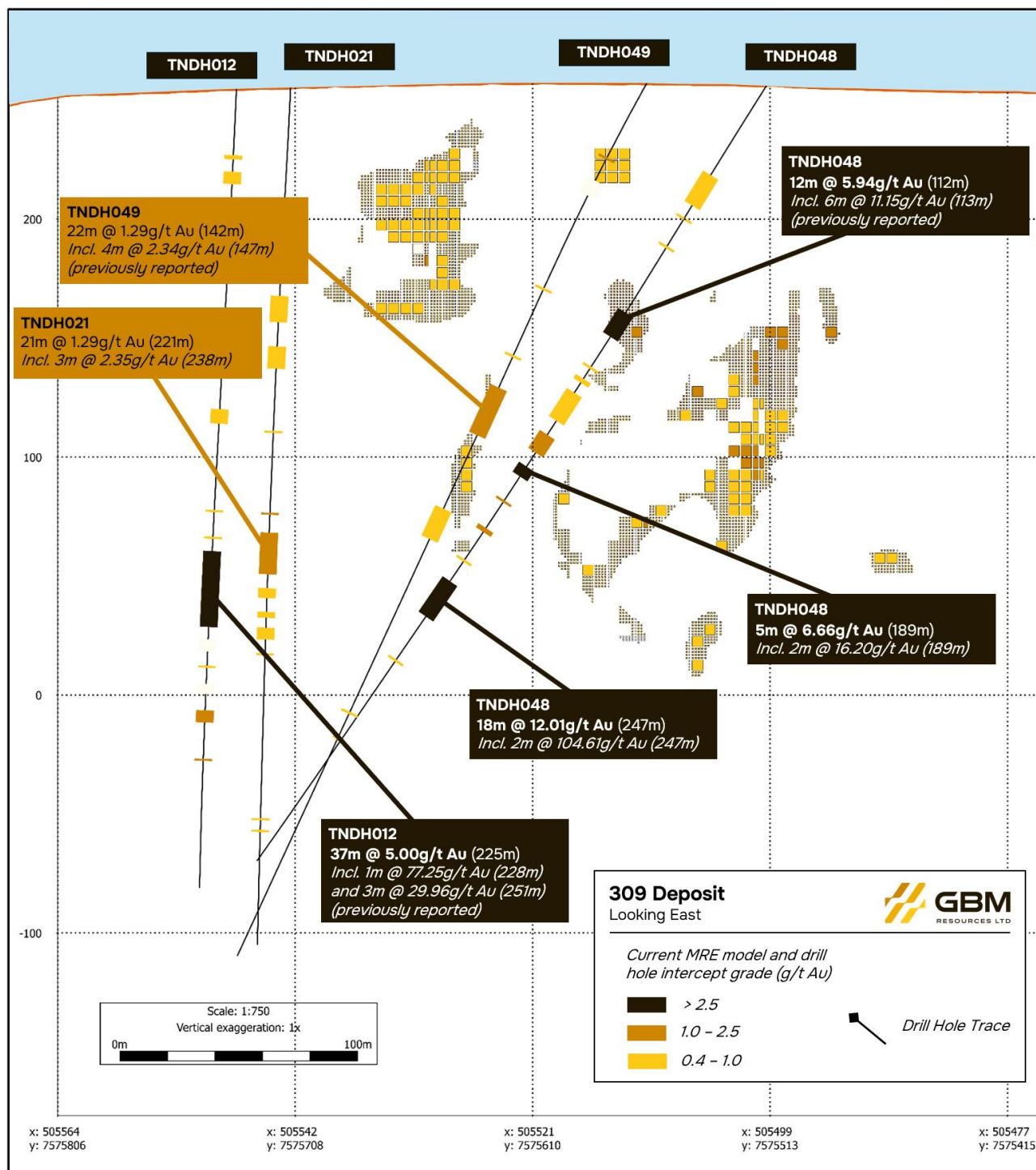
Figure 1 – Cross section of drill hole TNDH048 at the 309 deposit.
