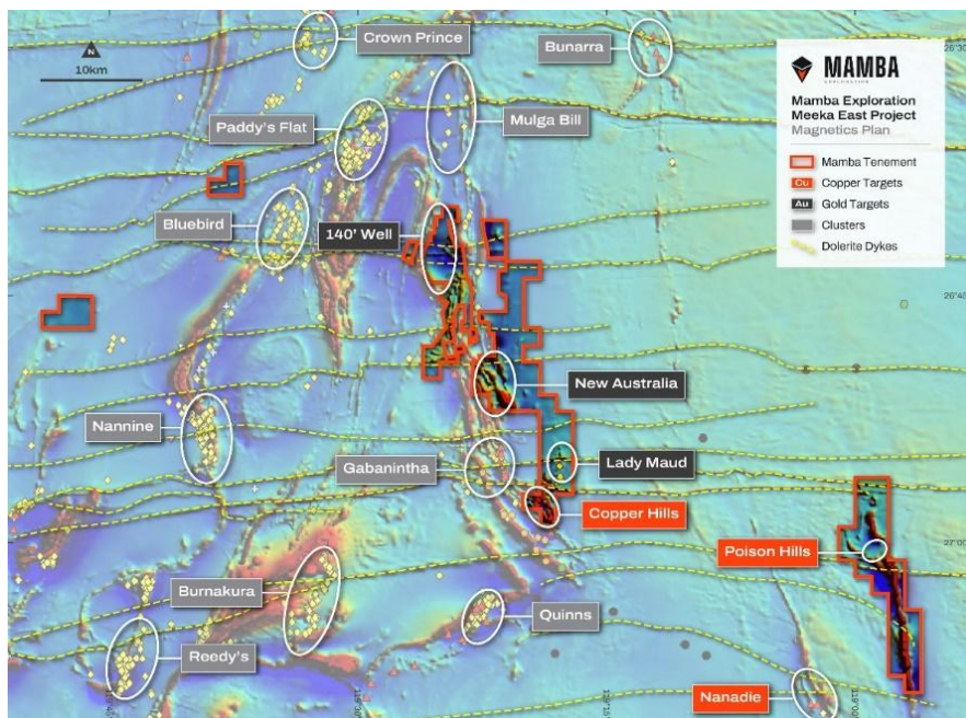
Figure 1 Meeka East Project magnetics plan showing 140 Foot Well, New Australian and Lady Maud, the Copper Hills–Lady Alma corridor and Poison Hills, with the regional gold deposits referenced in this announcement.
