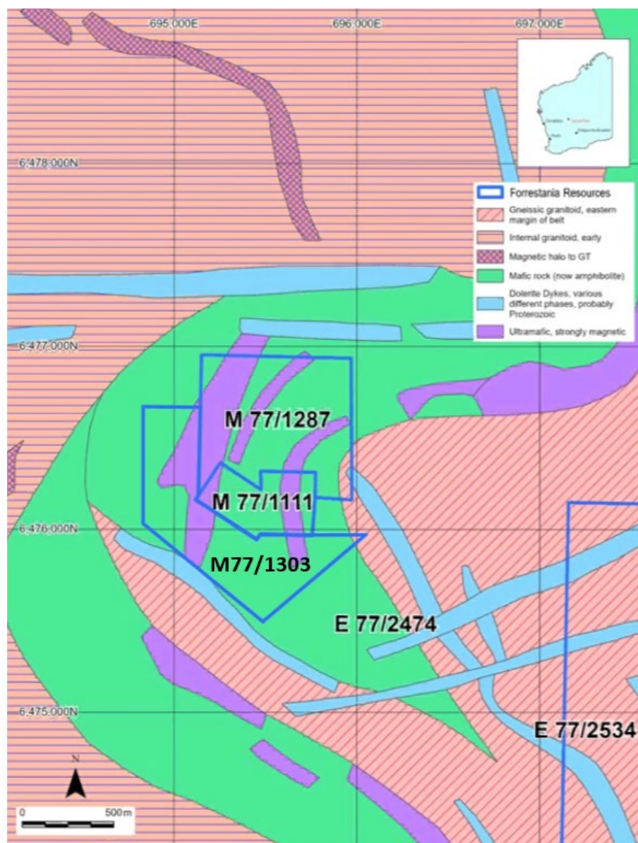
Figure 3: Geology of the Symes Find Area
