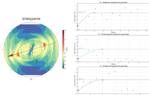
Figure 7: Variogram Models
