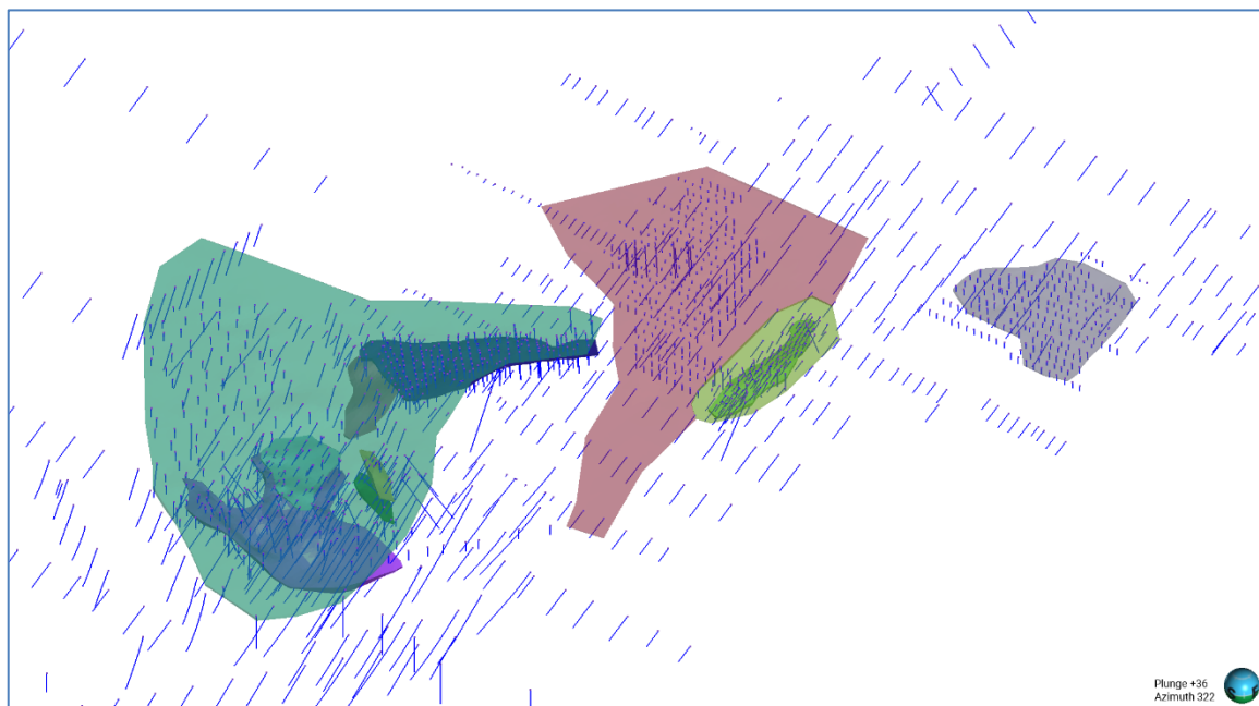
Figure 4: Perspective View of Model Wireframes and Drilling Data
