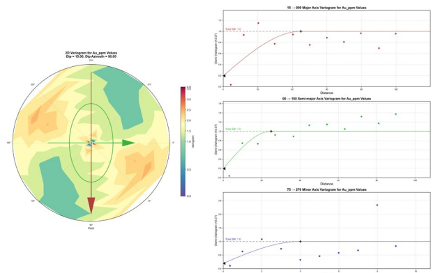
Figure 7: Variogram Models
