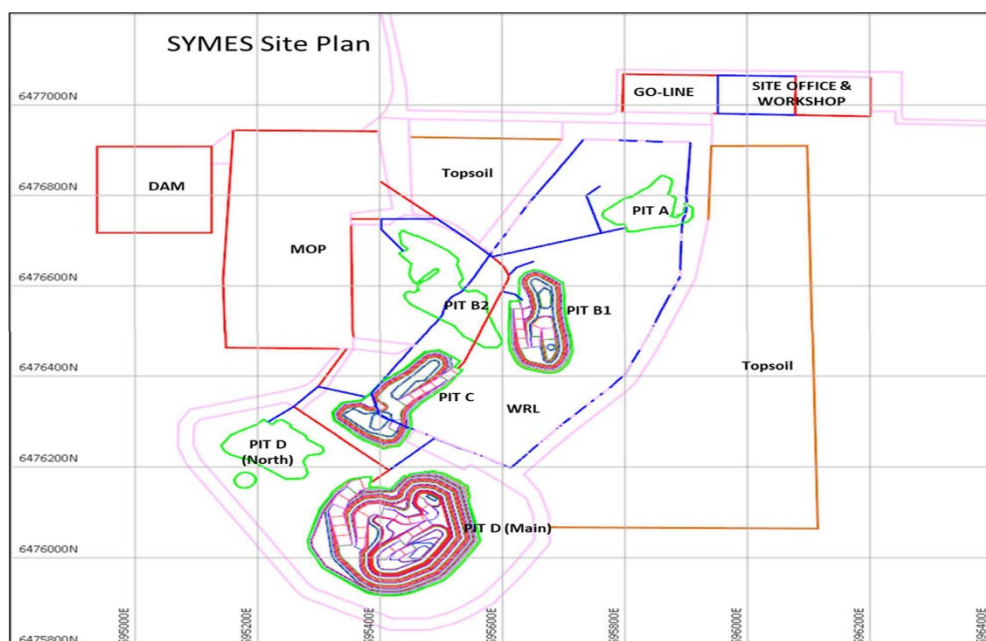
Figure 9: PFS Symes Find Proposed Site Layout
