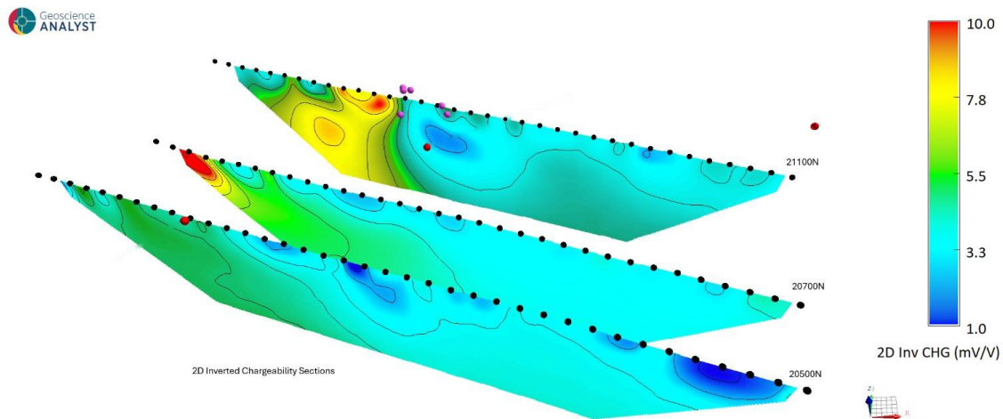
Figure 9. Three-dimensional perspective view (looking north) of the 2D inverted chargeability sections for lines 21100N, 20700N and 20500N. Elevated chargeability is concentrated towards the western ends of all three lines, immediately west of the Silver Valley 2 workings. Red dots are known mineral occurrences and pink dots are mapped old workings.
