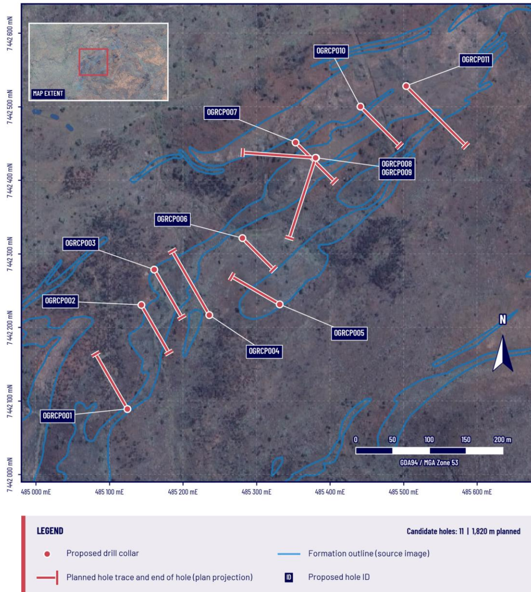
Figure 7. Oonagalabi Main Zone proposed drill collars and planned hole traces over the georeferenced Oonagalabi Formation image. Blue formation outlines are retained from the base image. Coordinates are GDA94 / MGA Zone 53. Inset shows the map extent within the full image. Traces connect planned collars and end-of-hole positions in plan projection and are not surveyed trajectories. Formation outlines do not define mineralisation limits. Hole IDs are numbered southwest to northeast along the Main Zone and do not indicate drilling order or individual hole priority.
