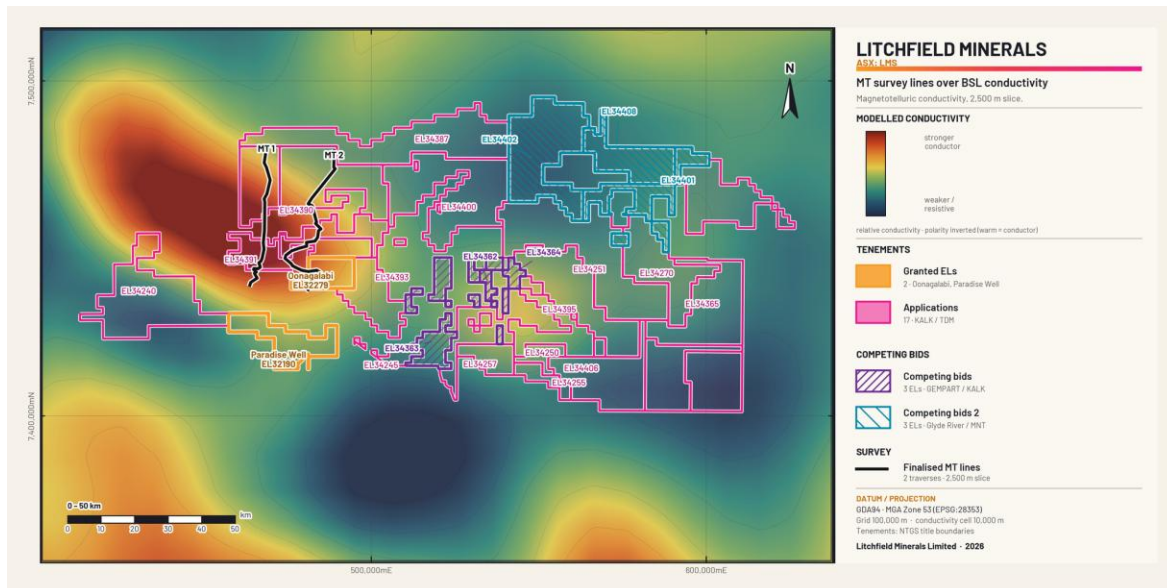
Figure 8. Finalised MT survey lines (MT 1 and MT 2) over modelled conductivity, 2,500m slice (relative, polarity inverted so warm tones indicate stronger conductors). GDA94 MGA Zone 53 (EPSG:28353).
