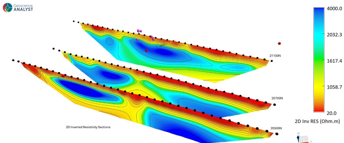
Figure 10. Three-dimensional perspective view (looking north) of the 2D inverted resistivity sections. Deeper low-resistivity zones on the southern lines 20700N and 20500N sit beneath and to the west of the elevated chargeability and may be mapping the interpreted western structural corridor. Red dots are known mineral occurrences and pink dots are mapped old workings.
