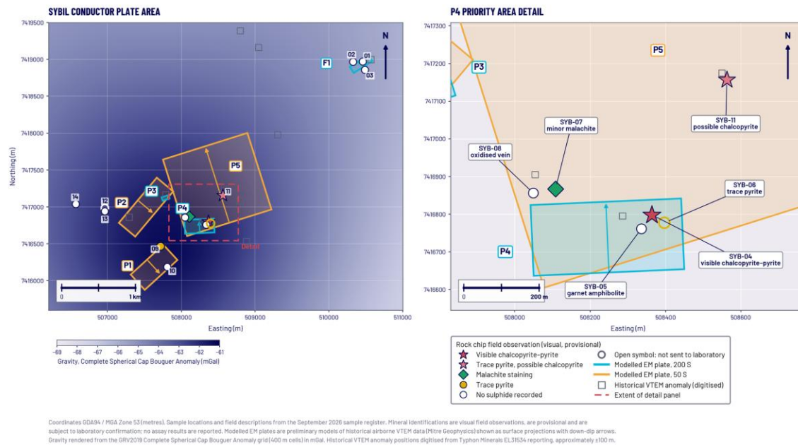
Figure 3. Sybil rock chip locations from the September 2026 sample register plotted over the preliminary modelled EM conductor plates on a regional gravity background, shown as a zoomed-out view of the Sybil conductor plate area (left) and a zoomed-in view of the P4 priority area (right). Coloured polygons are the conductor plates modelled by Mitre Geophysics from historical VTEM data; small grey squares are the historical Mithril Resources VTEM anomaly positions. Mineral identifications are visual field observations and hence are provisional and subject to laboratory confirmation; no assay results are reported.
