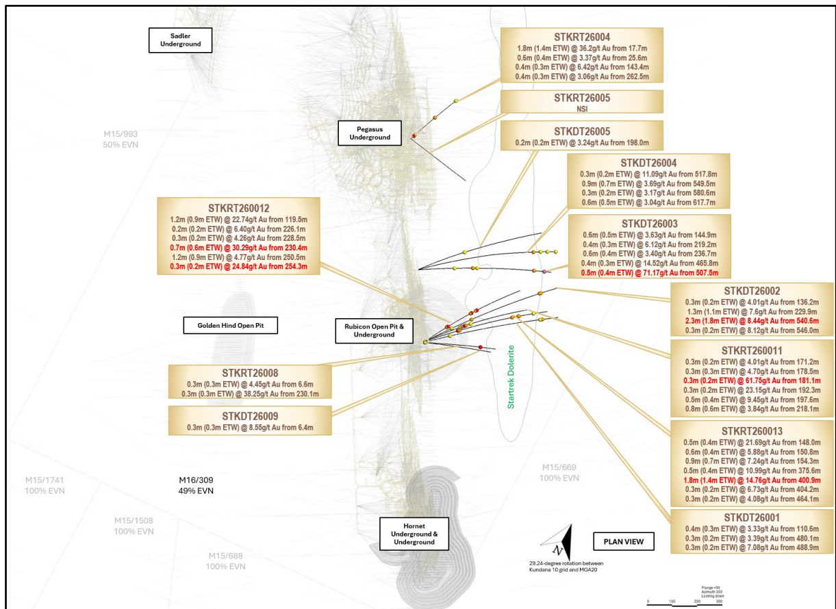
Figure 1 A Plan view of the assay results location returned from within the quarter for Star Trek. Image provided in K10 Mine Grid.
