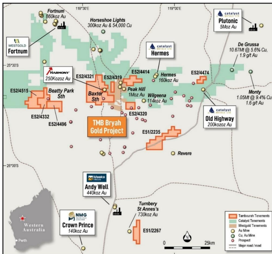
Figure 2 Location plan showing Tambourah's Bryah Gold Project tenements and prospects.
