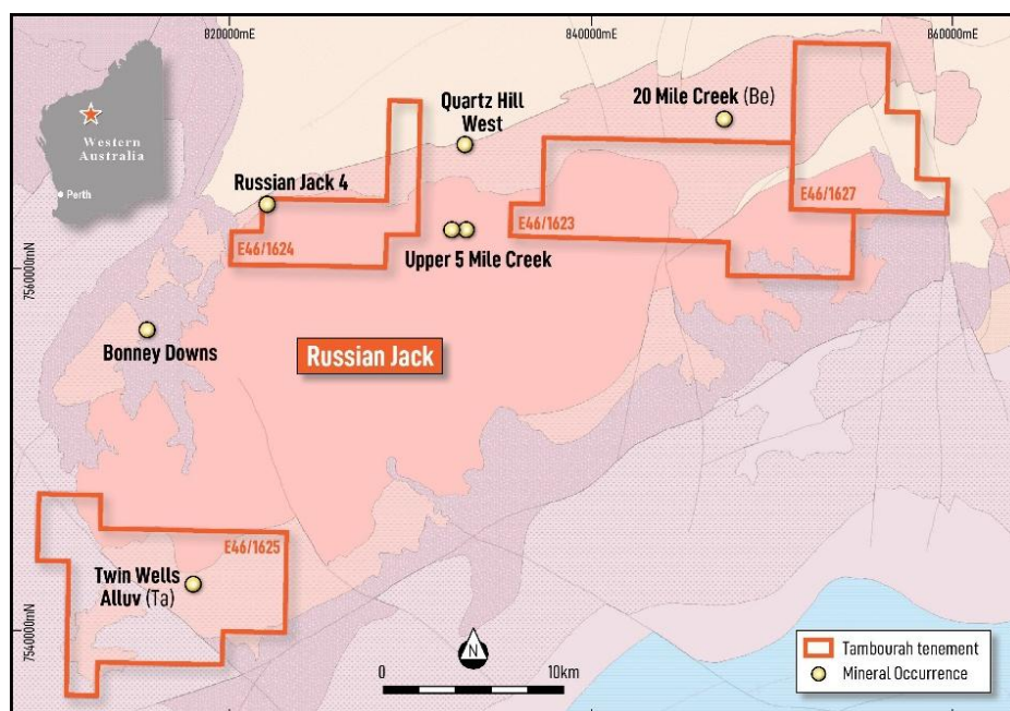
Figure 10 Kurrana project tenements adjacent to the contact of the Bonney Downs Monzogranite.
