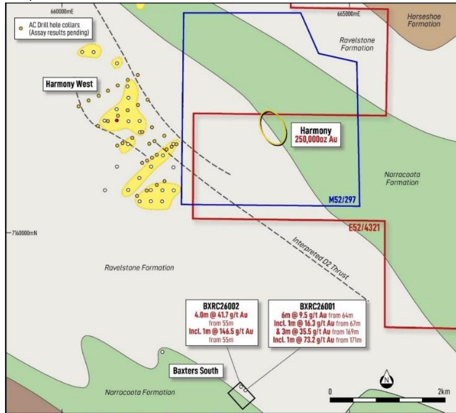
Figure 4: Baxter Sth location plan showing gold targets
