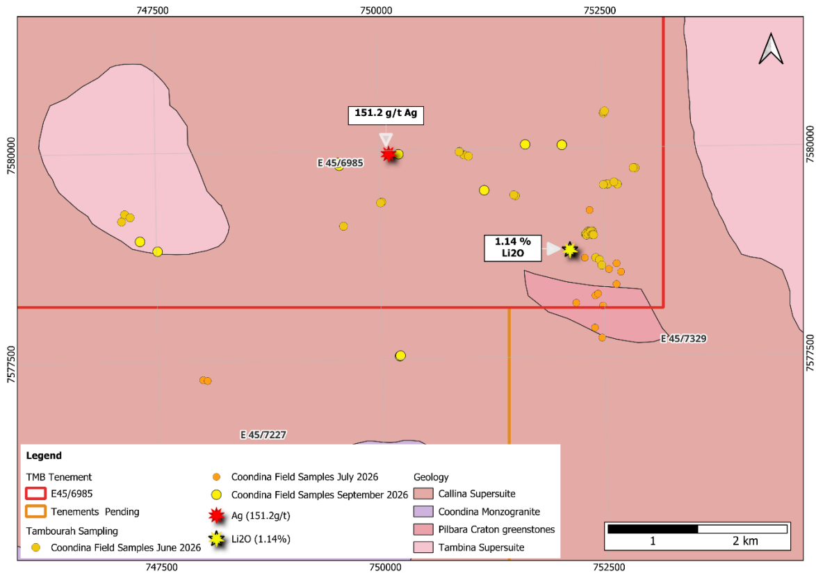
Figure 8 Coondina project geology, sample locations showing Silver and LCT anomalies.
