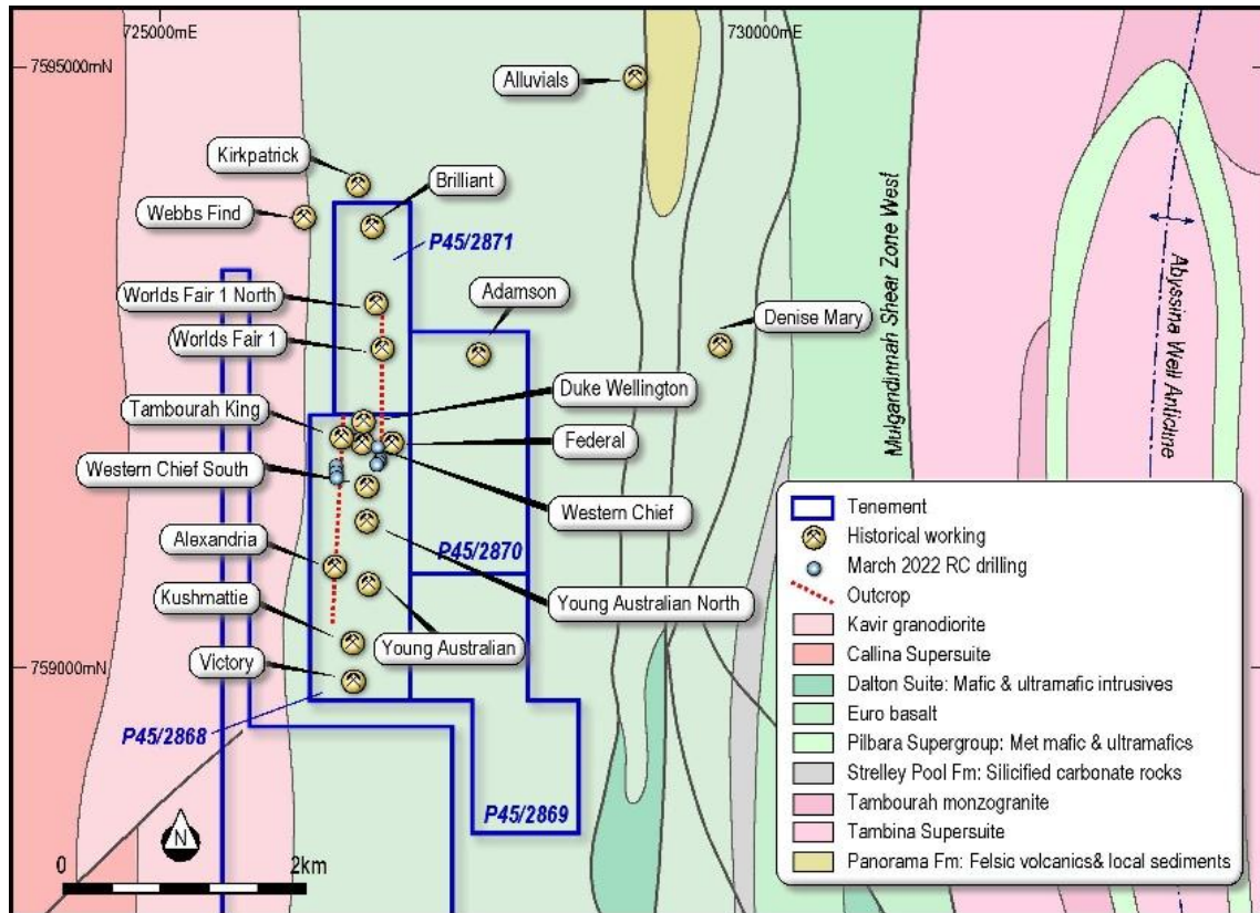
Figure 5 Tambourah Gold Project prospect plan.
