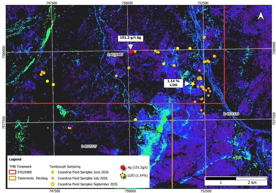
Figure 9 Coondina project hyperspectral, showing Silver and LCT anomalies.
