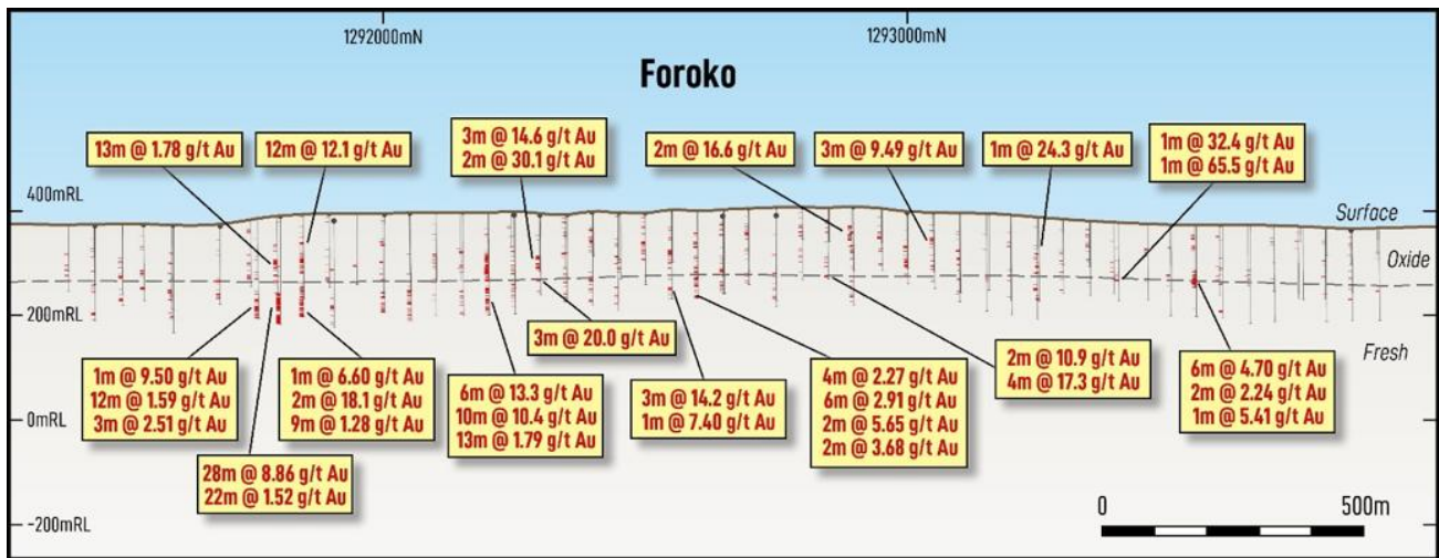
Figure 8: Long Section Showing Drilling Results at Foroko
