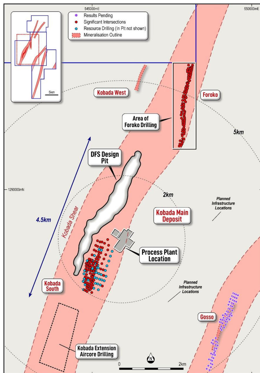
Figure 7: Plan Showing RC drilling at Foroko, Gosso and Kobada South Completed During 2026
