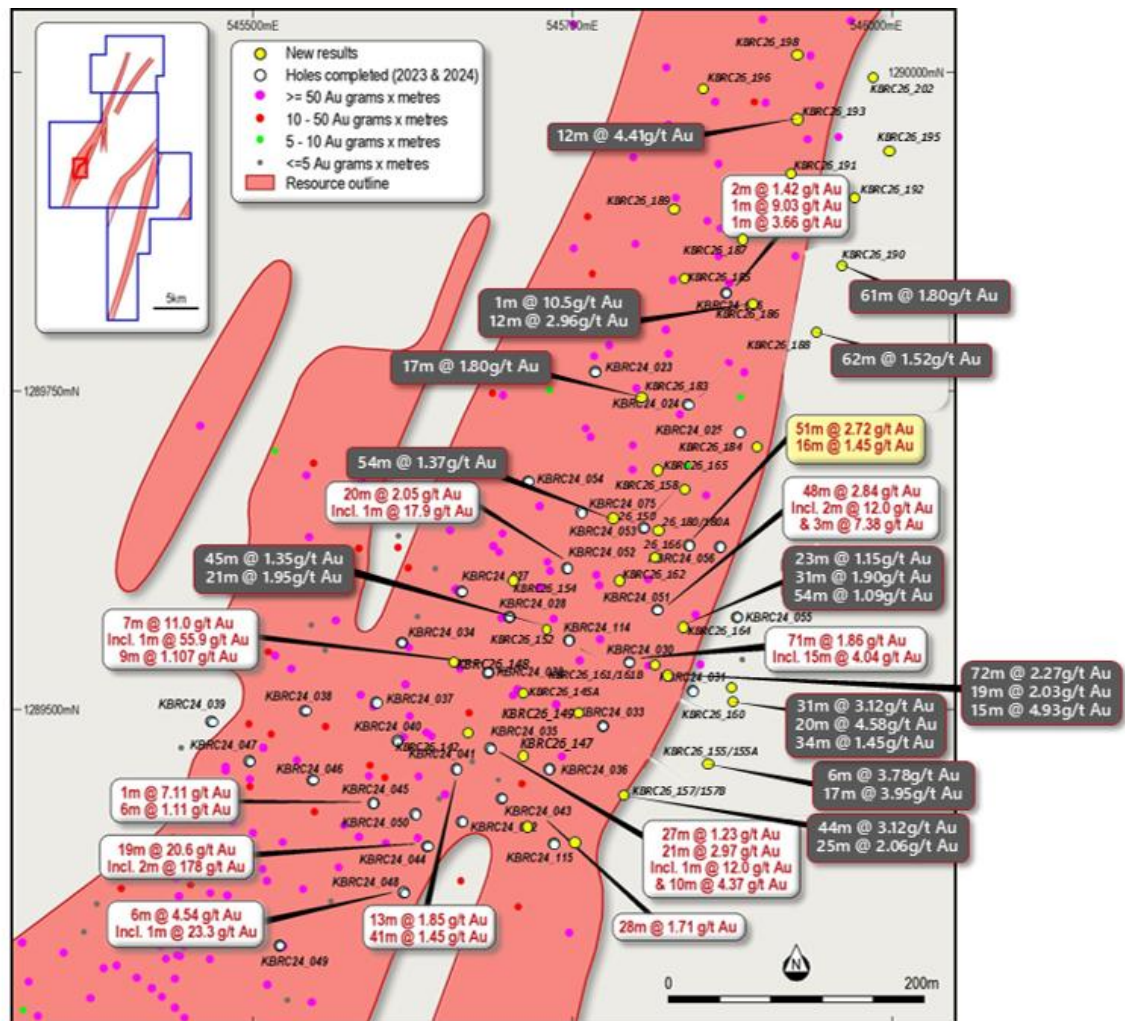
Figure 9: Plan Showing Infill Drilling Results at Kobada Reported During the Quarter
