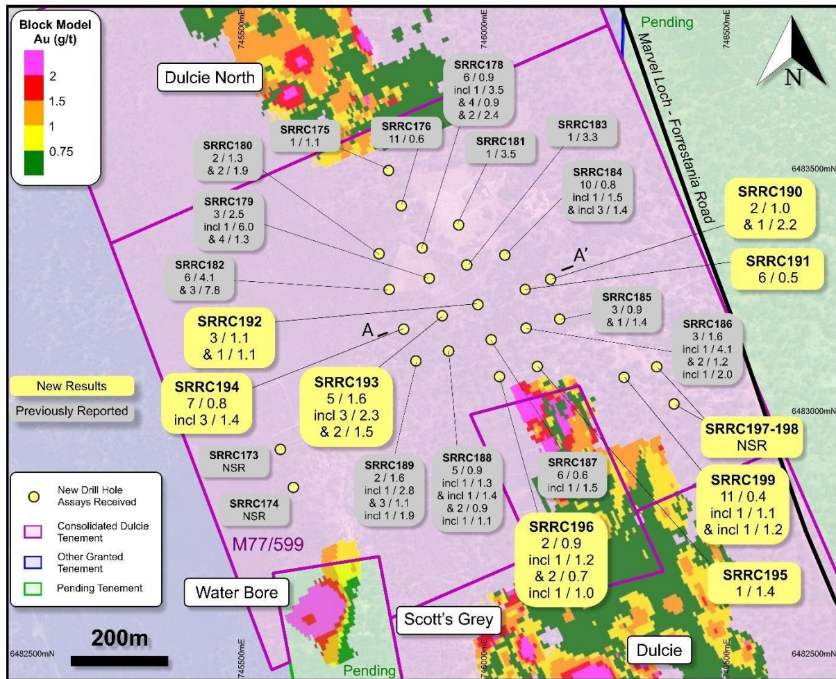
Figure 4: Dulcie Central plan showing the RC holes completed between Dulcie North and Dulcie within M77/599, outside the current Mineral Resource, with results reported during and after the quarter (refer ASX announcements 25 September, 15 October and 27 October 2026). Down-hole widths; true widths not yet determined.
