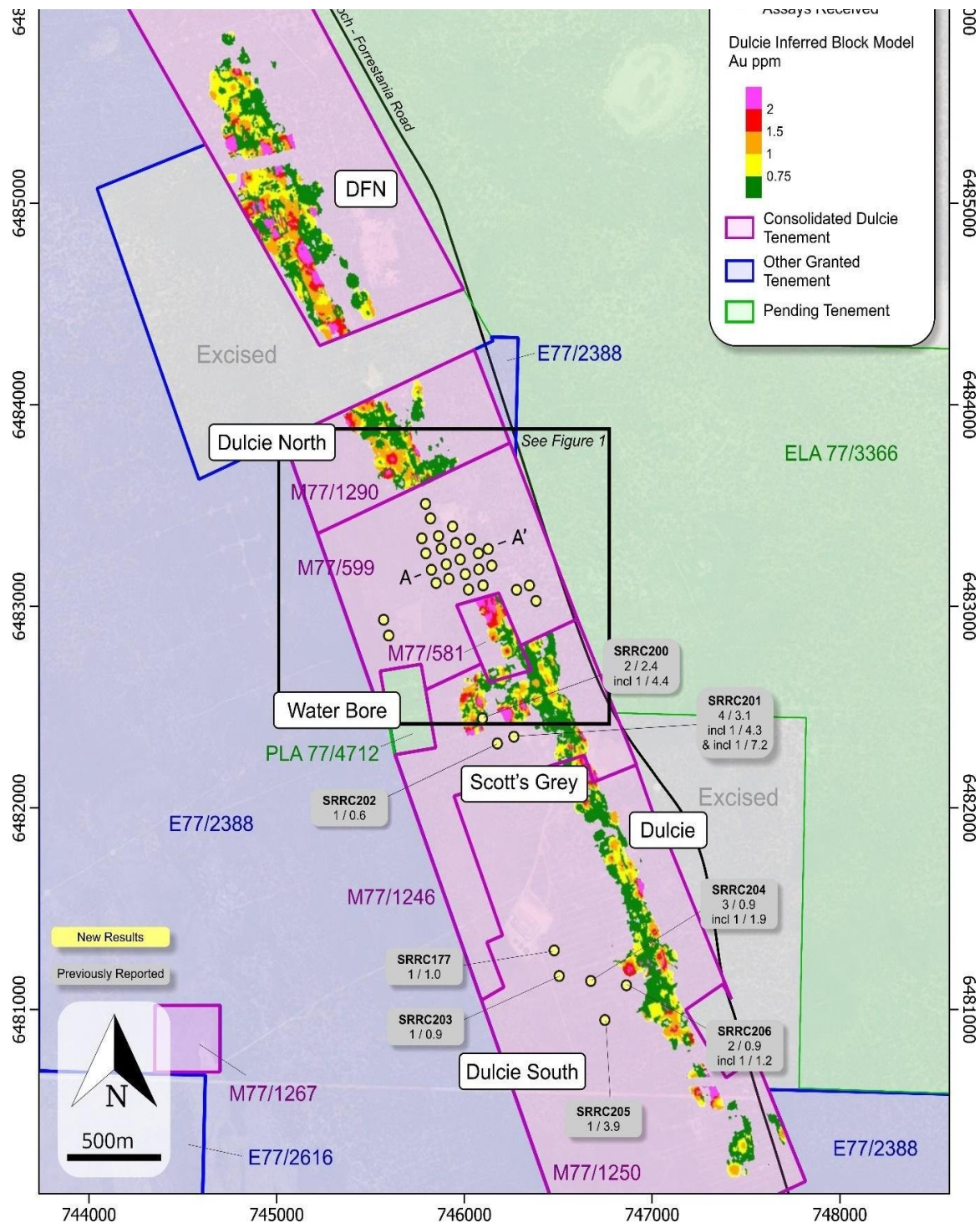
Figure 3: Consolidated Dulcie Gold Project plan showing the Inferred Mineral Resource block model (Au ppm) at Dulcie Far North (DFN), Dulcie North and Dulcie, and the RC holes completed in the 2026 programme at Dulcie Central, Water Bore, Scott's Grey and Dulcie South (refer ASX announcement 27 October 2026).
