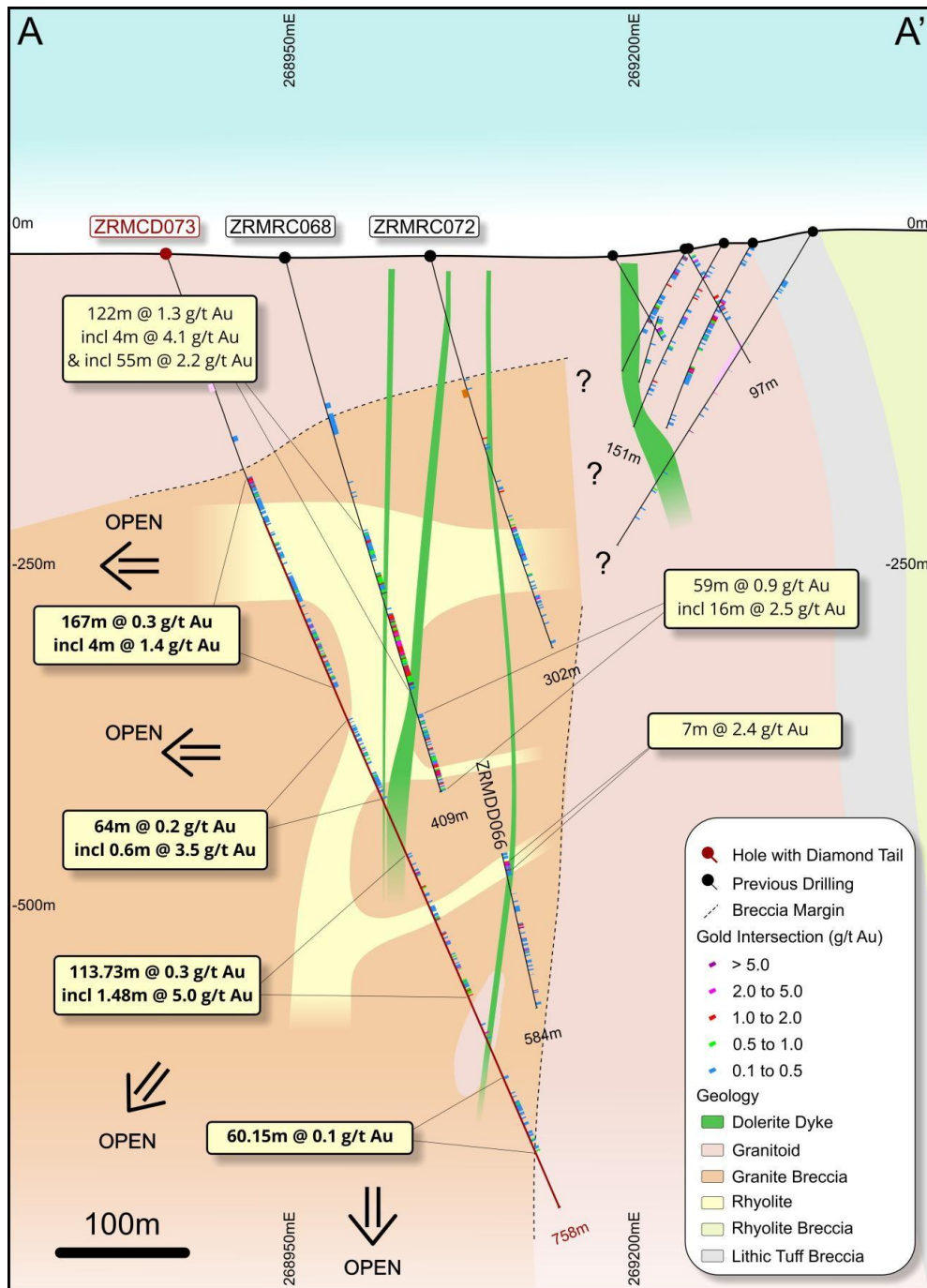
Figure 5: Cross-section A-A' through the Red Mountain breccia system showing deep diamond hole ZRMCD073 and prior drilling (refer ASX announcement 10 April 2026).
