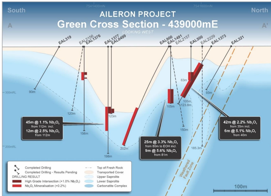
Figure 3 – Green Deposit 438700E – Cross Section A-A'
