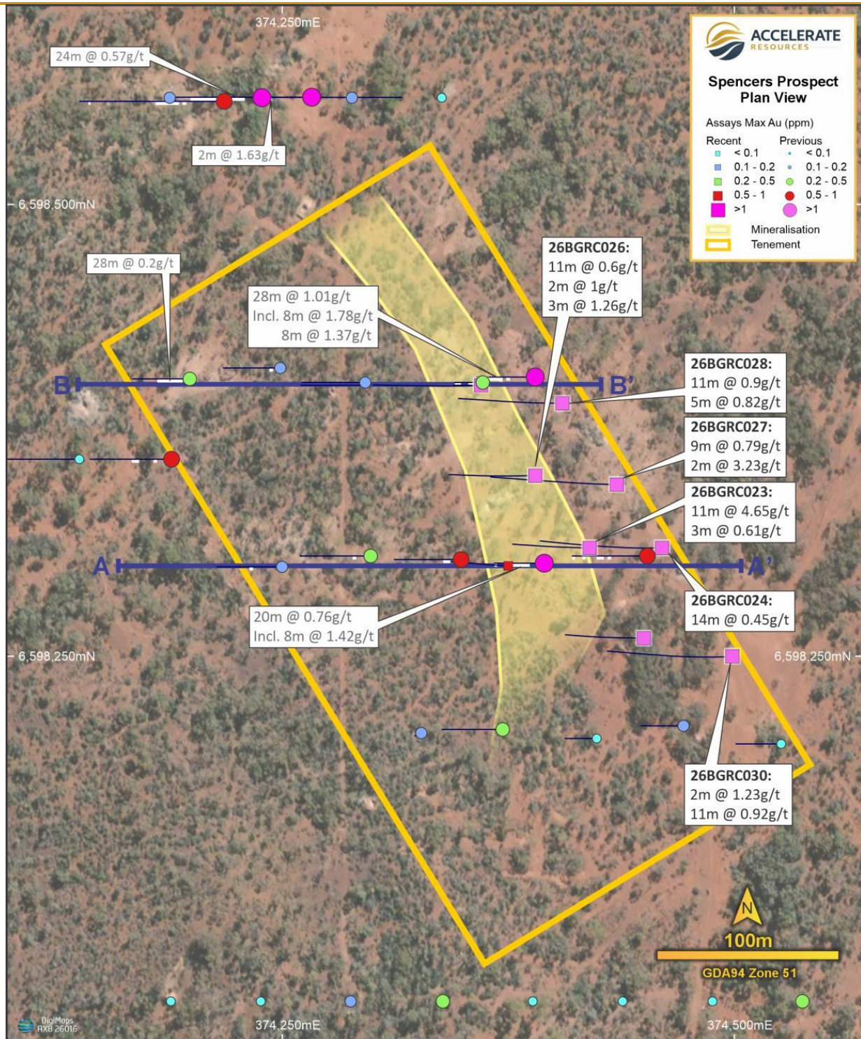
Figure 8: Spencers Prospect plan view showing RC drill results, the interpreted 300m mineralised trend and the location of cross sections. Intervals are downhole.
