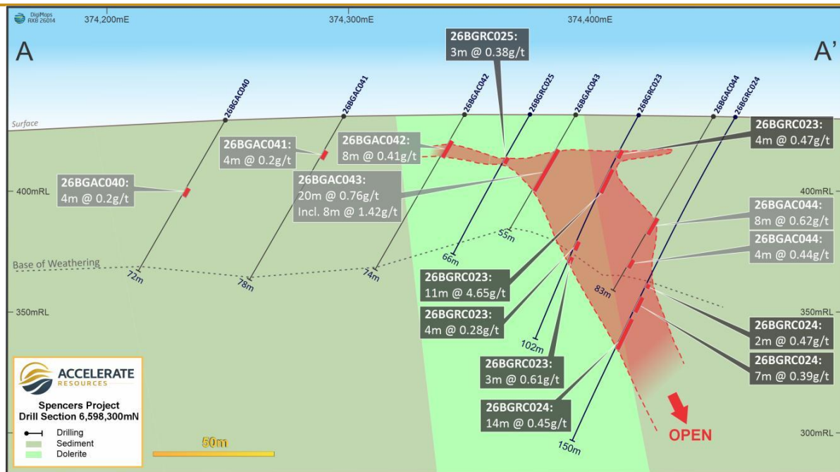
Figure 9: Spencers cross section A to A' (6,598,300mN) showing the high grade intercept in 26BGR023 and gold mineralisation remaining open at depth.
