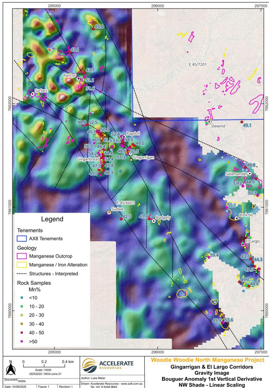
Figure 3: First vertical derivative (1VD) gravity image across Gingarrigan and El Largo showing interpreted structures and mapped manganese outcrops with Mn% assays.
