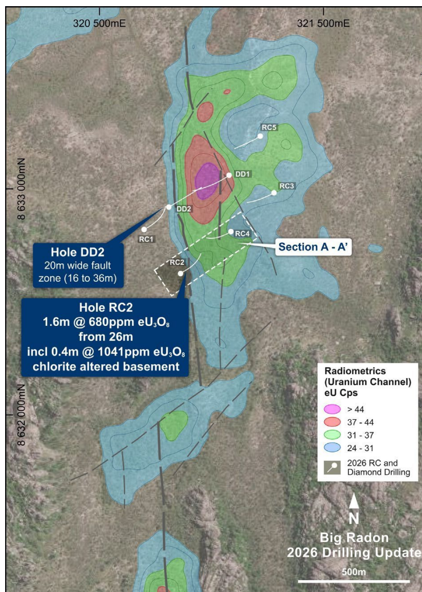
Figure 8: Big Radon Prospect – first-pass drilling intersected a north-south fault zone on the western side of the radon anomaly, with uranium mineralisation in RC2 adjacent to the fault.
