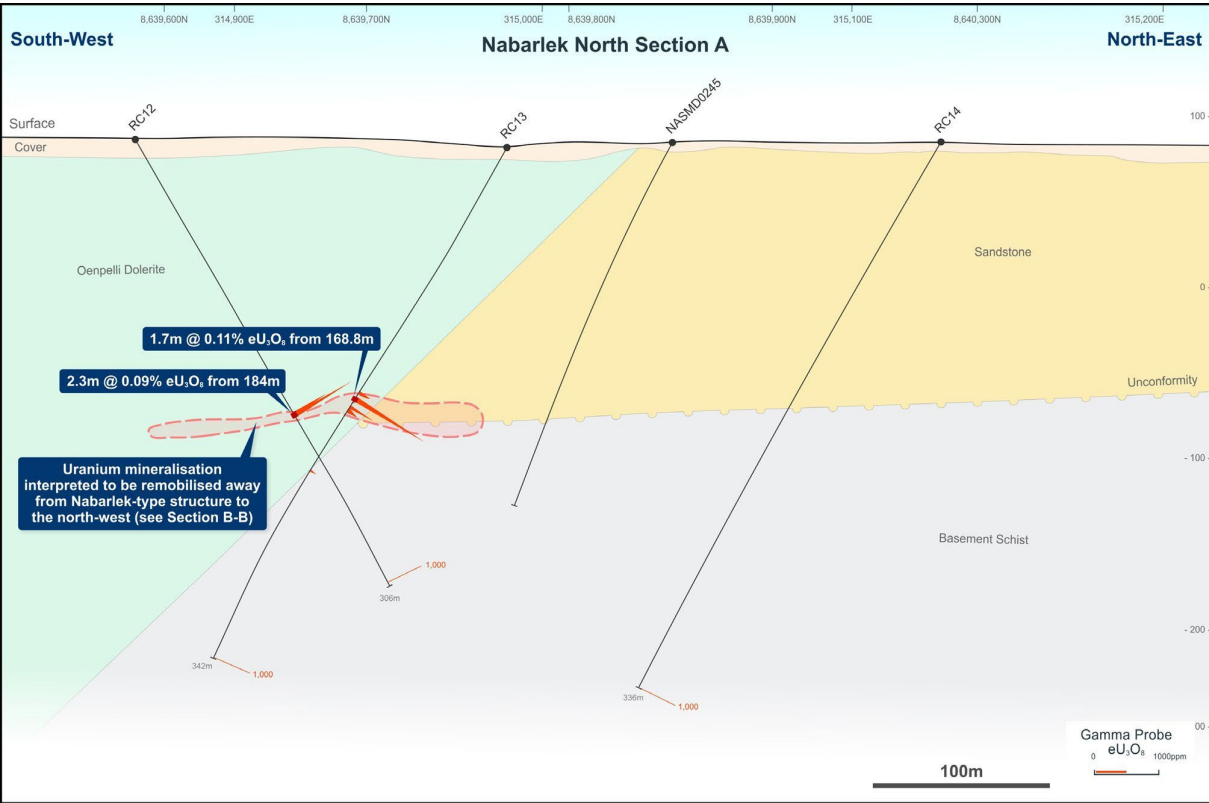
Figure 5: Nabarlek North Section A – first-pass RC drilling intersected a sub-horizontal zone of uranium mineralisation within a broad haematite zone in the footwall of the Oenpelli Dolerite.
