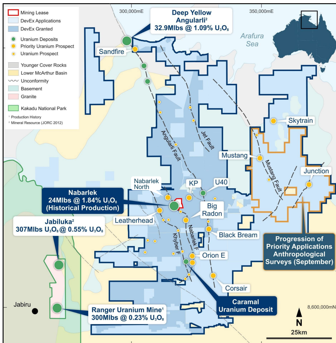
Figure 2: DevEx's Northern Territory, Nabarlek Uranium Project. (Company tenements are combined where continuous and minor excisions are removed for ease of presentation)
