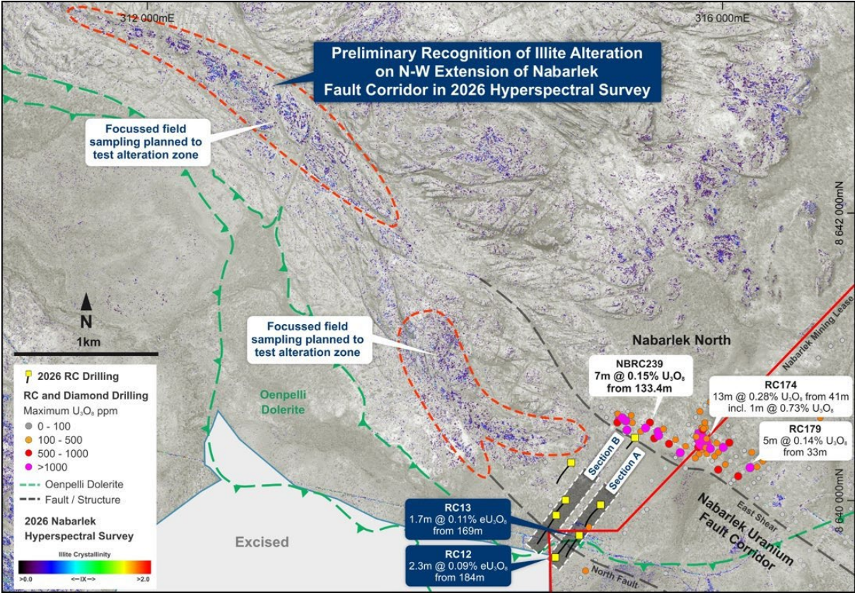
Figure 4: Nabarlek North Prospect – uranium mineralisation intersected proximal to the projected position of a fault offset in the unconformity, interpreted to be a possible position for the Nabarlek Fault. The fault zone remains open to the north-west, where the 2026 hyperspectral survey has mapped fault-controlled illite alteration over several kilometres.
