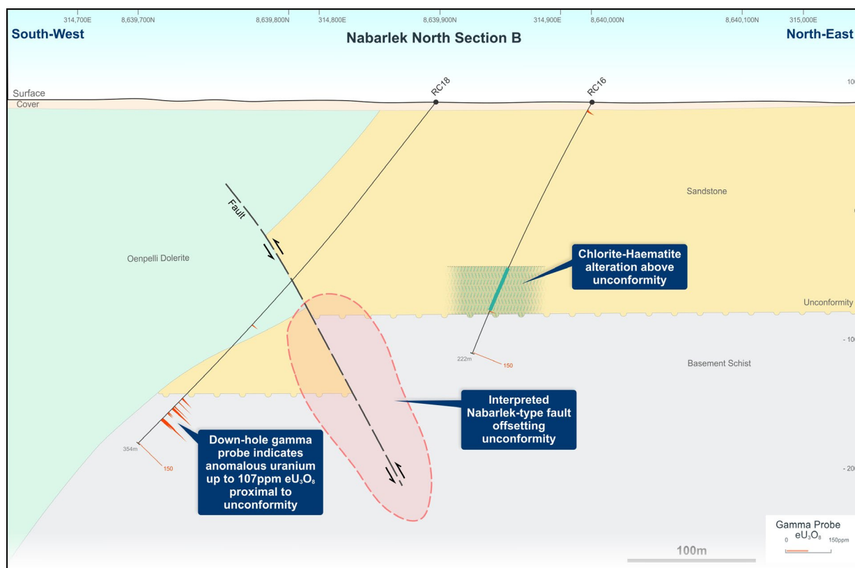
Figure 6: Nabarlek North Section B: follow-up RC drilling interprets an offset in the unconformity and dolerite between RC16 and RC18, with anomalous uranium near the unconformity in RC18 and moderate chlorite-haematite alteration above the unconformity in hole RC16 supporting a potential Nabarlek-type structure that remains untested and open to the north-west.
