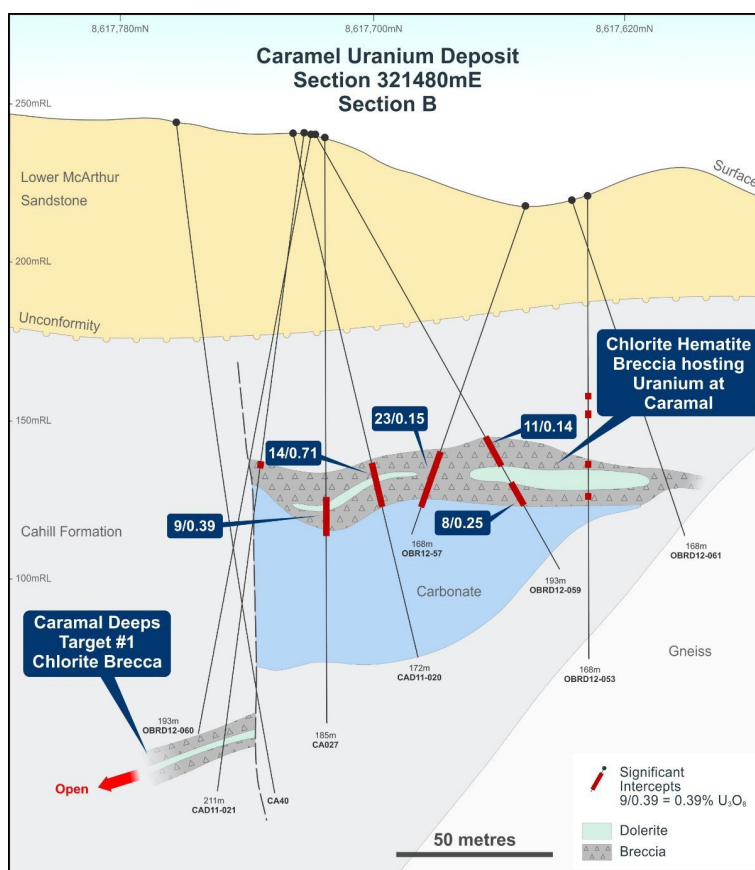
Figure 9: Caramal cross section (looking east) – relogging identified a deeper breccia and dolerite in hole CAD11-021 (Caramal Deeps Target #1) with identical geological relationships to the breccia and dolerite hosting high-grade uranium mineralisation at Caramal.
