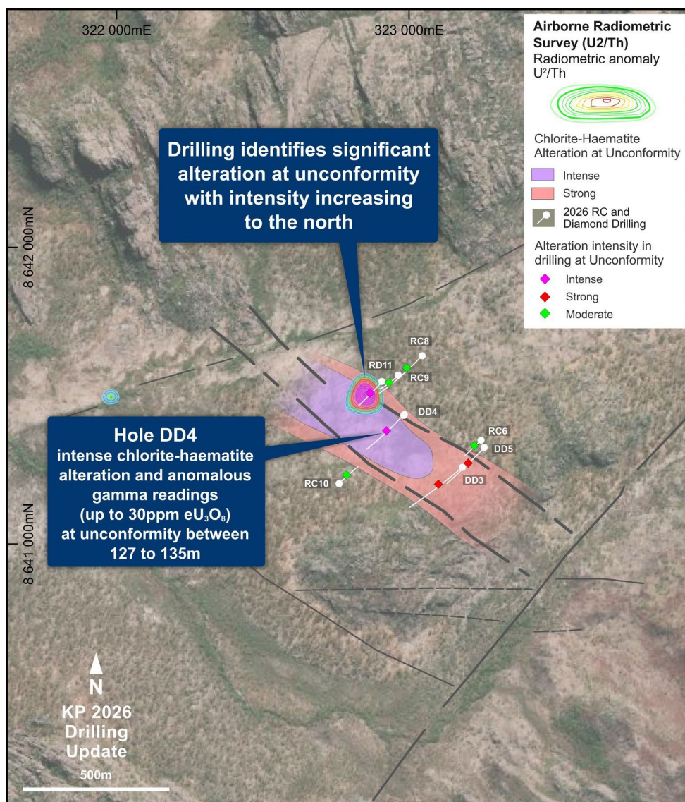
Figure 7: KP Prospect – significant chlorite-haematite alteration encountered at the unconformity in RC and diamond drilling, with alteration intensity increasing to the north.
