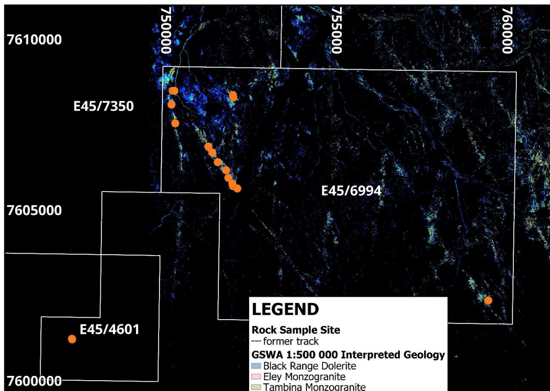
Figure 5 Sample locations on hyperspectral imagery, Eleys Project.
