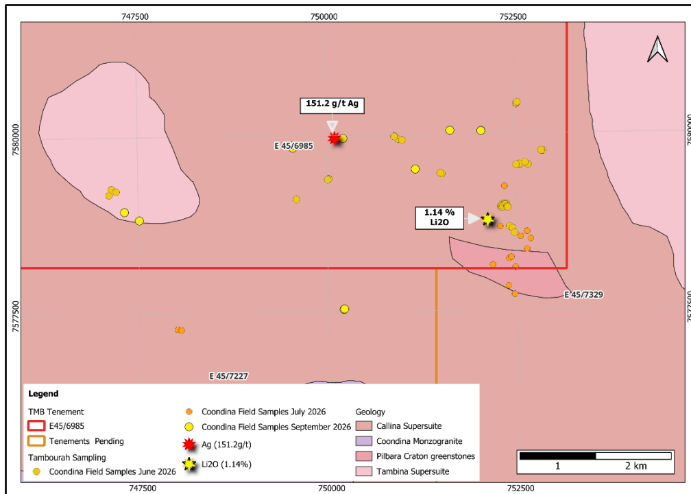
Figure 1 Coondina project sample locations on geology, showing greenstone inlier within E45/6985.
