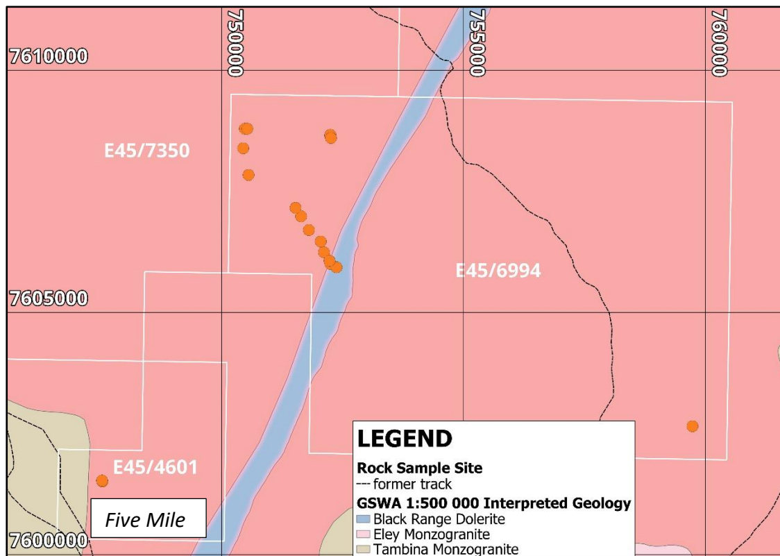
Figure 4 Sample locations, Eleys project on interpreted geology.
