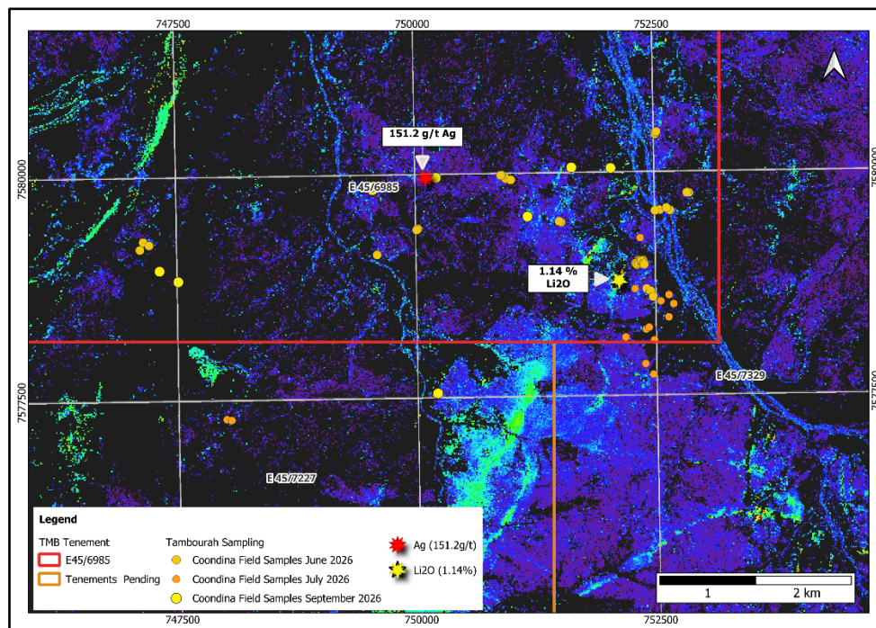
Figure 2 Sample locations on Coondina hyperspectral image.
