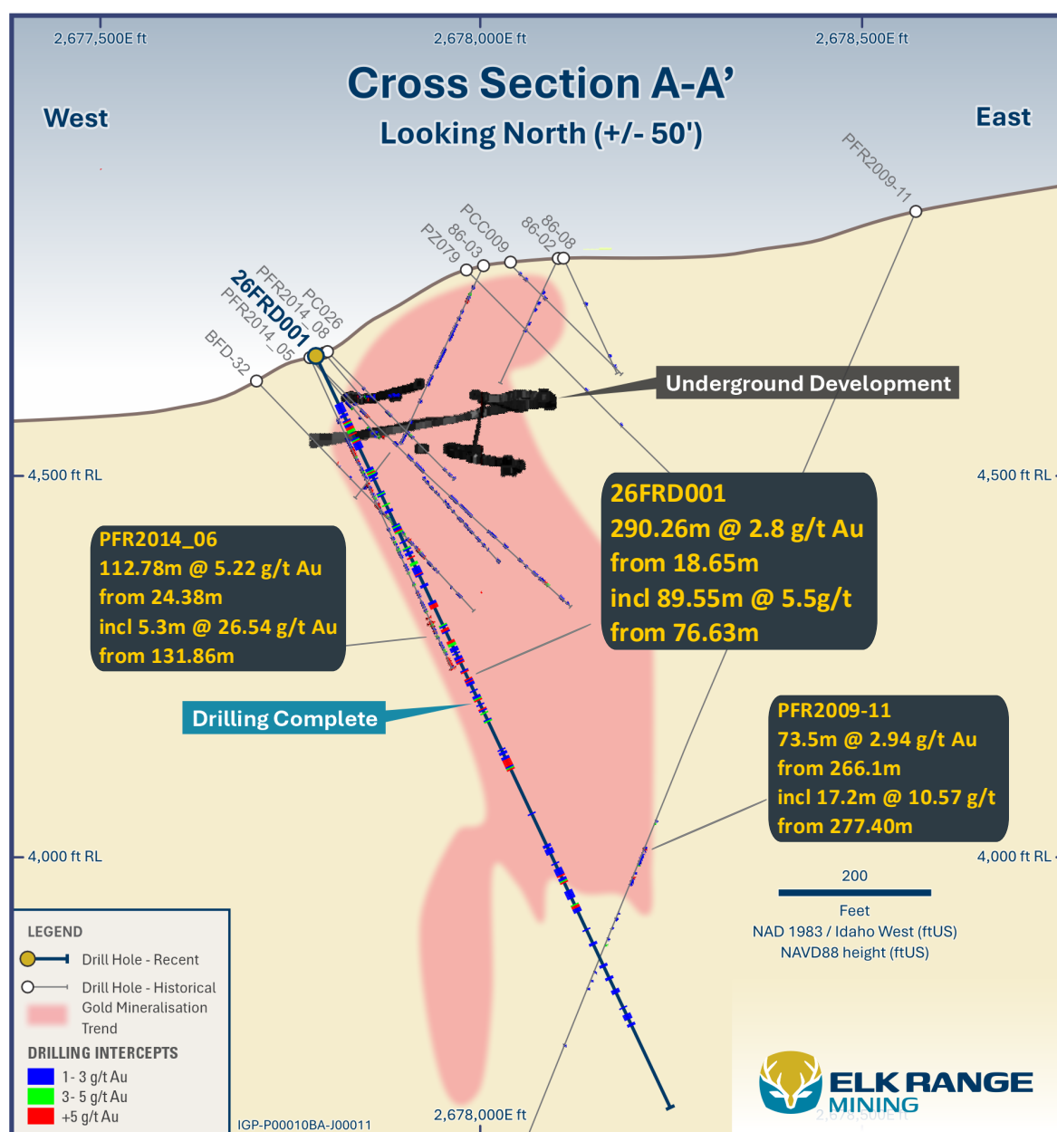
Figure 1: Cross-section A-A' (looking north) showing 26FRD001 assays and historical holes PFR2014_06 and PFR2009_11. Section displayed on the plan map (Figure 2).
