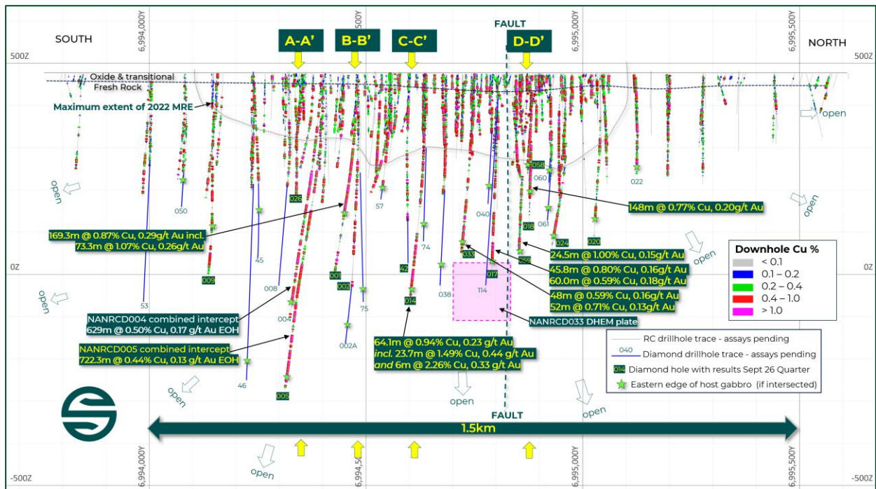
Figure 1. Nanadie long section looking west, showing all Solstice diamond drillhole numbers, holes released during the September Quarter highlighted in yellow font 2 . All prior drilling is coloured for downhole copper values 1,2 , the location of cross-sections this release and location of the NANRCD033 DHEM plate 3 relative to the maximum extent of the 2022 MRE block model 1 .
