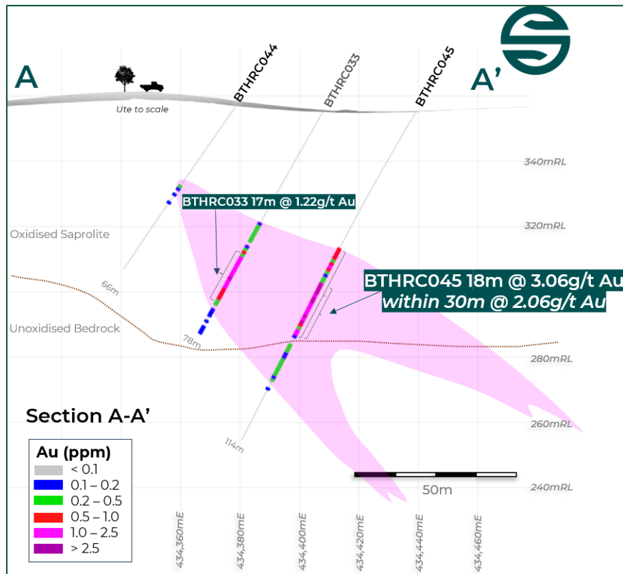
Figure 15: Bluetooth Gold Prospect cross-section A-A' (see Figure 14) showing Solstice's RC gold intercepts (white text) 5 .
