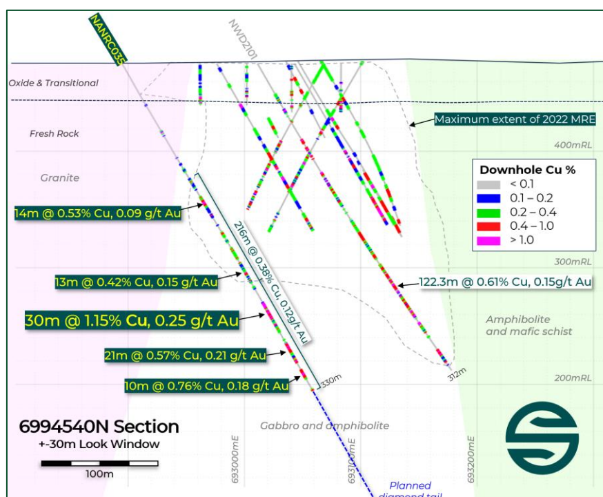
Figure 7. Nanadie Deposit cross-section 6994540N showing NANRC035 assay results 2 , simplified geology, historical drilling 1 , and the boundary of the 2022 MRE block model 1 .
