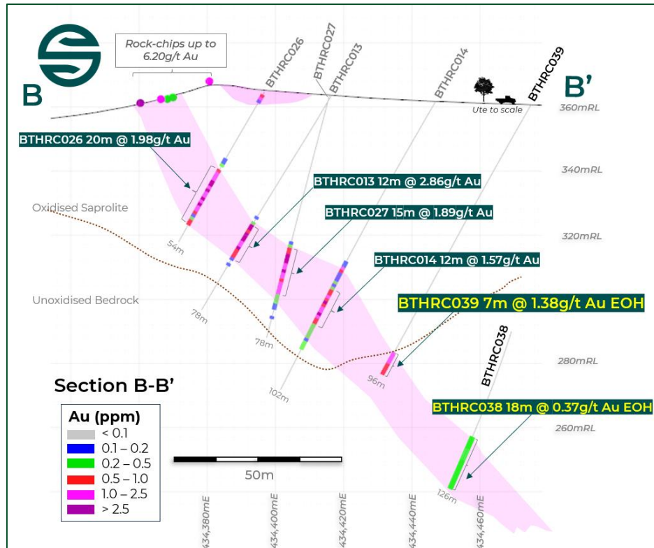
Figure 16: Bluetooth Gold Prospect cross-section B-B' (see Figure 14) showing Solstice's oxide gold intercepts (white text) and fresh rock intercepts (yellow text) 5 .
