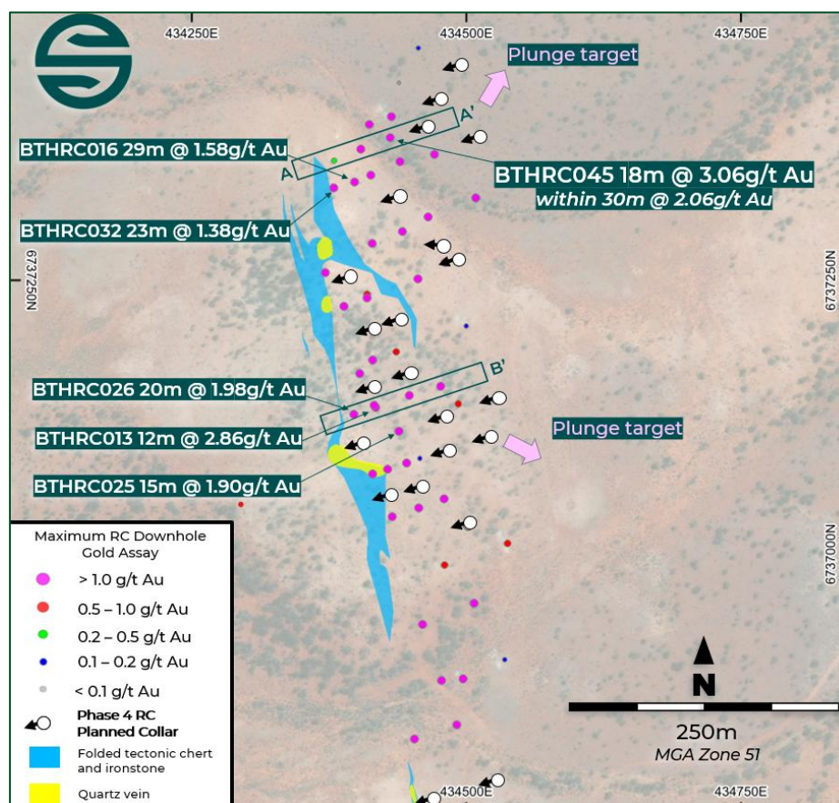
Figure 14: Bluetooth Gold Prospect showing all RC drill collars coloured for peak down-hole gold value, planned Phase 4 RC drillholes, selected gold intercepts 5 , and the outcrop of the mineralised chert and ironstone horizon.
