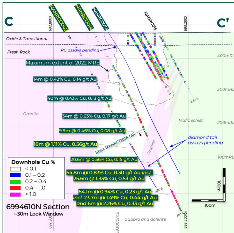
Figure 4. Nanadie Deposit cross-section 6994610N showing NANRCD014 and NANRCD042 assay results, simplified geology, Solstice's RC and diamond holes 2 , historical drilling 1 , and the boundary of the 2022 MRE block model 1 .
