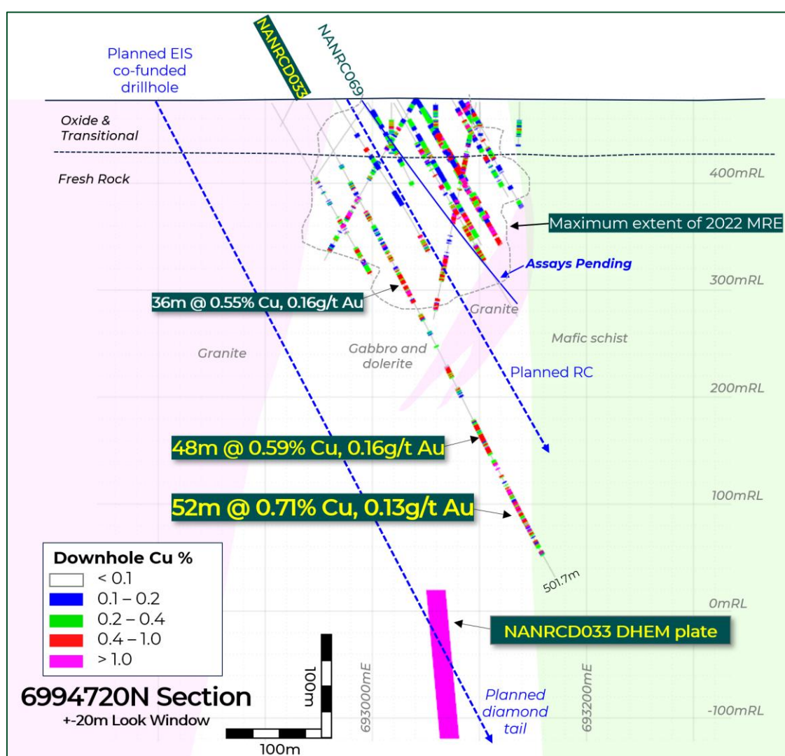
Figure 10. Nanadie Deposit cross-section 6994720N showing NANRCD033 assay results, simplified geology, and the location of the conductive plate generated by DHEM survey 3 in the hole. Also shown downhole copper values in Solstice’ earlier drilling 2 and in historical drilling 1 , and the boundary of the 2022 MRE block model 1 .
