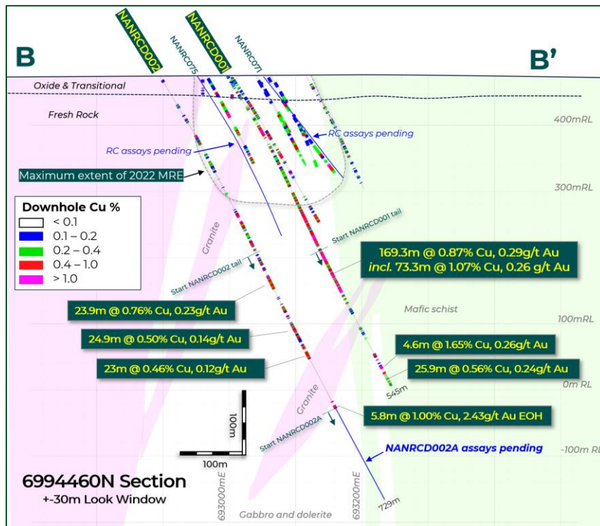
Figure 3. Nanadie Deposit cross-section 6994460N showing NANRCD001 and NANRCD002 assay results, simplified geology, Solstice's RC holes 2 , historical drilling 1 , and the boundary of the 2022 MRE block model 1 .
