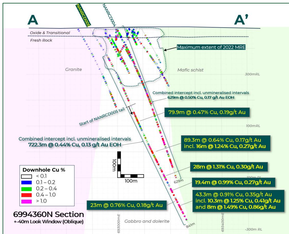
Figure 2. Nanadie Deposit cross-section 6994360N showing NANRCD005 assay results, simplified geology, and trace of earlier NANRDC004 diamond tail 2 . Also showing Solstice's RC holes 2 and historical drilling 1 , and the boundary of the 2022 MRE block model 1 .
