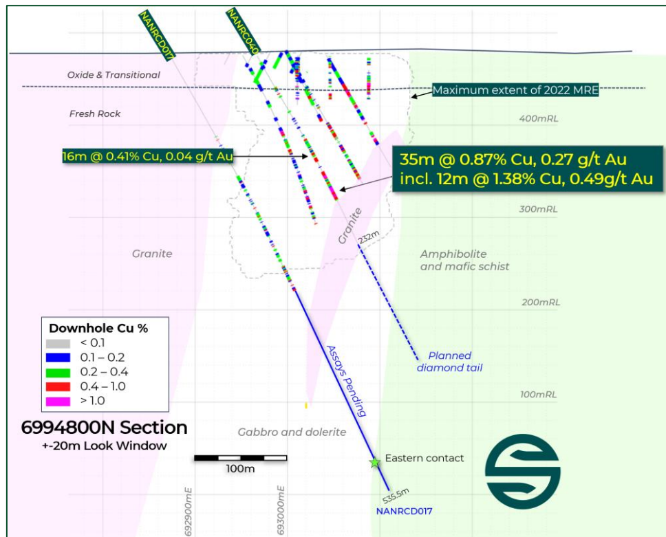
Figure 8. Nanadie Deposit cross-section 6994800N showing NANRC040 assay results, simplified geology, Solstice's RC and diamond holes 2 , historical drilling 1 , and the boundary of the 2022 MRE block model 1 .
