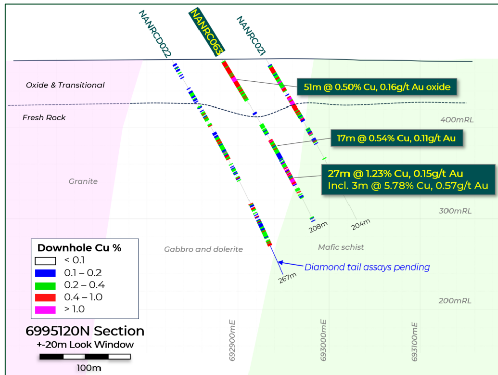
Figure 9. Nanadie Deposit cross-section 6995120N showing NANRC063 assay results, simplified geology, and prior Solstice RC holes 2 .
