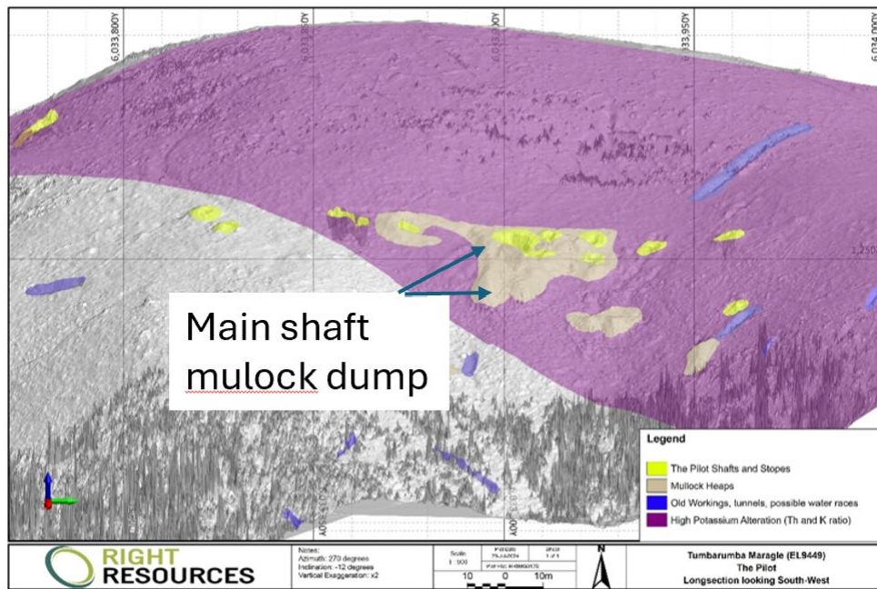
Figure 4: LiDAR image showing the relationship of the Pilot main shaft mullock dump to shafts and workings.
