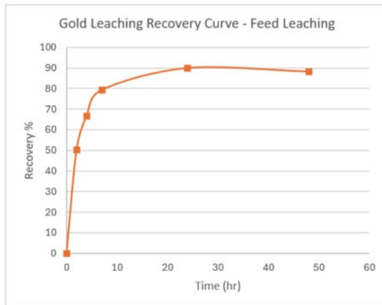
Figure 5: Whole-ore cyanide leaching extraction curve showing 89.9% gold extraction after 24 hours and 88.1% after 48 hours.
