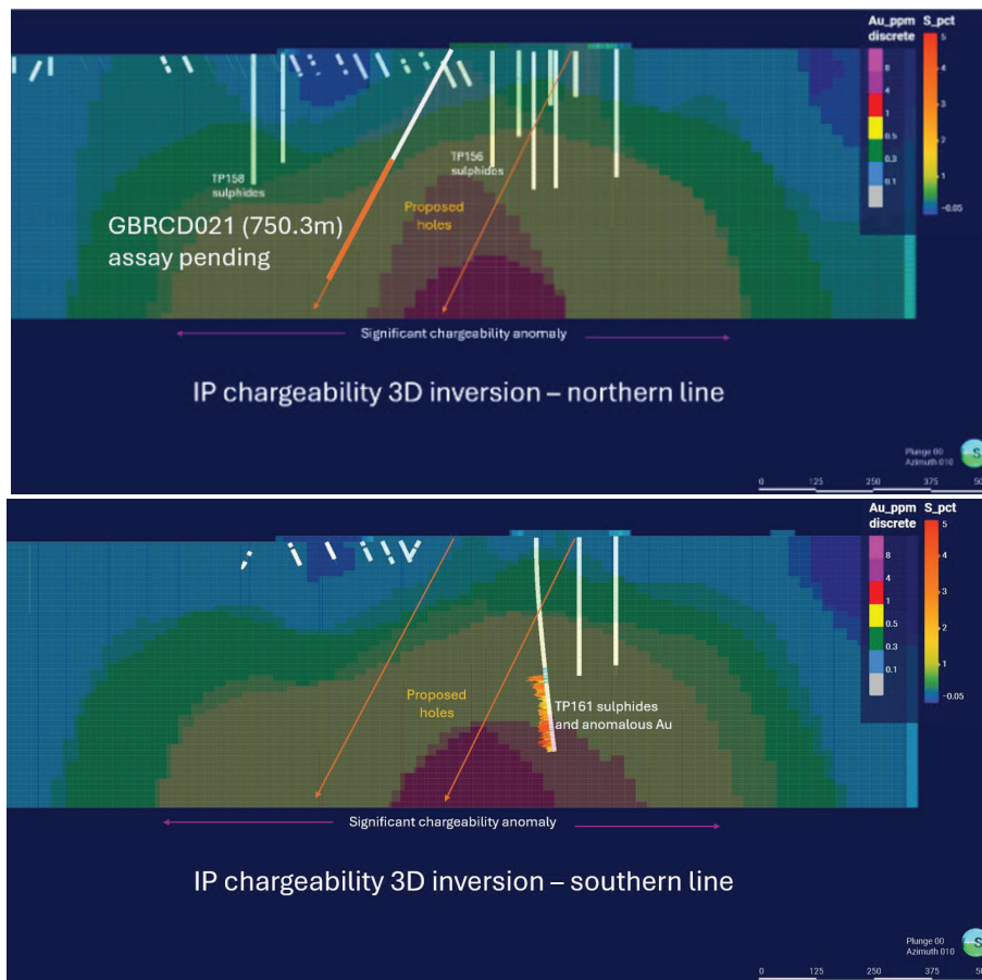
Figure 5: Cross section of the modelled IP data along IP line 1 (top) showing location of GBRCD021 (assay pending) and IP line 2 (bottom) with proposed holes.
