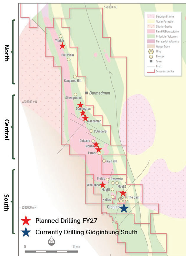
Figure 1: Location of current and developing drill targets across the Gilmore Project.
