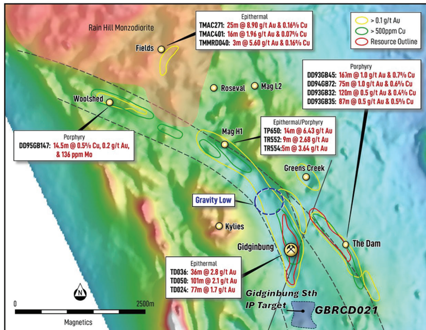
Figure 3: Reduced to pole (RTP) magnetic map of the Southern Zone including Gidginbung South target zone.
