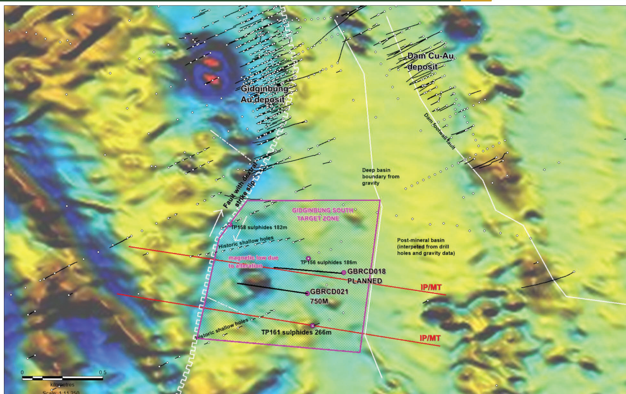
Figure 4: First vertical derivative reduced to the pole magnetics (Southern Zone) with drill hole locations of GBRCD021 and GBRCD018 (planned).
