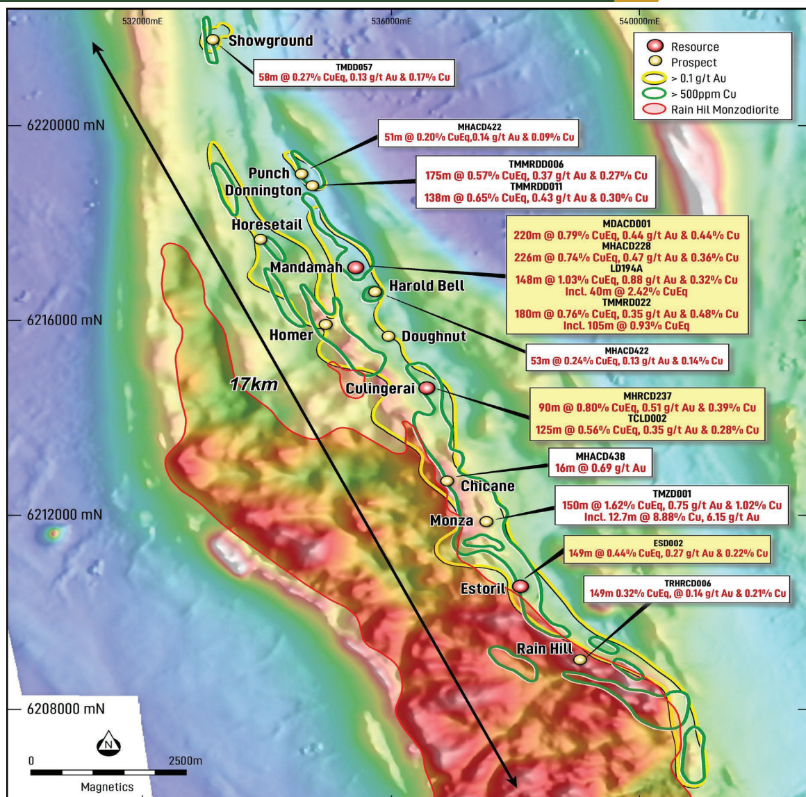
Figure 6: Plan view of the Central Zone highlighting the 17km strike and selected drill hole intercepts.
