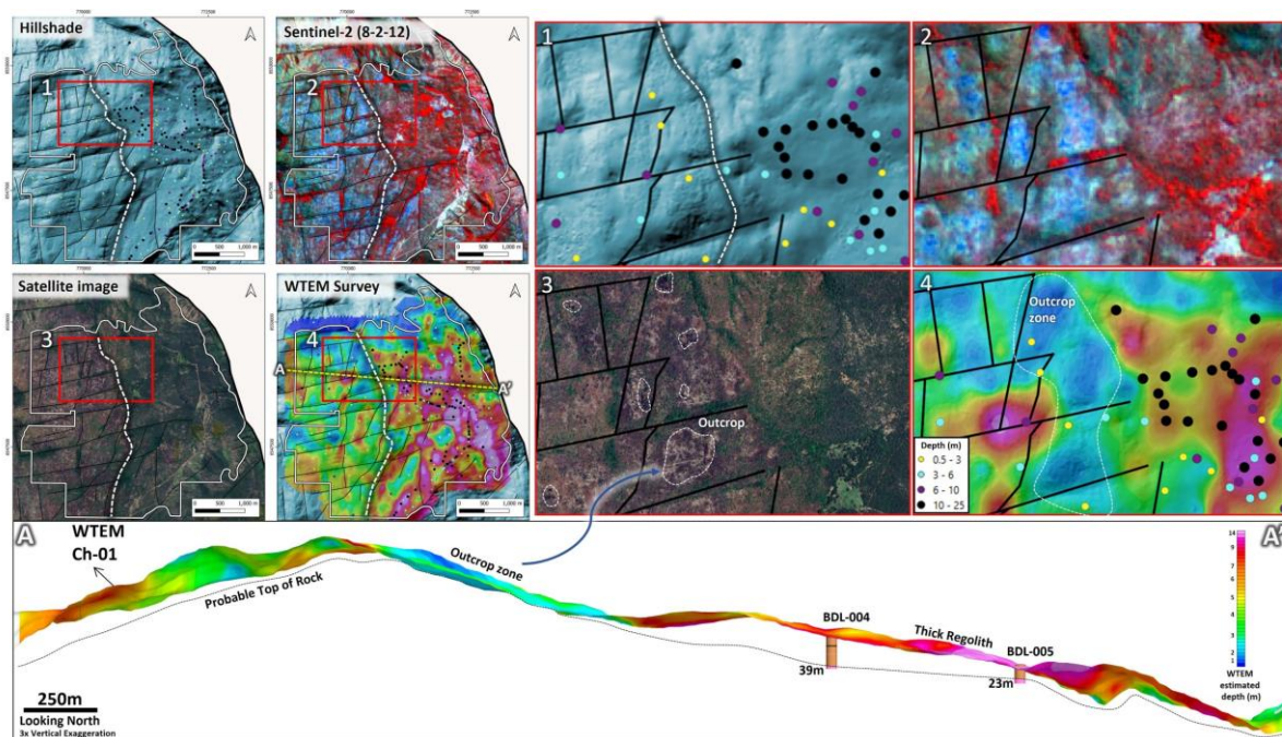
Figure 1: Boa Vista prospect. Upper panels: (1) terrain hillshade, (2) Sentinel 2 satellite composite, (3) satellite image and (4) EM survey response, with auger holes coloured by depth. The red box marks the detail area shown at right. Lower panel: section A to A' looking north (3x vertical exaggeration) with diamond holes BDL004 and BDL005.
