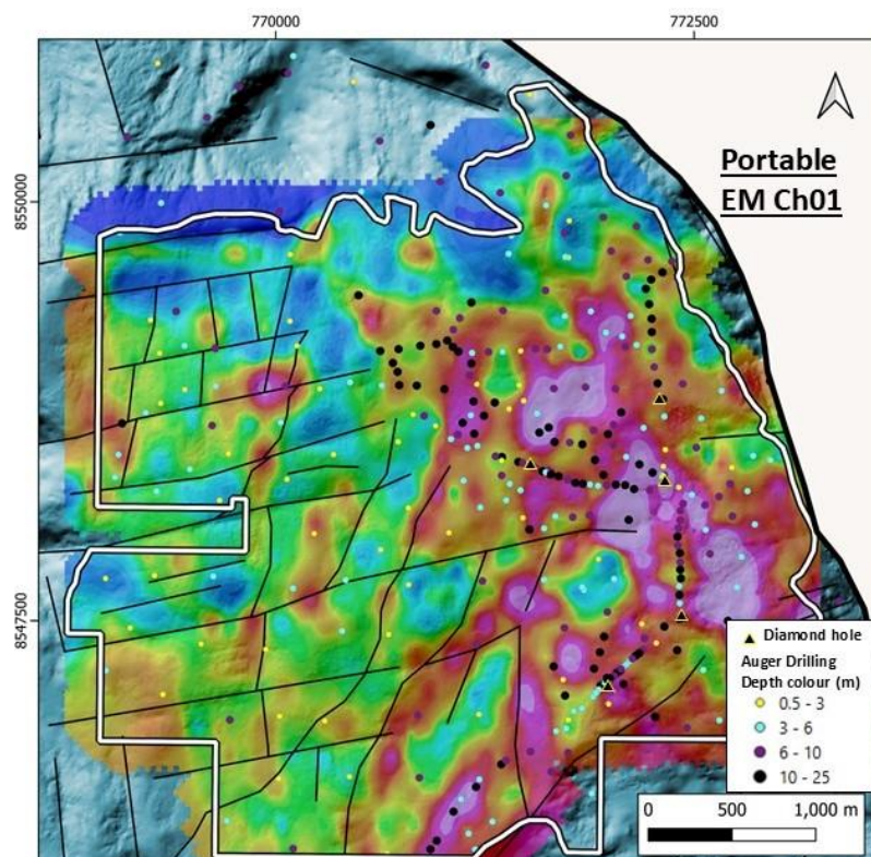
Figure 2: Boa Vista EM survey response (CH01) with holes labelled and coloured by depth (m). Stronger responses (red to pink) coincide with deeper drill holes.
