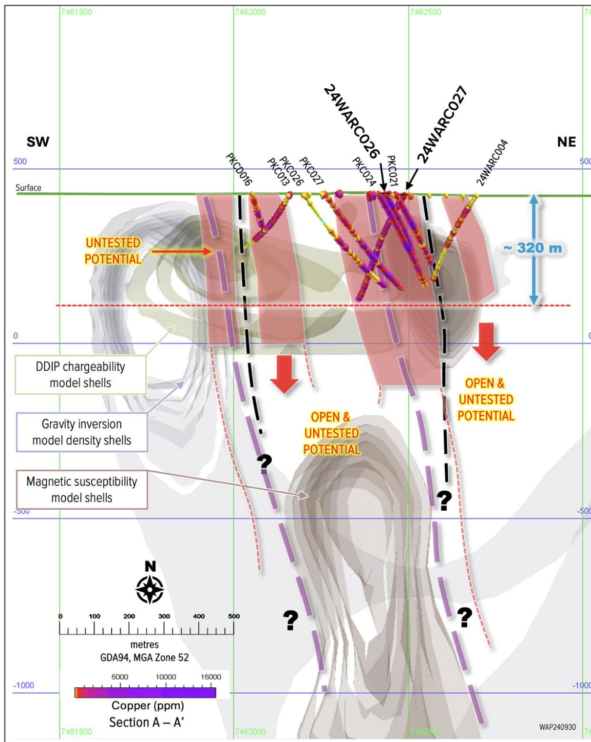
Figure 5 – Schematic section A-A' through Pokali East showing infill/validation drillholes 24WARC026 and 24WARC027 twinning historical holes PKC024 and PKC021, and confirming sub-vertically oriented, high-grade (>1.0% Cu) copper lodes open at depth (source: Rincon Resources Limited, ASX announcement dated 2 October 2024).
