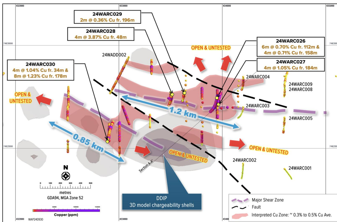
Figure 4 – Enlarged schematic plan of the Pokali East infill/validation drilling program, showing significant intercepts and open, untested strike extensions (source: Rincon Resources Limited, ASX announcement dated 2 October 2024).
