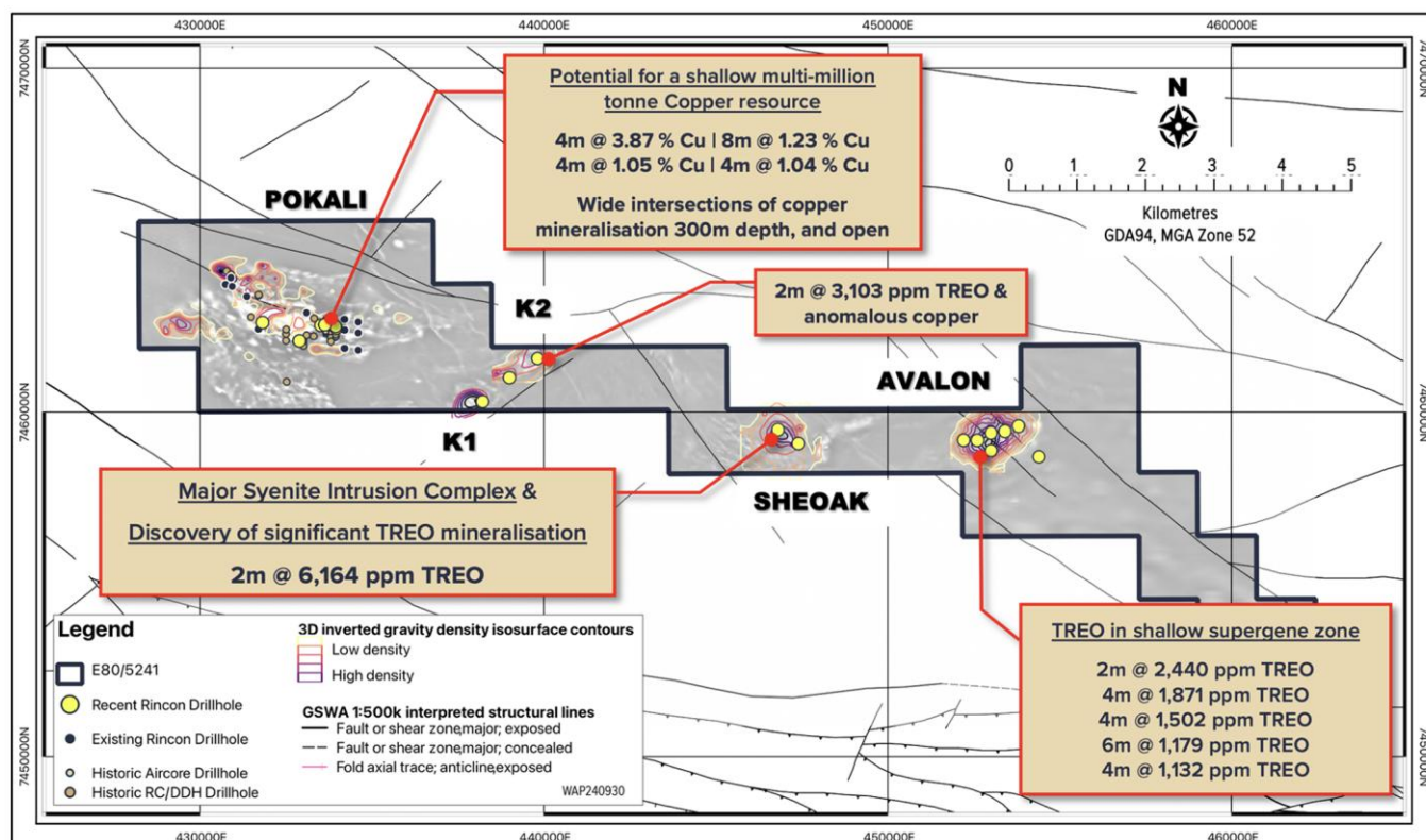
Figure 3 – West Arunta Project tenement E80/5241 showing drilling locations and selected significant historical intercepts at Pokali and surrounding targets (source: Rincon Resources Limited, ASX announcement dated 2 October 2024). (Note: the tenement area has changed since the Rincon Resources Limited 2 October 2024 announcement)
