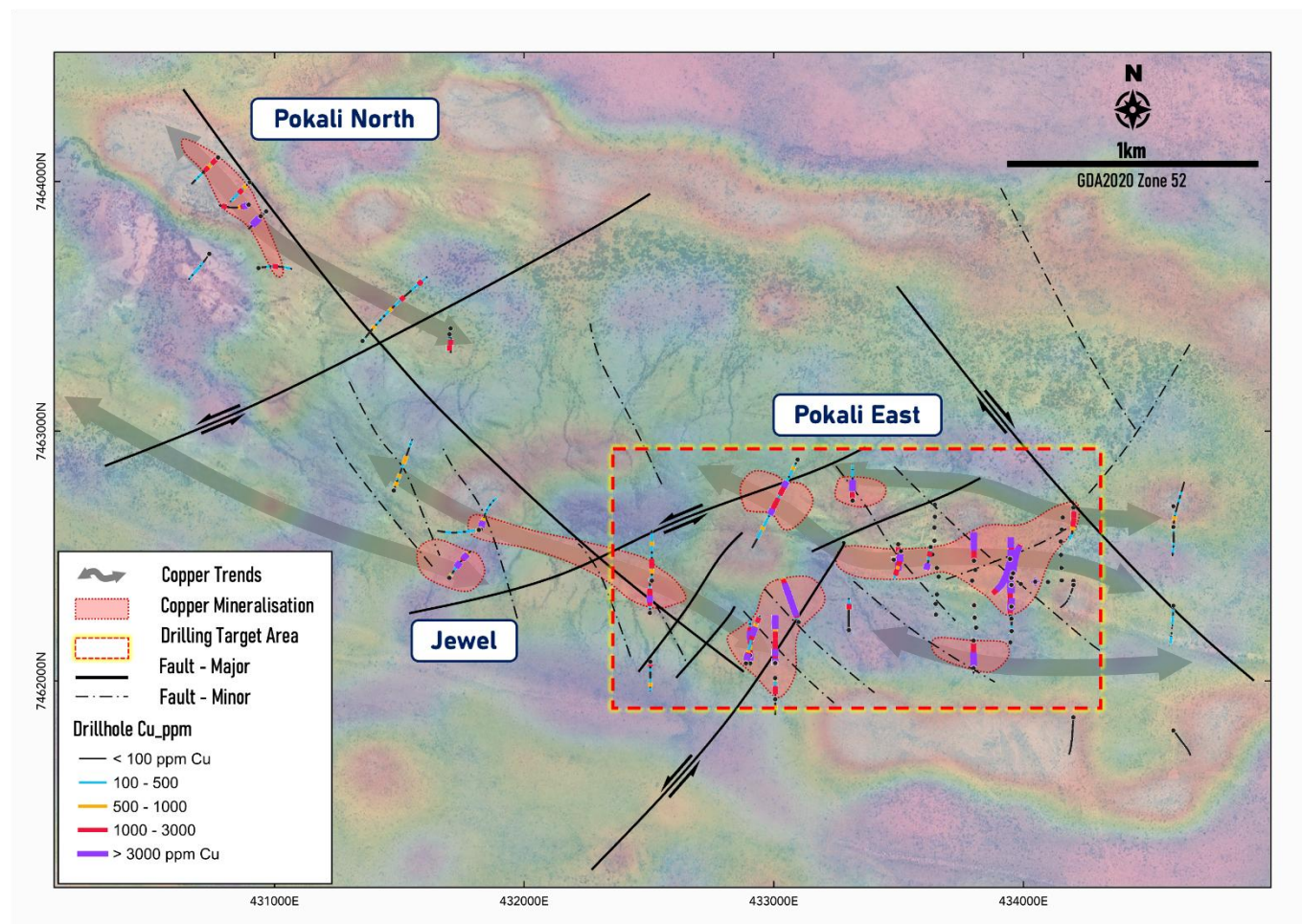
Figure 2 – Pokali East gravity/magnetic inversion image showing the priority copper anomaly targeted by Maverick's RC/Aircore drilling program (Company interpretation).
