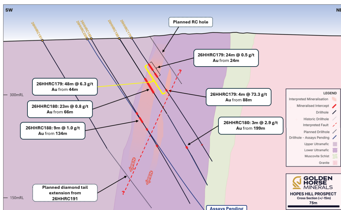
Figure 7: Cross Section looking Northwest of hole 26HHRC179 (4m @ 73.3 g/t Au from 88m).
