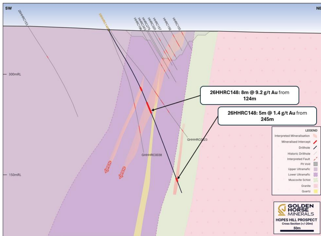
Figure 8: Cross section of hole 26HHRC148 (8m @ 9.2 g/t Au from 124m, including 4m @ 17.4 g/t Au from 128m) with footwall mineralisation of 5m @ 1.4 g/t Au from 245m also shown.
