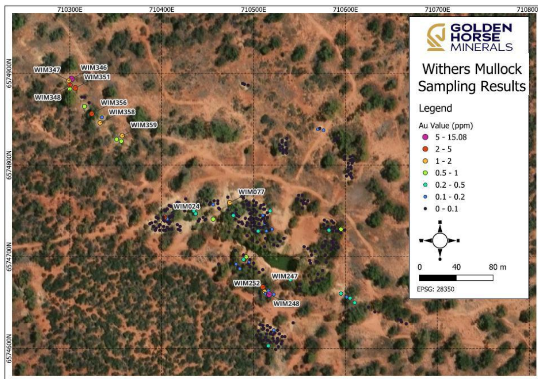
Figure 13: Plan view of Withers 2026 grab sampling program showing Au grades by colour.
