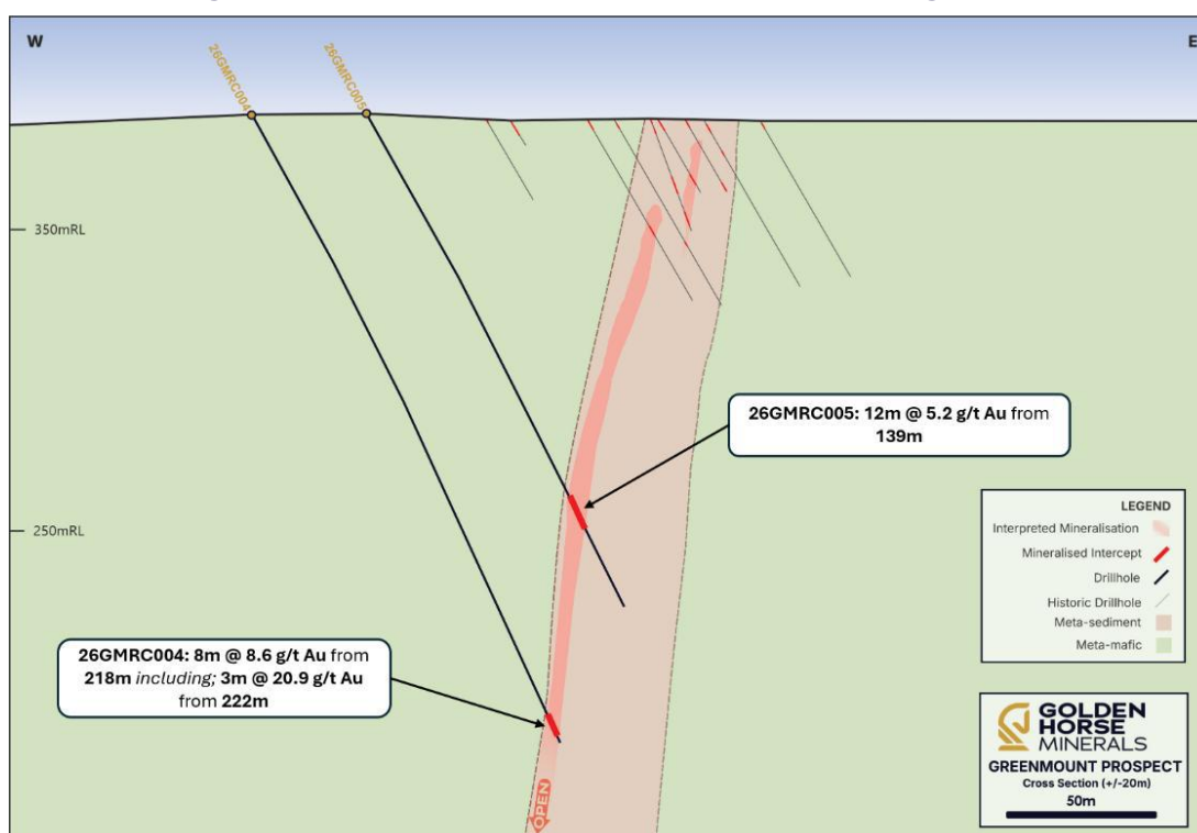
Figure 11: Cross section looking North denoting high-grade intersection within hole 26GMRC005: (12m @ 5.2 g/t Au from 139m) and hole 26GMRC004 (8m @ 8.6 g/t Au from 218m).
