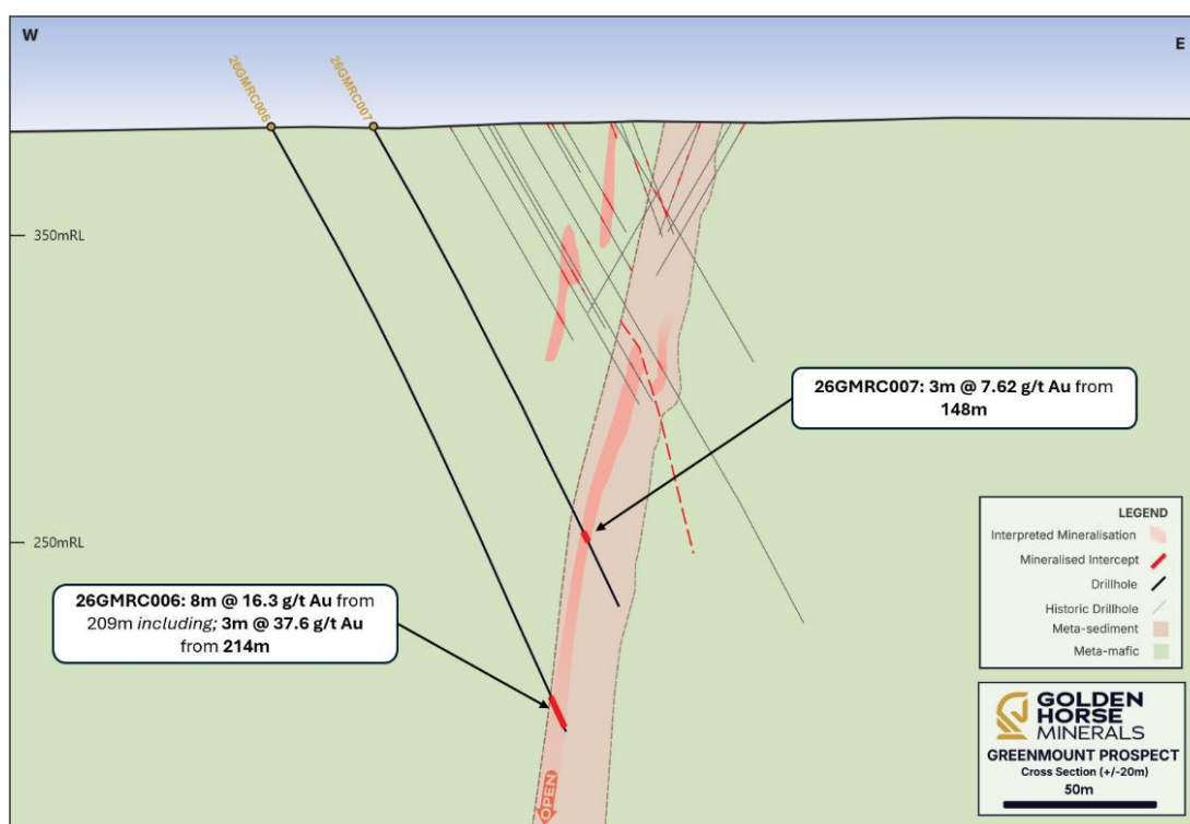
Figure 10: Cross section looking North denoting high-grade intersection within hole 26GMRC006: 8m @ 16.3 g/t Au from 209m and hole 26GMRC007: 3m @ 7.62 g/t Au from 148m.
