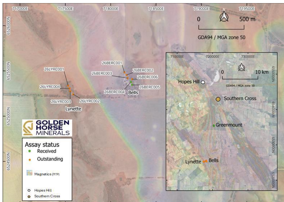
Figure 14: Plan view map of the Bells & Lynette prospects.
