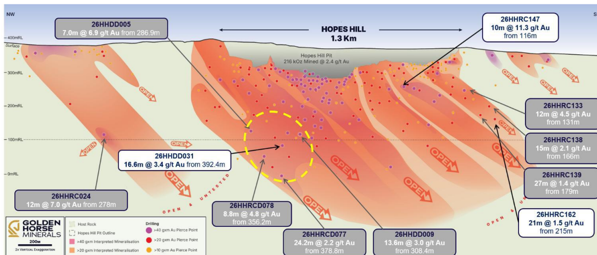
Figure 3: Hopes Hill long section (looking East) showing holes reported for the quarter 3 .
