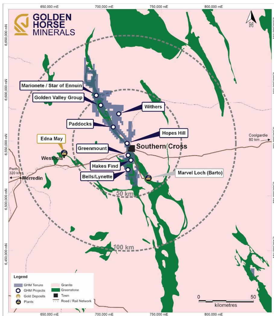
Figure 9: Regional map outlining regional prospects over Golden Horse tenure.
