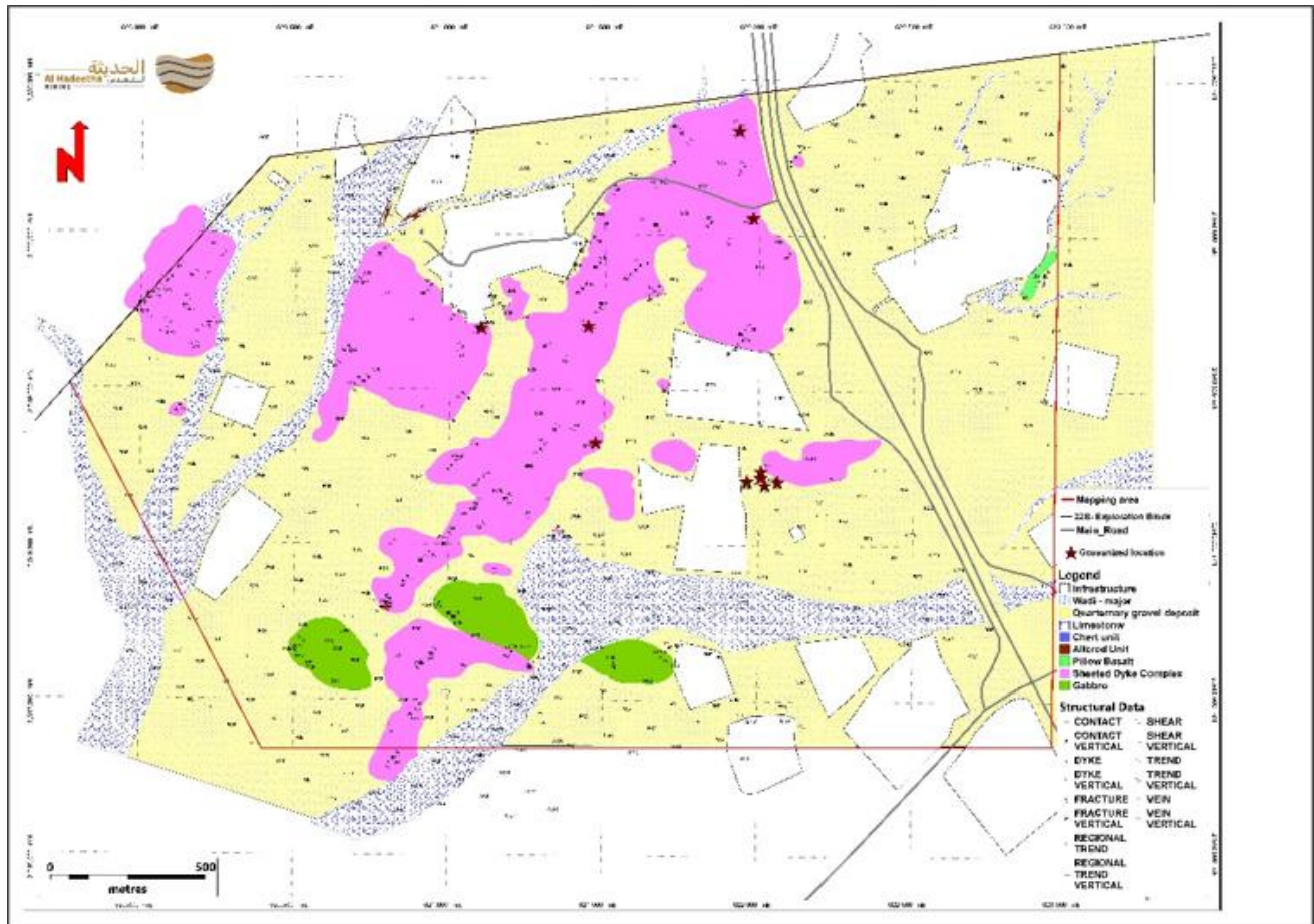
Figure 31 – Geological map of Prospect 22B-T08
