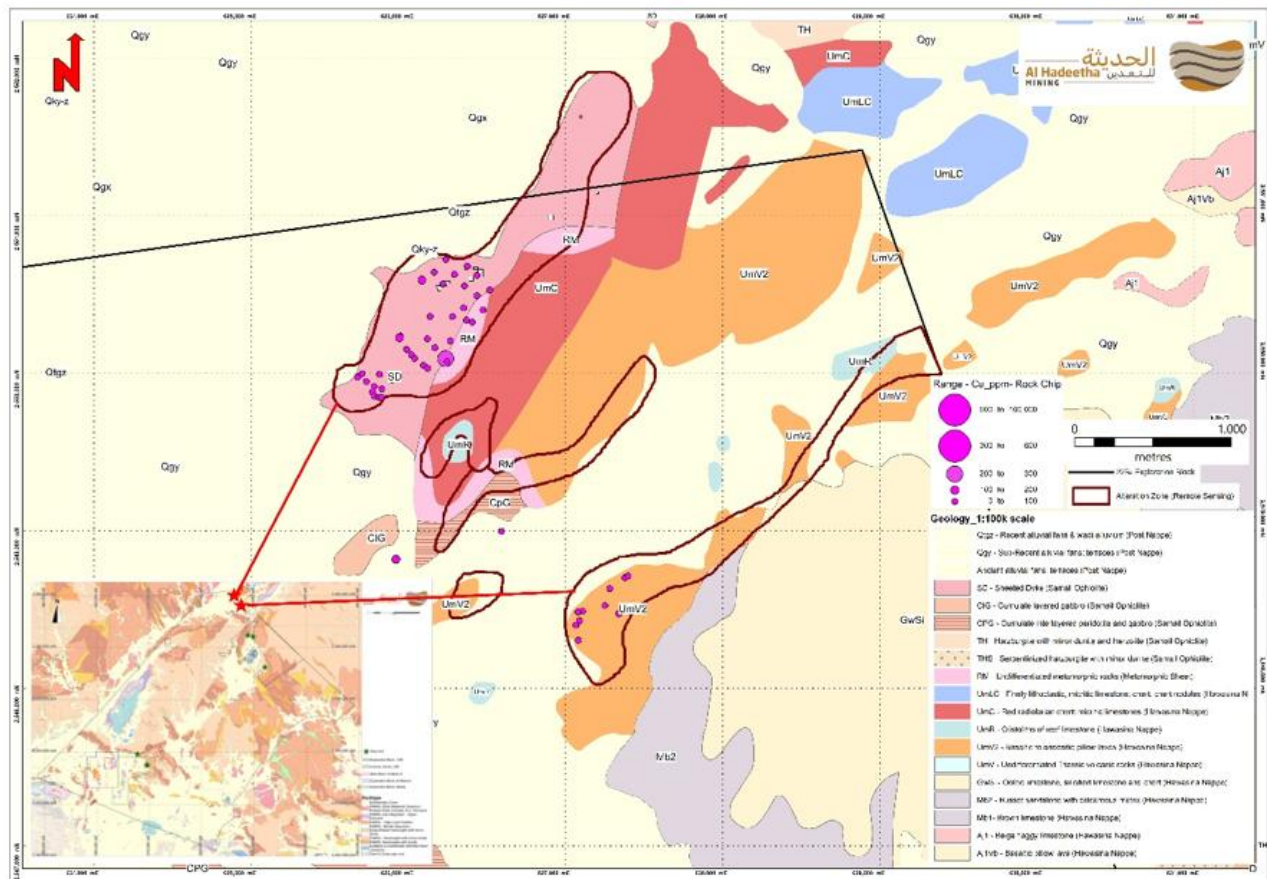
Figure 28 – Geological traversing and ground truthing north-western sector of the concession
