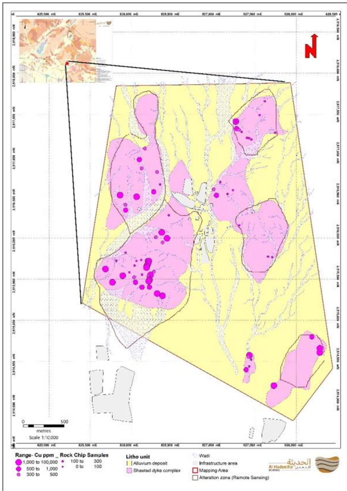
Figure 29 – Geological mapping of Prospect 22B-T10
