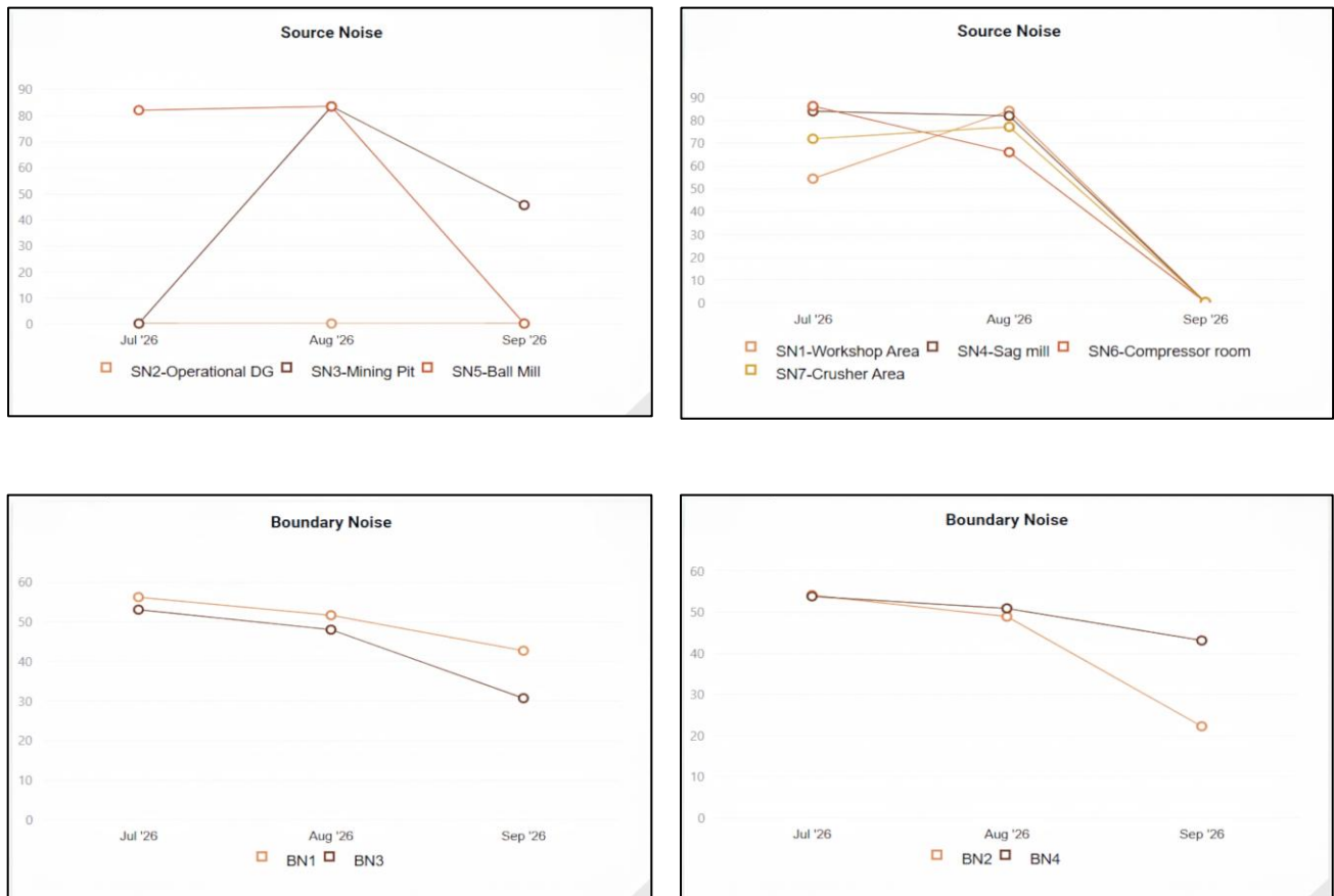
Figure 21 – Boundary Noise Monitoring
