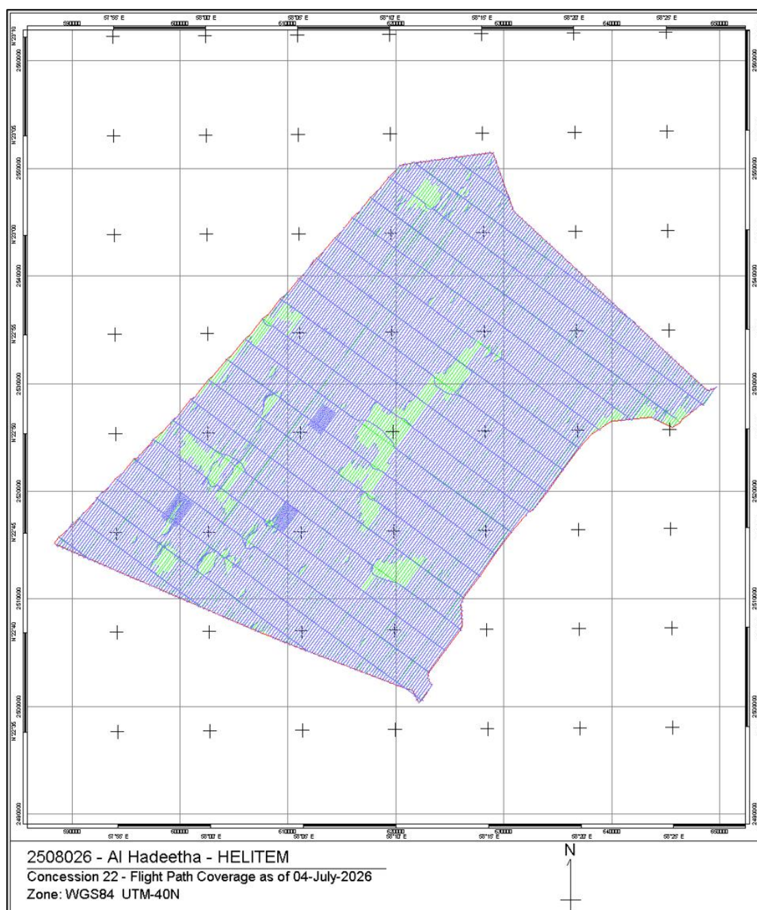
Figure 34 – Block 22B Flight Path Coverage for HelITEM survey
