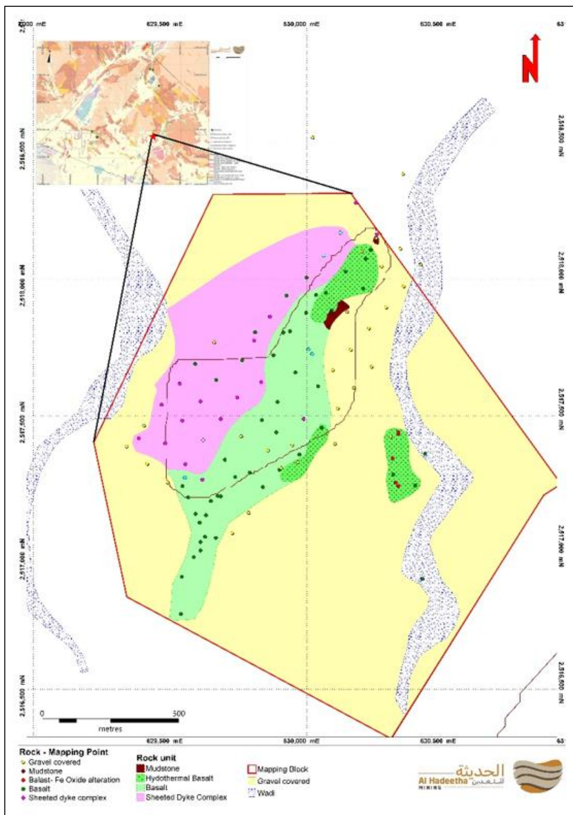
Figure 32 – Geological map of Prospect 22B-T11
