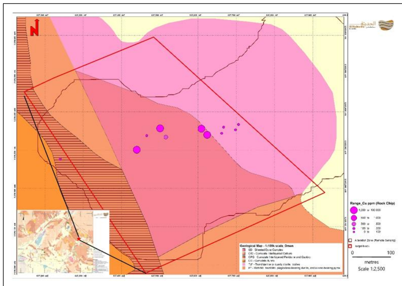
Geological Mapping – 22B-T08
