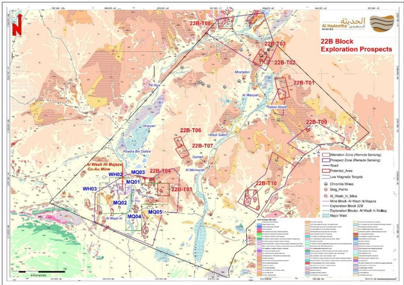
Figure 27 – Block 22B identified Prospects based on geological mapping, field observations & remote sensing study
