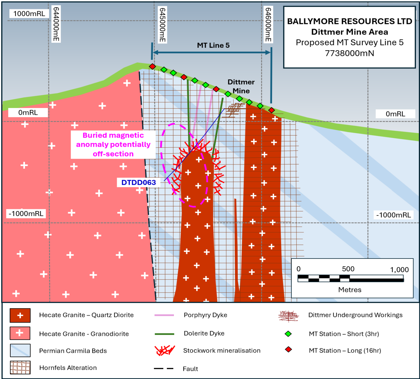
Figure 3 - Dittmer interpreted cross section 7738000mN with MT survey stations and conceptual target.
