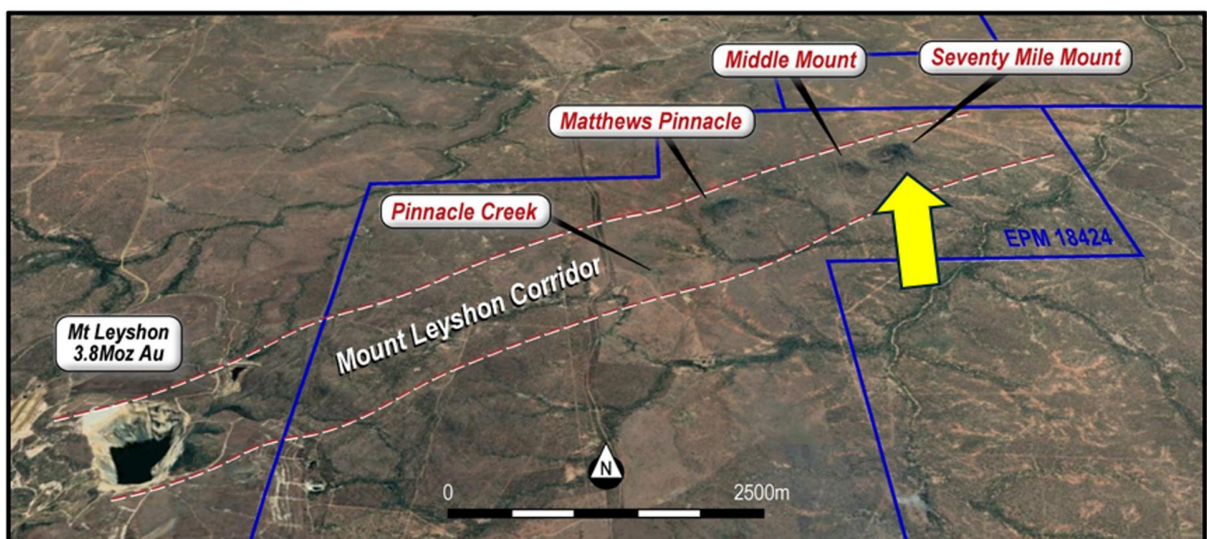
Figure 7 – Airphoto showing the Mount Leyshon mine and the Seventy Mile Mount breccia pipe, sitting within the Mount Leyshon Corridor.
