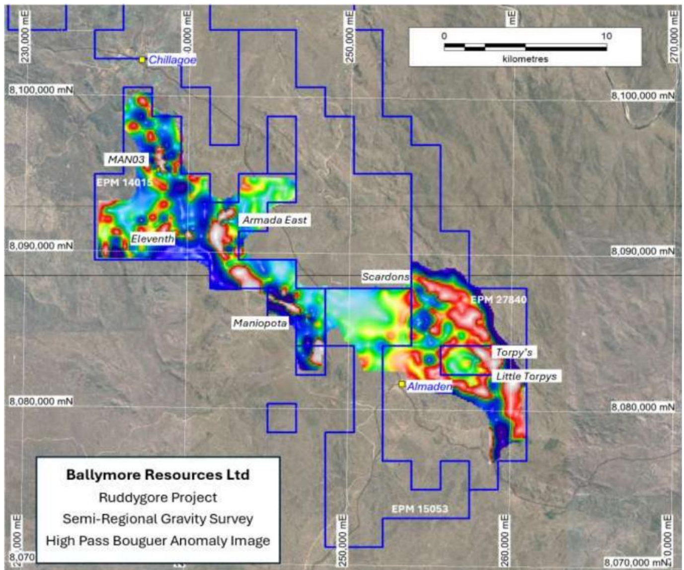
Figure 6 – Ruddygore gravity high pass filter Bouguer anomaly image based on preliminary gridded data (released 29 June 2026). Final data is being modelled.
