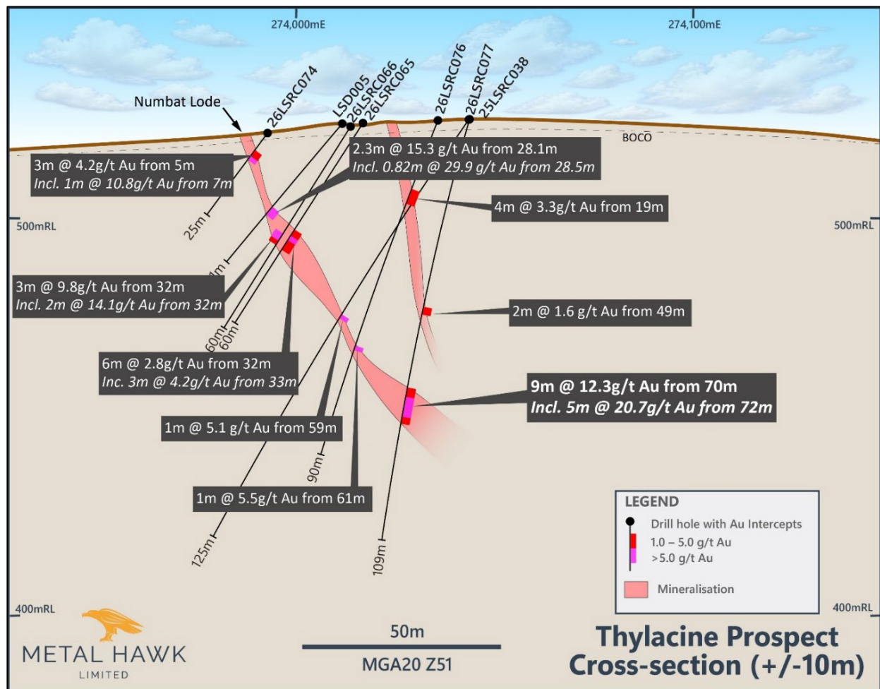
Figure 4. Cross-section of the Numbat lode looking north
