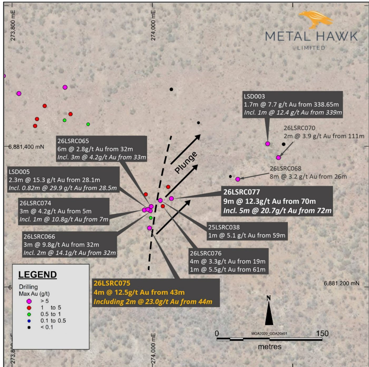
Figure 3. Thylacine south zone drilling (max Au g/t). Holes intersecting the Numbat lode labelled white; 26LSRC075 resplit result (reported 8 October 2026) labelled orange
