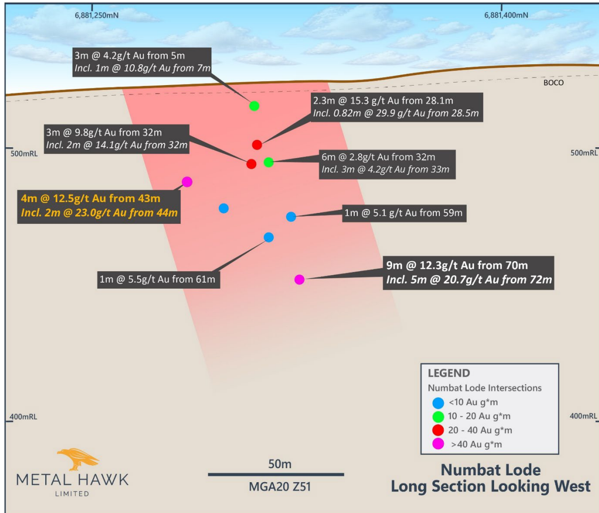
Figure 5. Long section looking west, showing Numbat drill intersections. Numbat shear zone intersection result labelled yellow.
