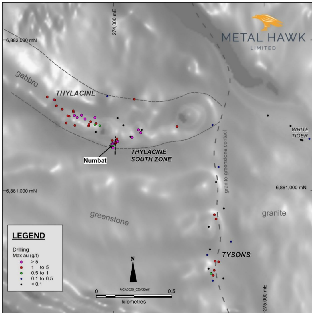
Figure 6. Leinster South drilling (max Au g/t)
