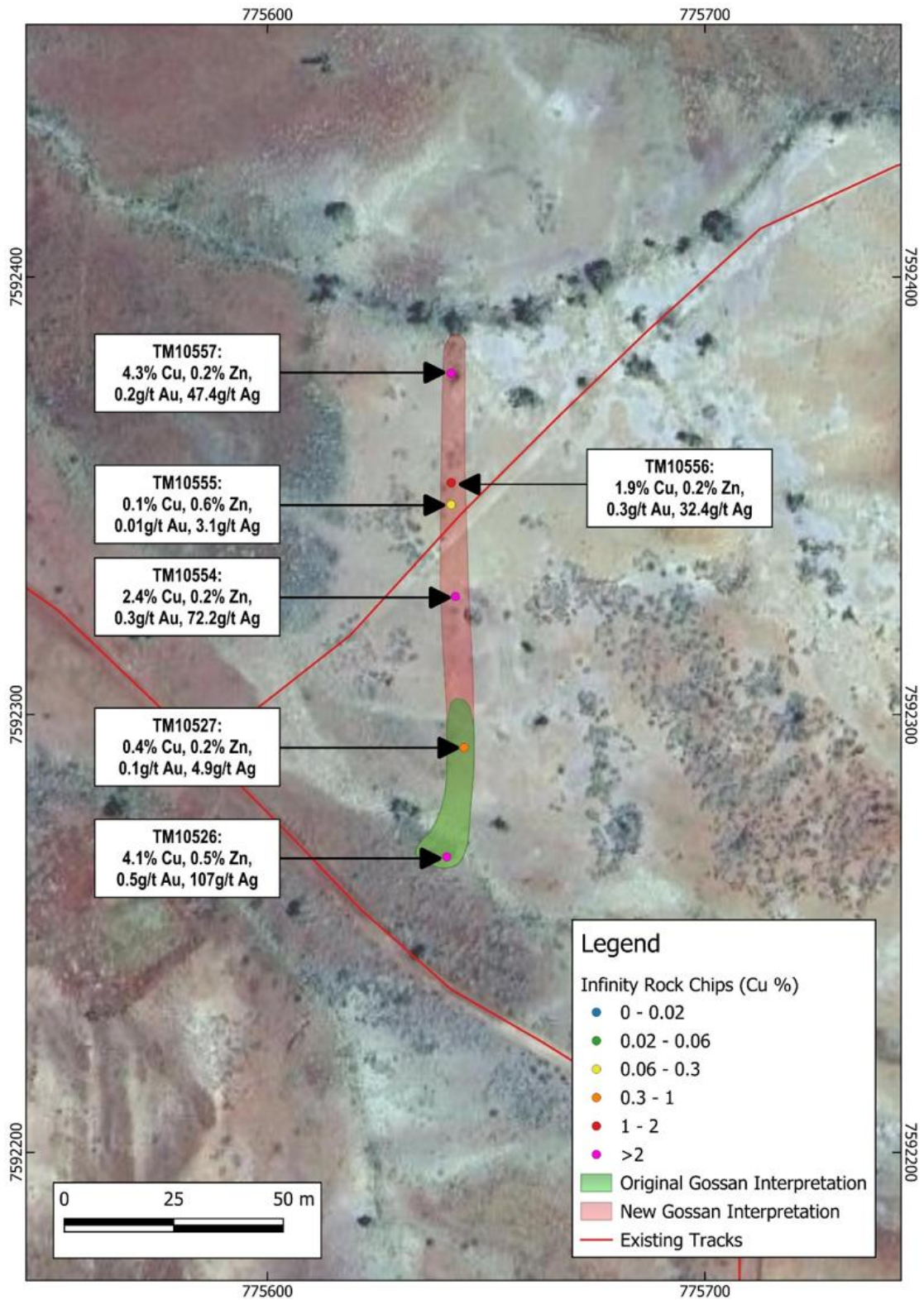
Figure 3: Image showing extended Gossan Interpretation in the Northern Trend
