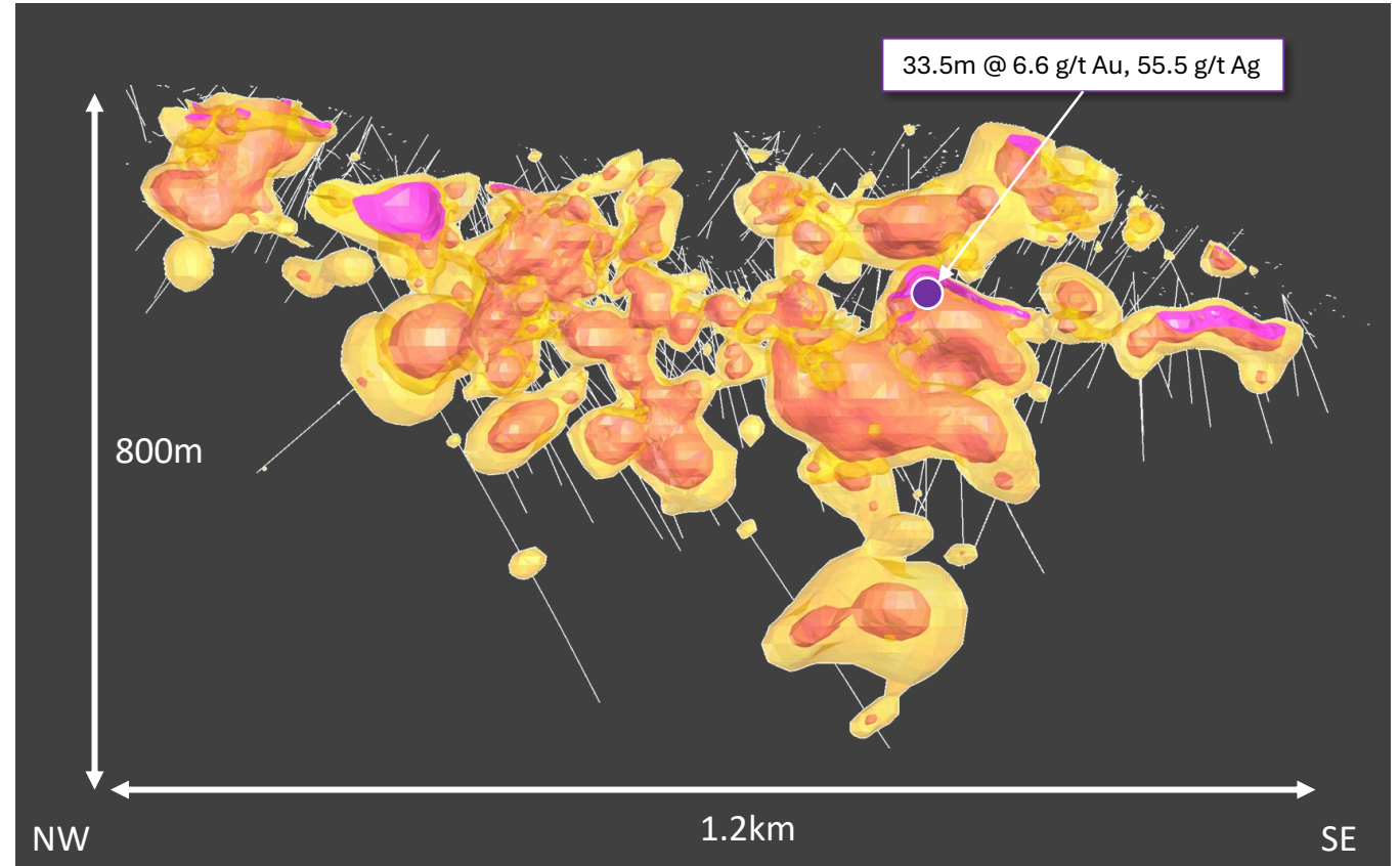
Cerro Verde long section displaying drill traces and 5 and 10 Au gram gold metre contours (Not MRE), 1.2km wide viewing plane
