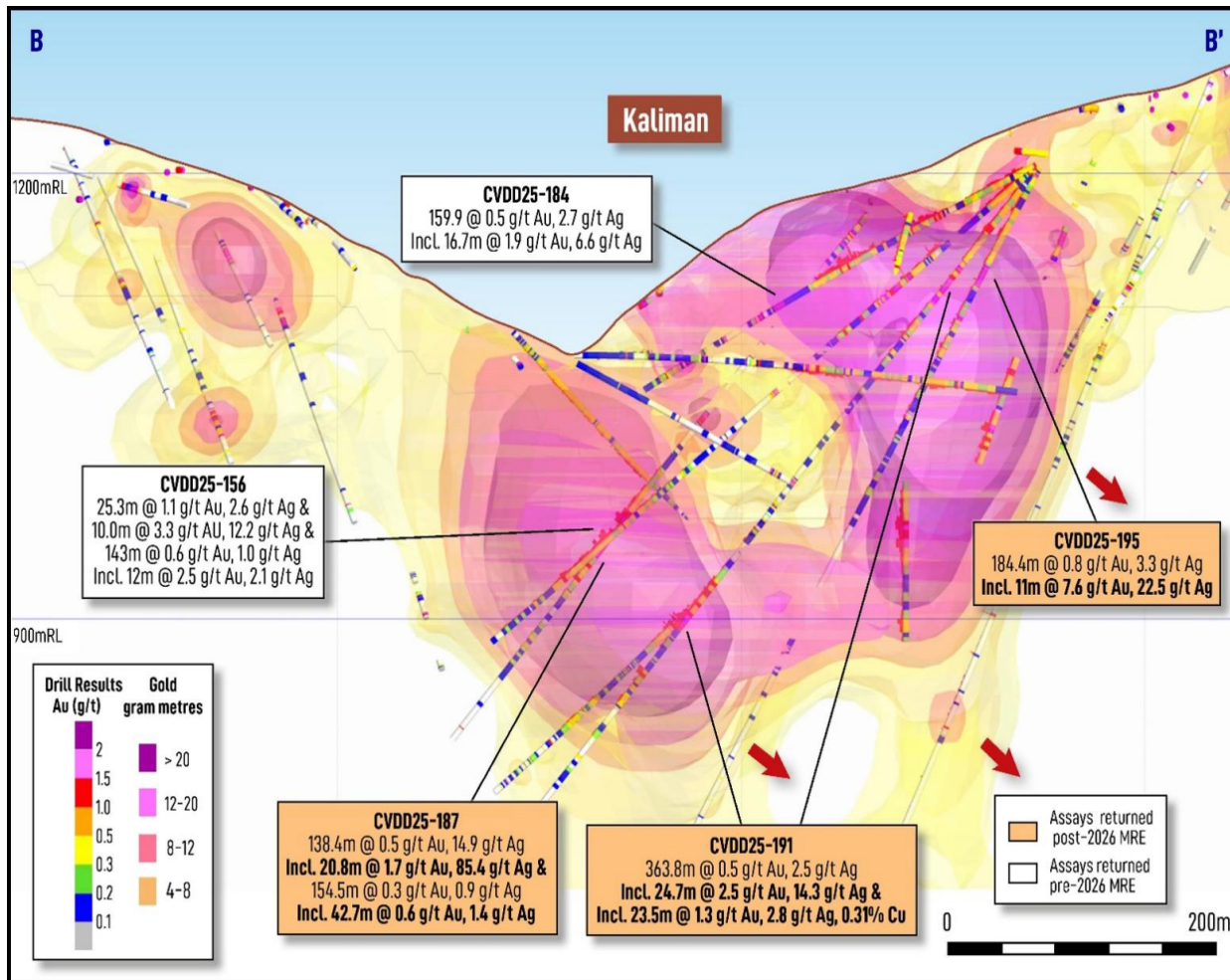
Cross section showing porphyry hosted mineralisation from surface at Cerro Verde
