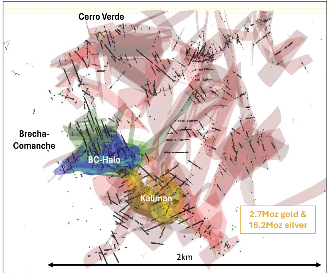
Plan view of Cerro Verde deposits showing drill hole traces and mineralisation domains
