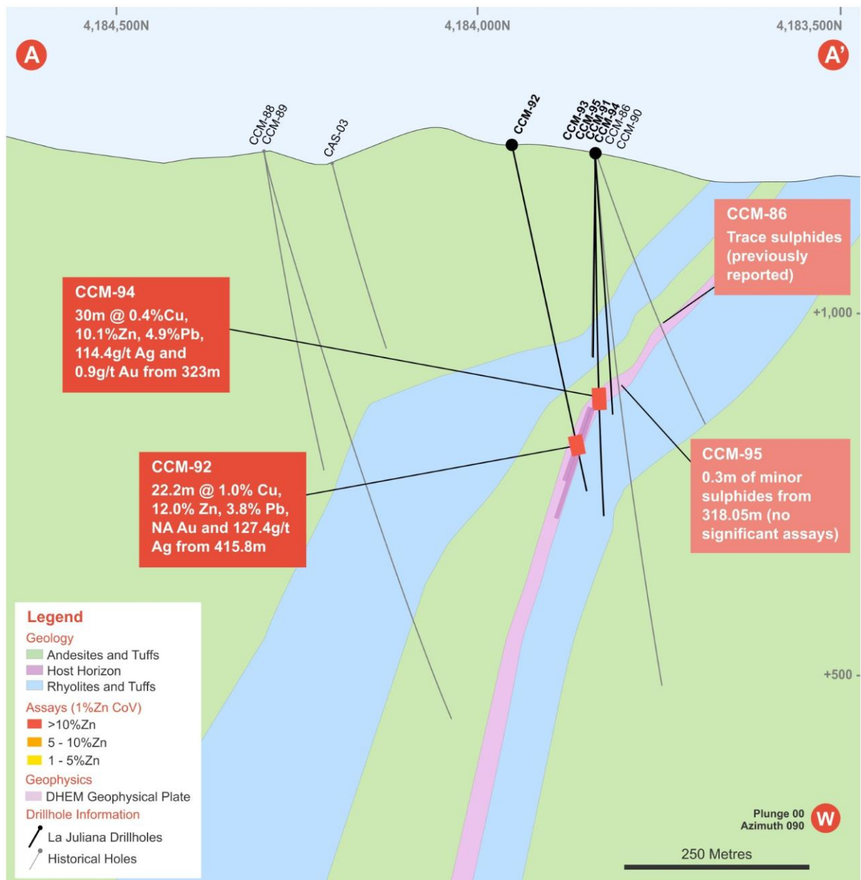
Figure 2 – La Juliana cross-section showing CCM-92 and CCM-94 with modelled DHEM off-hole geophysical plate from CCM-95.
