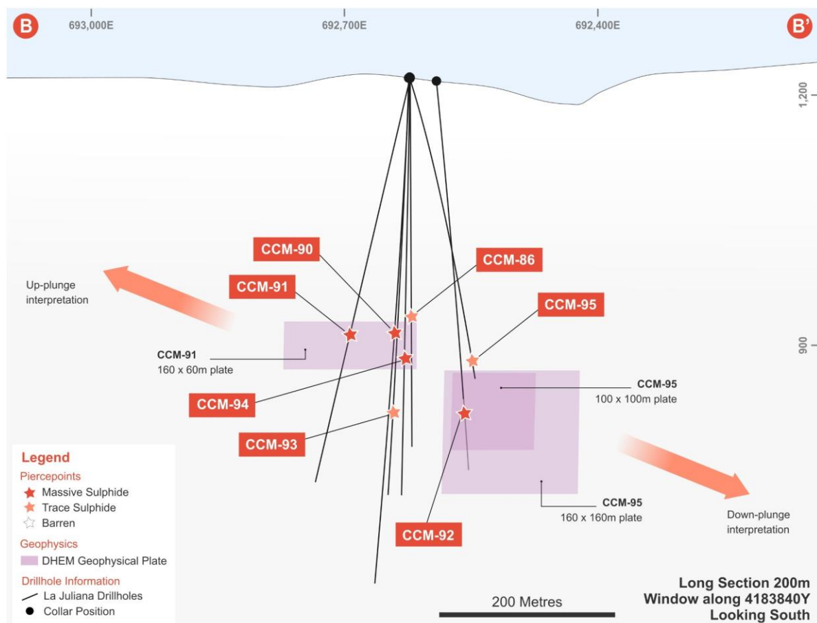
Figure 6 – La Juliana long section (4183840Y) showing drillhole pierce points and modelled DHEM conductor plates, indicating potential for the mineralised horizon to extend east and down-plunge to the west
