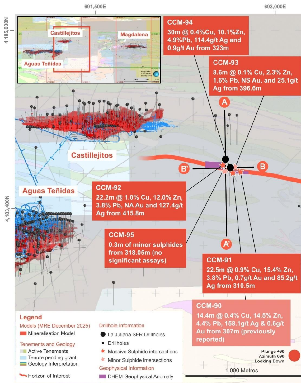
Figure 1 – La Juliana plan view showing drillhole collars and traces, with drilling confirming massive sulphide mineralisation over ~160m of strike and DHEM conductor plates indicating potential for at least ~350m of strike based on current data, with the system remaining open.
