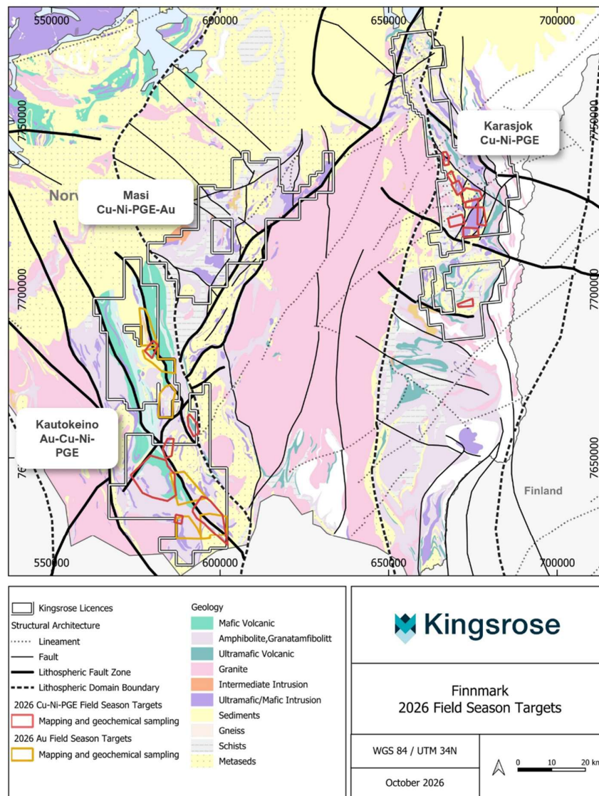
Figure 2: Finnmark 2026 field targets over regional geology and architecture interpretation.
