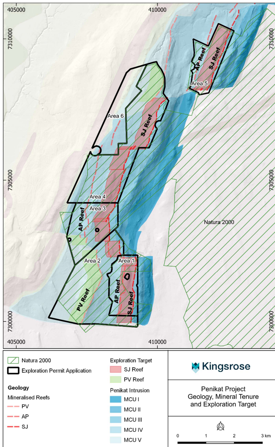
Figure 3: Kingsrose mineral tenure and geology of the Penikat Project.
