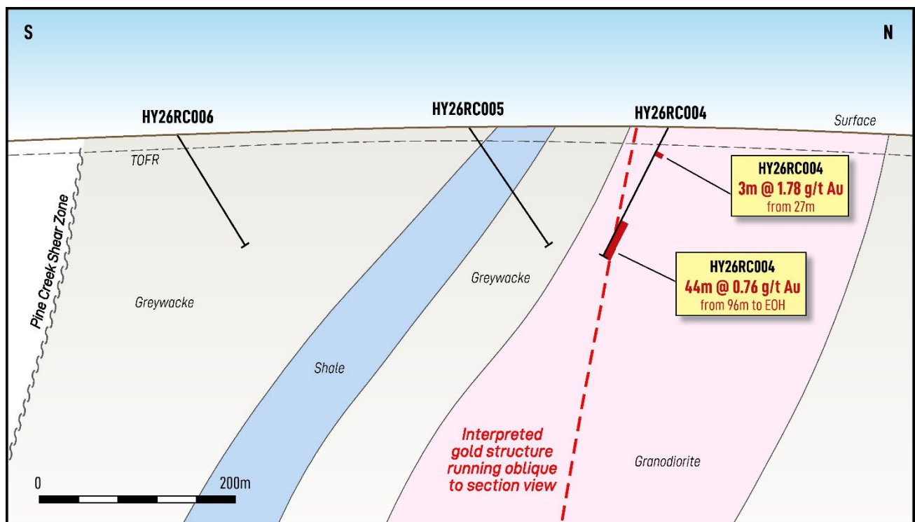
Figure 12: Cross-section looking west at HY26RC004 showing the wide gold intercept. Note the hole ended in mineralisation.
