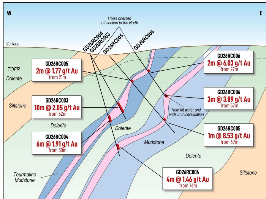
Figure 9: Cross-section A-A' looking north, showing significant drill intercepts and two interpreted mineralised lenses within each mudstone unit. GD26RC003 and GD26RC006 are projected onto the section as the holes were drilled oblique to the section. GD26RC006 was terminated early due to water and ended in mineralisation.
