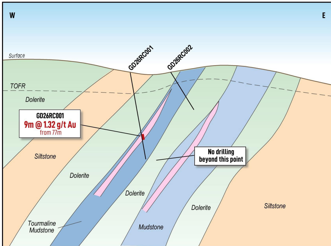
Figure 10: Cross-section B–B' looking north, showing the significant intercept in GD26RC001 and the interpreted hanging-wall and footwall mineralised lenses. GD26RC002 did not extend deep enough to test the footwall lens.
