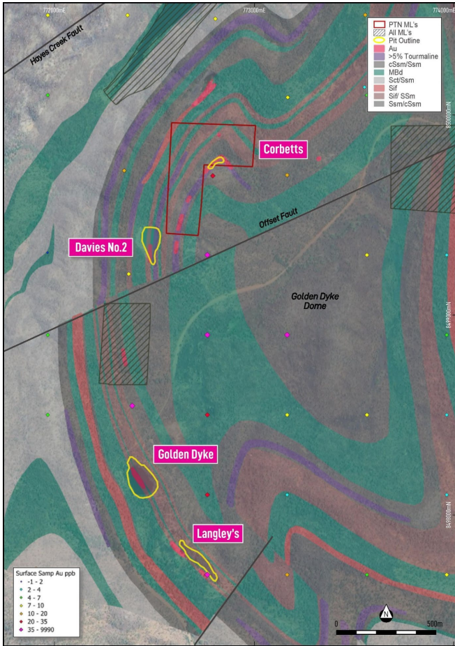
Figure 7: Golden Dyke Dome showing historical pits, interpreted geology digitised from Geopecko (1981) mapping and 2025 lag sampling highlighting the surface gold anomaly.
