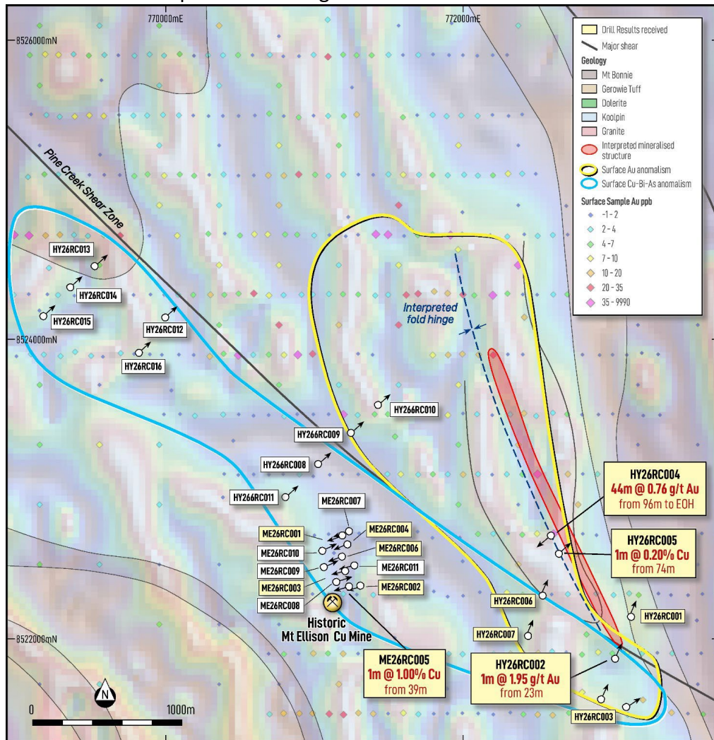
Figure 11: Plan view of Hydra and Hydrellison holes showing recent RC holes with PTN surface sampling.
