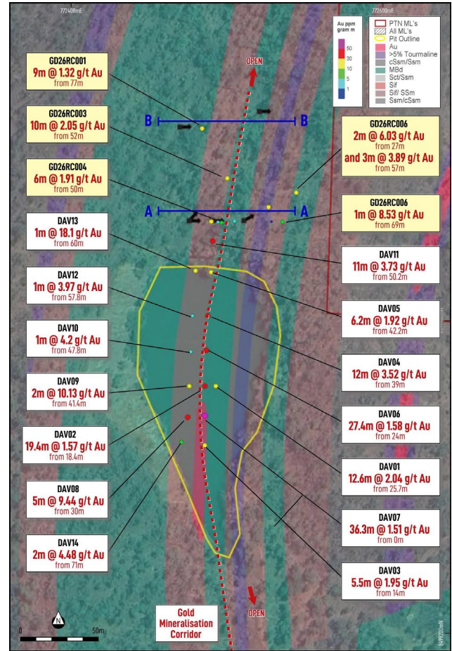
Figure 8: Plan view of Davies No.2 showing recent and validated historical drill-holes and the outline of the historical pit. Mineralisation remains open along strike to the north and south.
