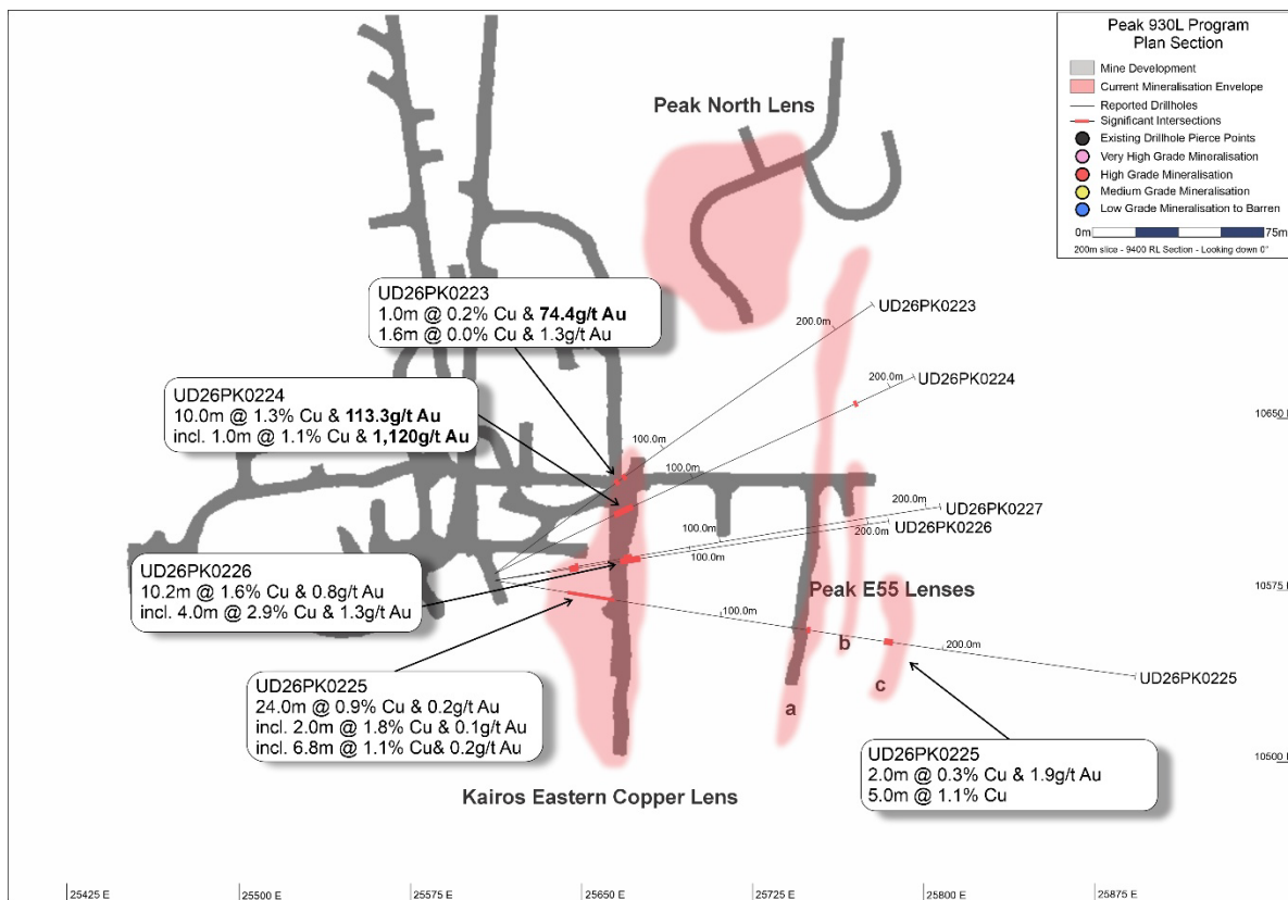
Figure 5: Plan section of the Kairos Eastern Copper Lens and the Peak E55 Lenses (a, b, c) showing mine development, visible mineralisation envelopes guided by existing drilling and currently reported drillholes.
