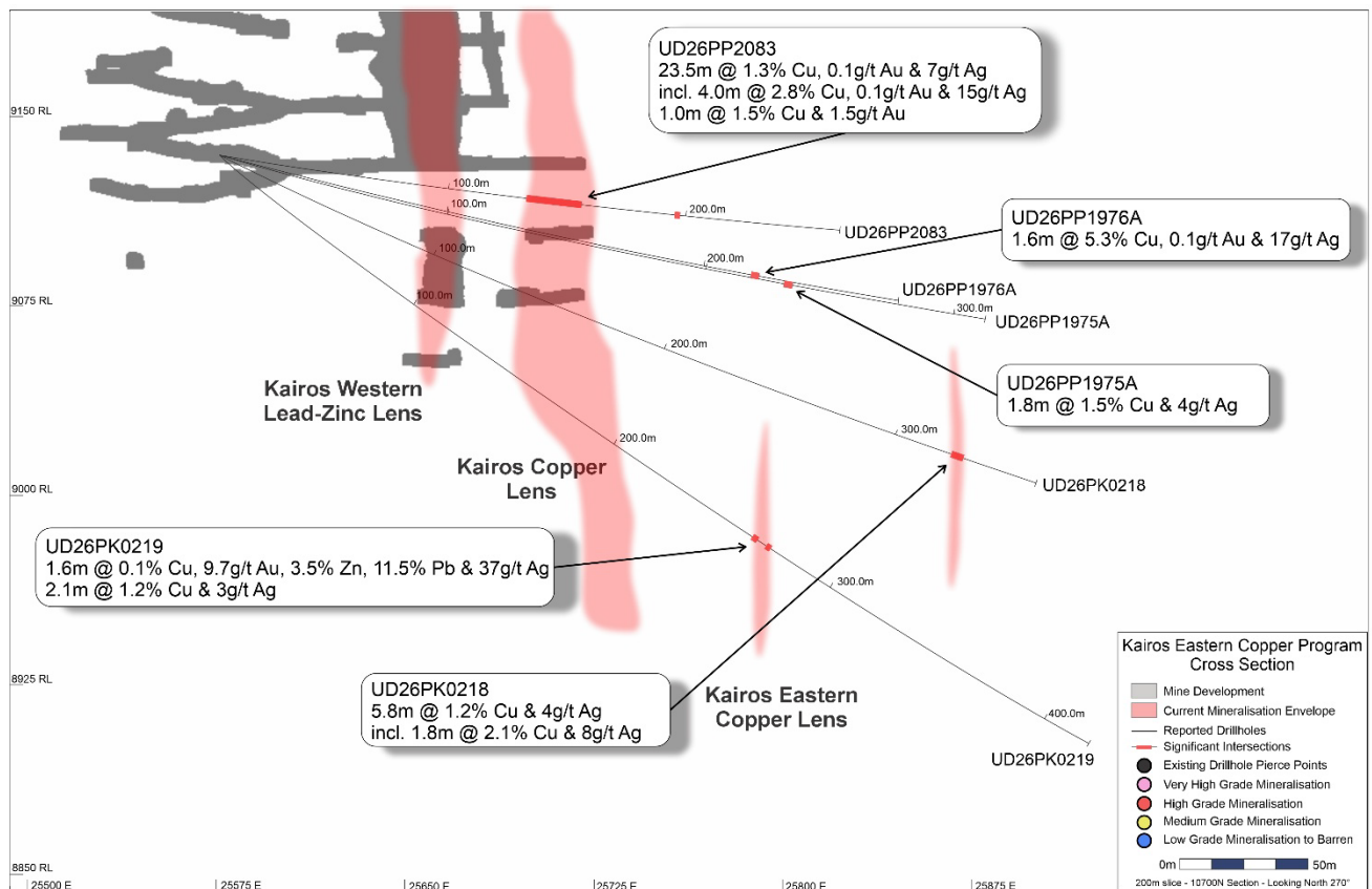
Figure 9: Cross section of the Kairos Eastern Copper Lens drill program showing mine development, visible mineralisation envelopes guided by existing drilling, and currently reported drillholes with significant intersections.
