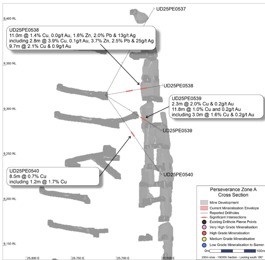
Figure 14: Cross section of the Perseverance Zone A drill program showing mine development, visible mineralisation envelopes guided by existing drilling, and currently reported drillholes with significant intersections.
