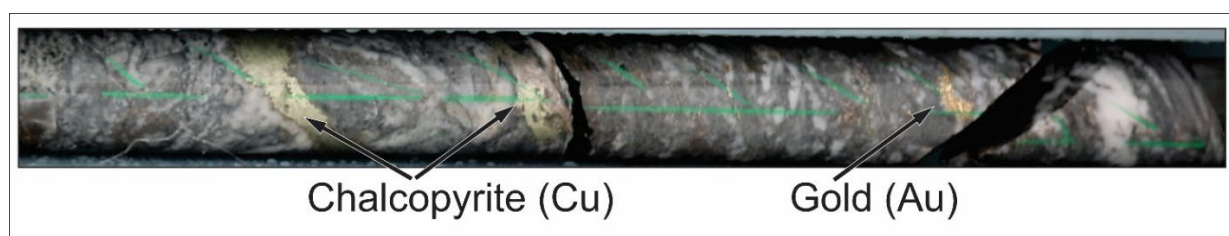
Figure 4: Drillcore from drillhole UD26PK0224 showing visible gold from 63.4m to 63.8m within significant intersection 1.0m @ 1.1% Cu and 1,120g/t Au from 63.0m.
