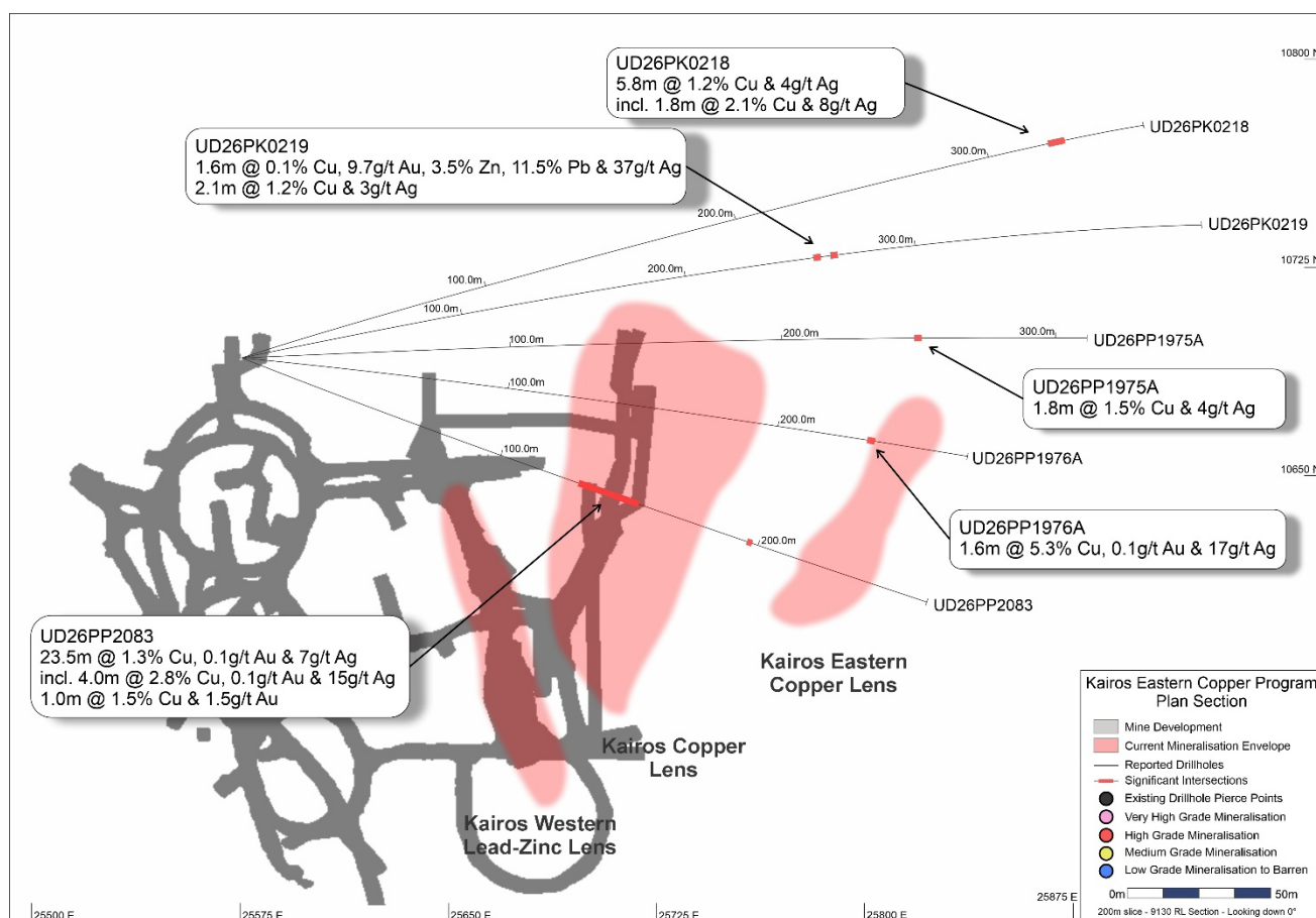
Figure 8: Plan section of the Kairos Eastern Copper Lens drill program showing mine development, visible mineralisation envelopes guided by existing drilling, and currently reported drillholes with significant intersections.
