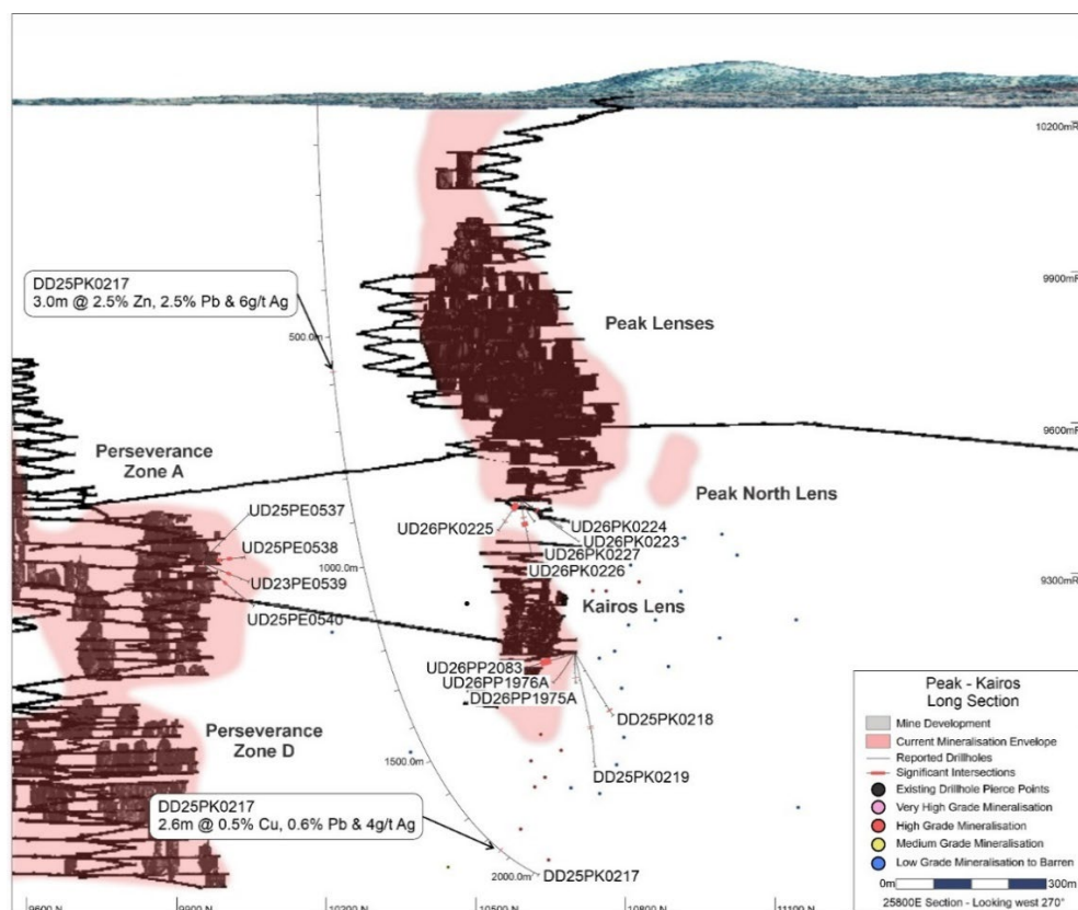
Figure 10: Long section of the Peak South Mine area with Peak, Kairos and Perseverance deposits, and the Kairos East Copper, Peak-Kairos, Perseverance Zone A and Lower Kairos drill programs along with mine development, the existing visible mineralisation envelope, and currently reported drillholes with significant intersections.
