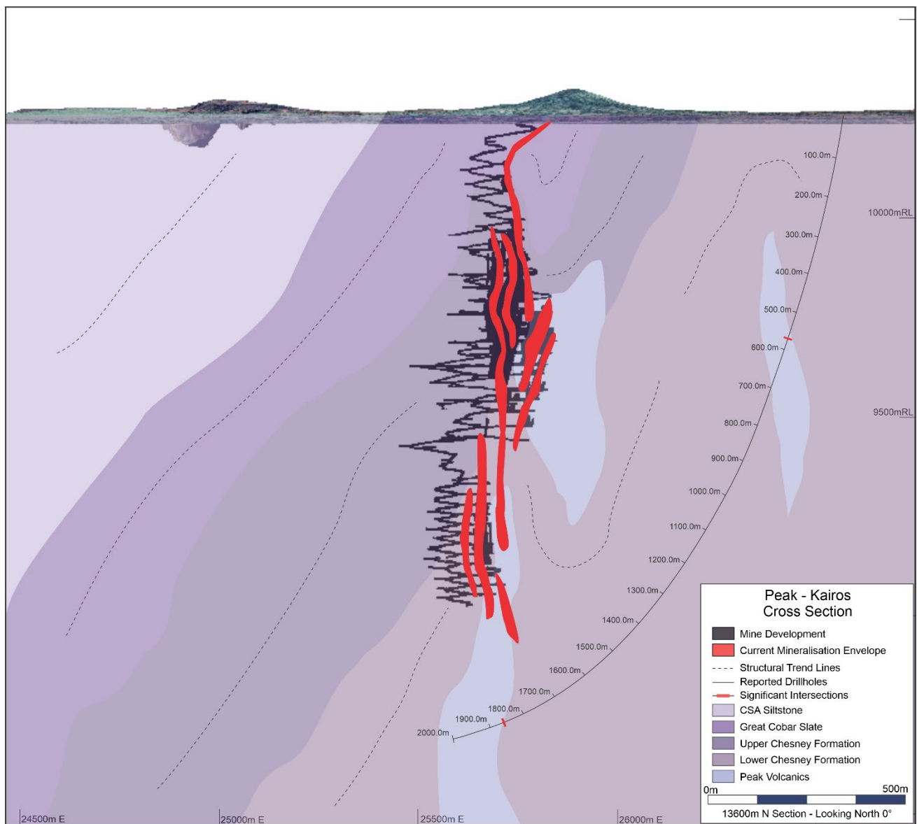
Figure 11: Generalised cross-section of the Peak South Mine area with Peak and Kairos deposits, with current mine development, visible mineralisation envelopes, interpreted geology, structural trends and currently reported drillholes with significant intersections.
