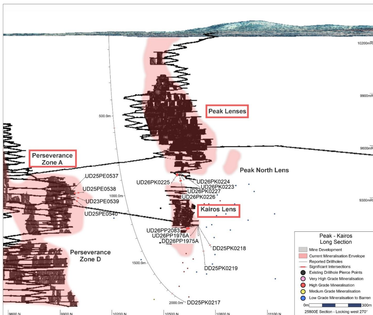
Figure 1: Long section of the Peak South Mine area with Peak, Kairos and Perseverance deposits, along with mine development, the existing visible mineralisation envelope, and currently reported drillholes with significant intersections.
