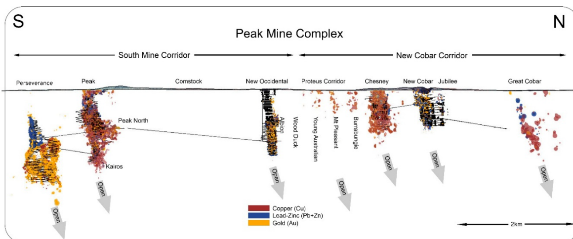
Figure 3: Long section of the Peak Mine Complex including Peak South Mine and New Cobar Mine areas, and individual deposits with generalised metal distribution
