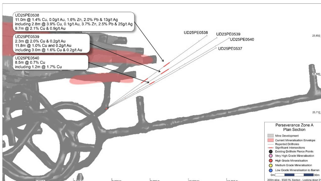
Figure 12: Plan section of the Perseverance Zone A drill program showing mine development, visible mineralisation envelopes guided by existing drilling, and currently reported drillholes with significant intersections.
