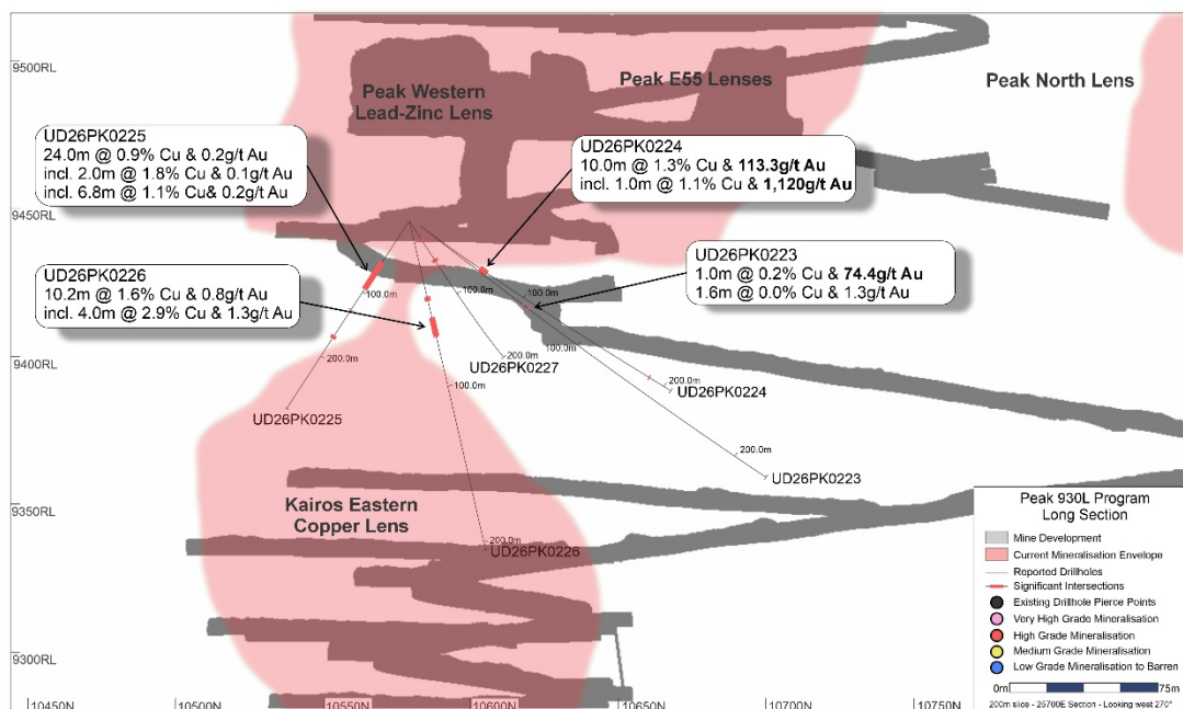
Figure 7: Long section of the Kairos Eastern Copper Lens and the Peak E55 Lenses showing mine development, visible mineralisation envelopes guided by existing drilling and currently reported drillholes.
