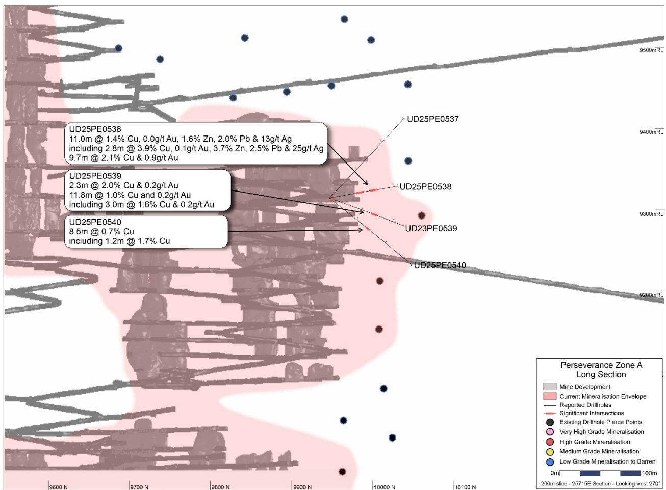
Figure 13: Long section of the Perseverance Zone A drill program showing mine development, visible mineralisation envelopes guided by existing drilling, currently reported drillholes with significant intersections and historical drillhole pierce points
