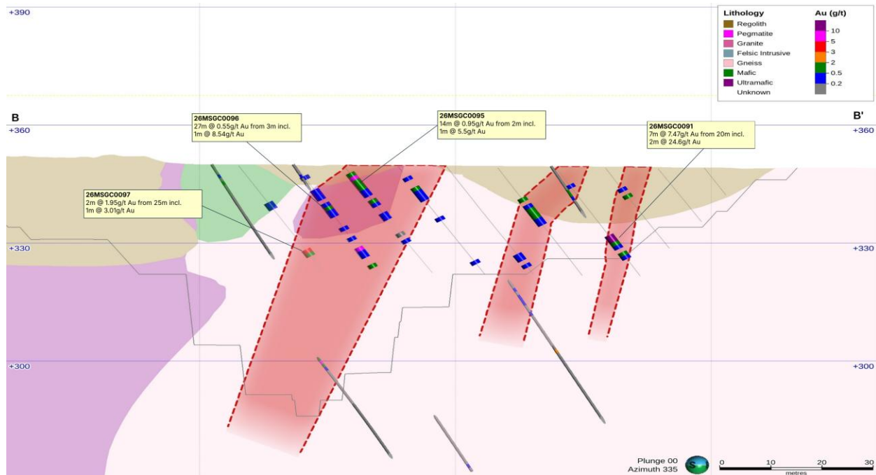
Figure 3: Cross section B–B' showing significant intercepts in holes 26MSGC0091, 26MSGC0095, 26MSGC0096 and 26MSGC0097
