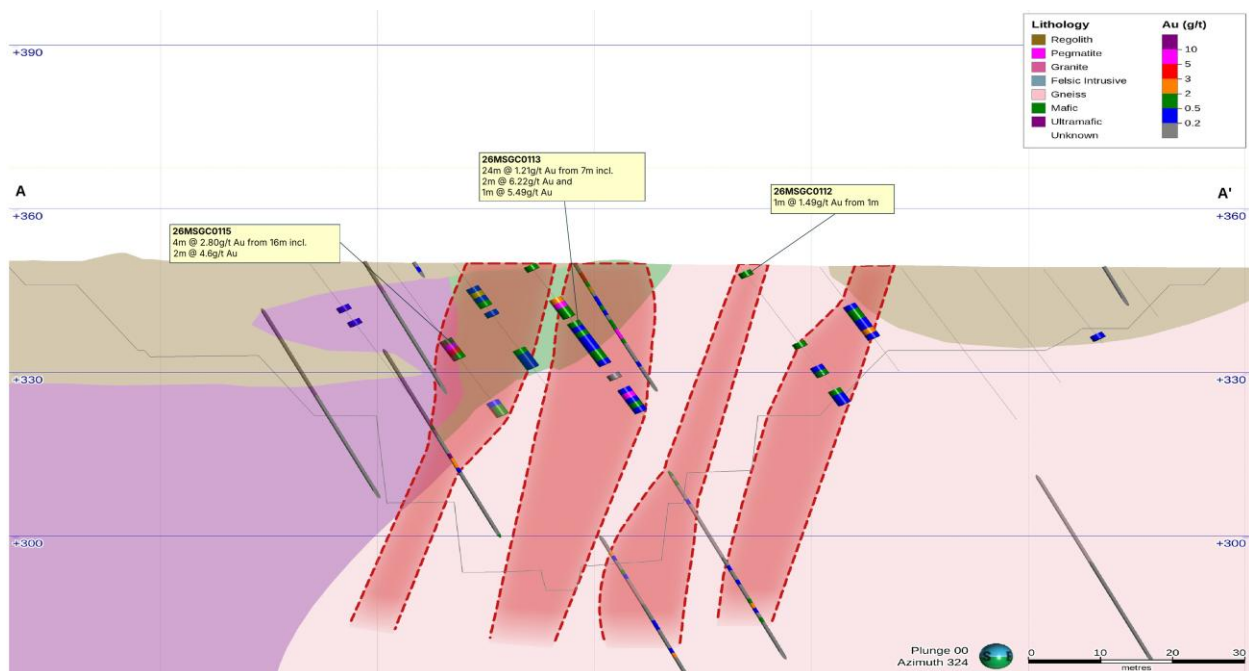
Figure 2: Cross section A–A' showing significant intercepts in holes 26MSGC0112, 26MSGC0113 and 26MSGC0115
