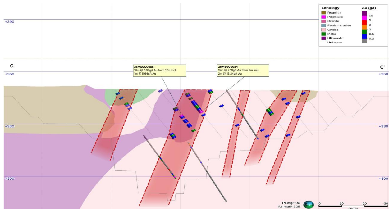
Figure 4: Cross section C–C' showing significant intercepts in holes 26MSGC0084 and 26MSGC0085
