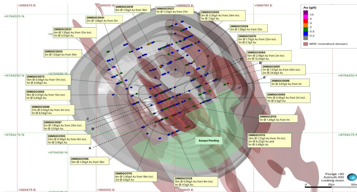
Figure 1: NW Pit plan view showing grade control drill holes (coloured by Au g/t), significant intercepts, MRE mineralised domains and the location of cross sections A–A', B–B' and C–C'
