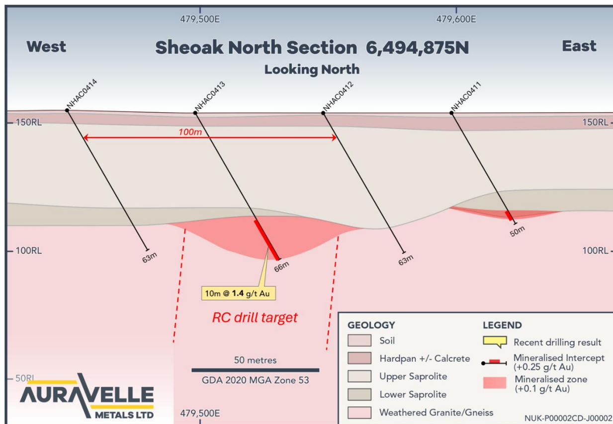
Figure 3: Sheoak North Prospect – Cross Section 6,494,875N
