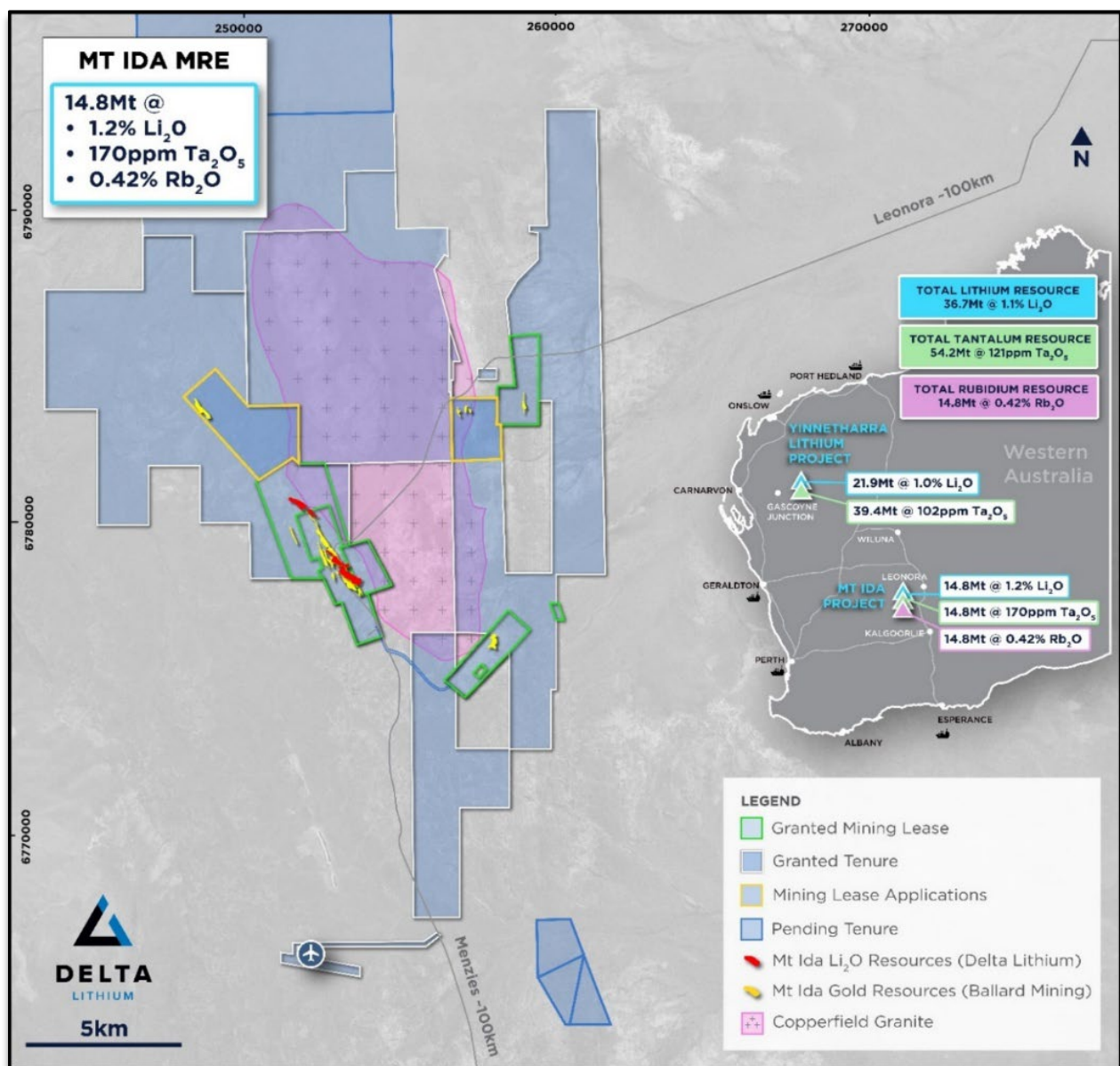
Figure 8: Mt Ida Project and Tenure with lithium, tantalum and rubidium resources
