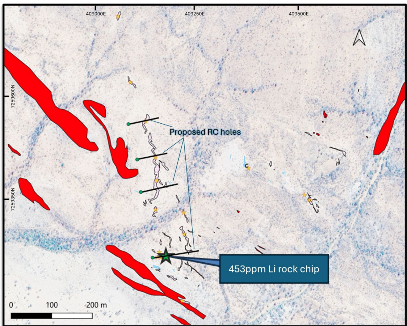
Figure 4: Bains Lithium target
