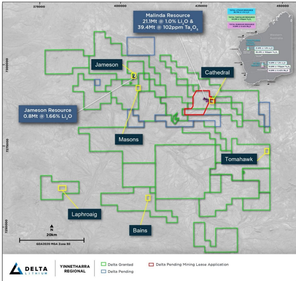
Figure 2: Yinnetharra Project and Tenure with current active prospects
