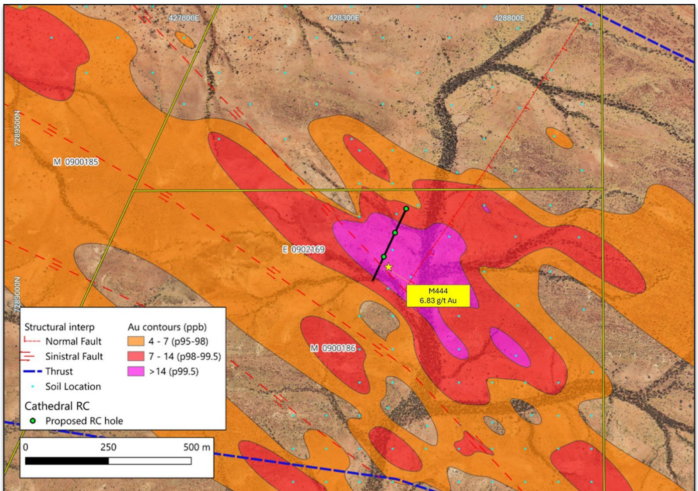
Figure 7: Cathedral Gold anomaly
