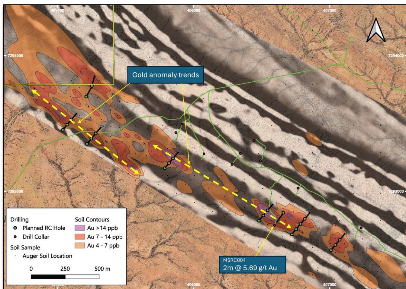
Figure 6: Masons Gold anomaly
