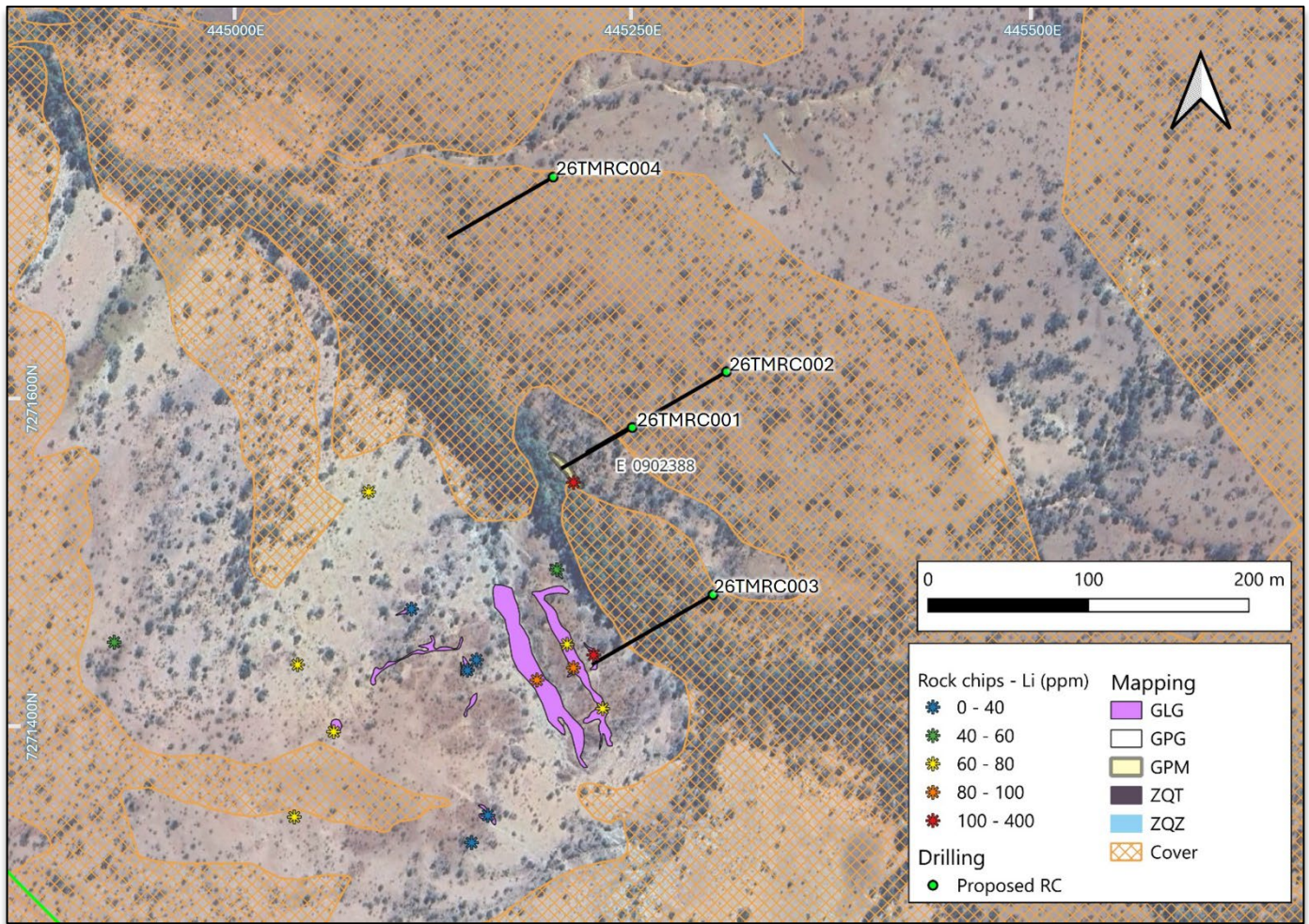
Figure 3: Tomahawk Lithium target
