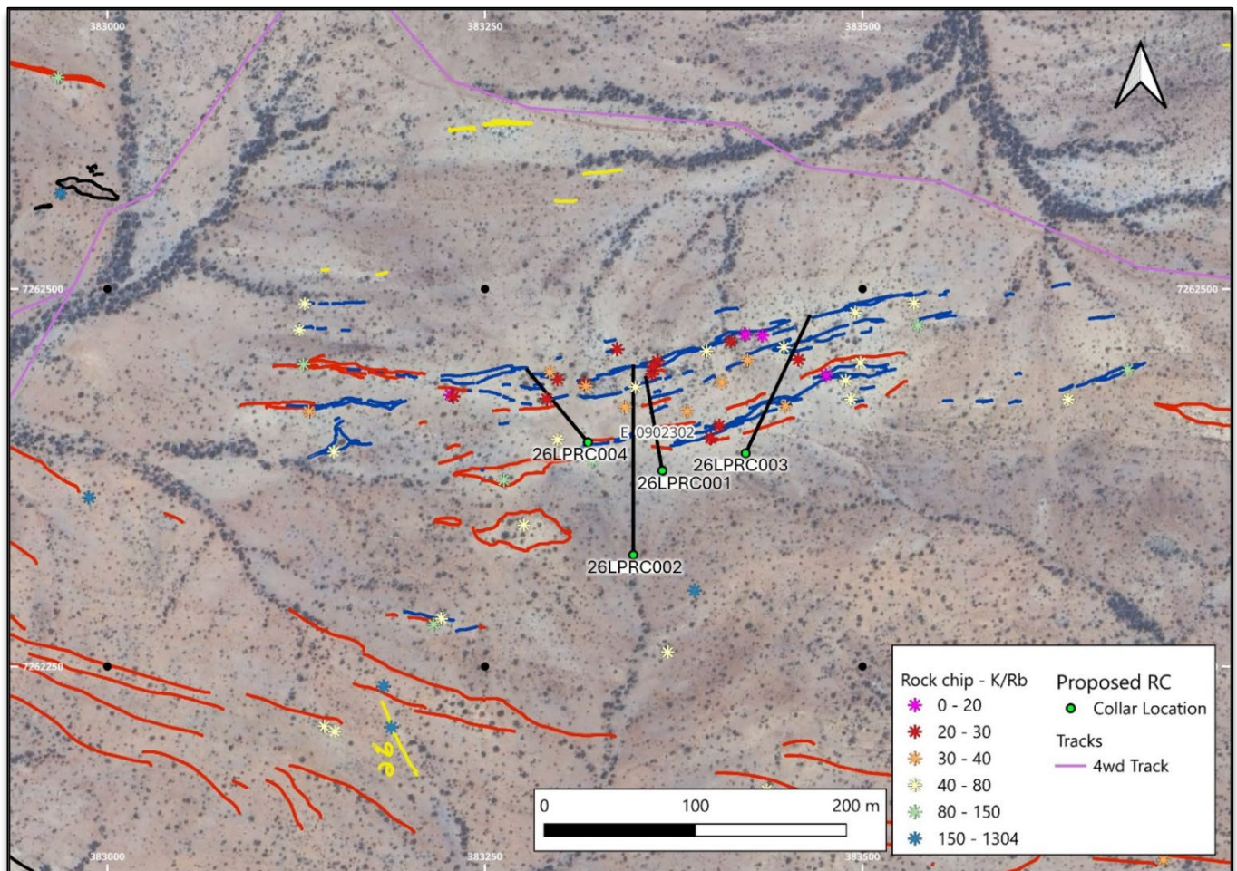
Figure 5: Laphroaig Lithium target
