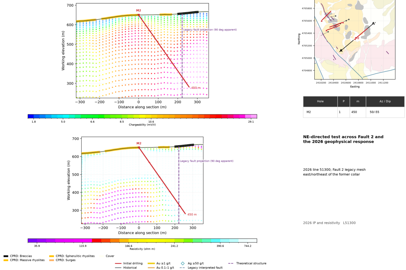
Figure 8 – Section SEC-11 showing SM26-016 (M2) drilled northeast across the interpreted Fault 2 and into the 2026 line 51300 chargeability (upper) and resistivity (lower) response.
