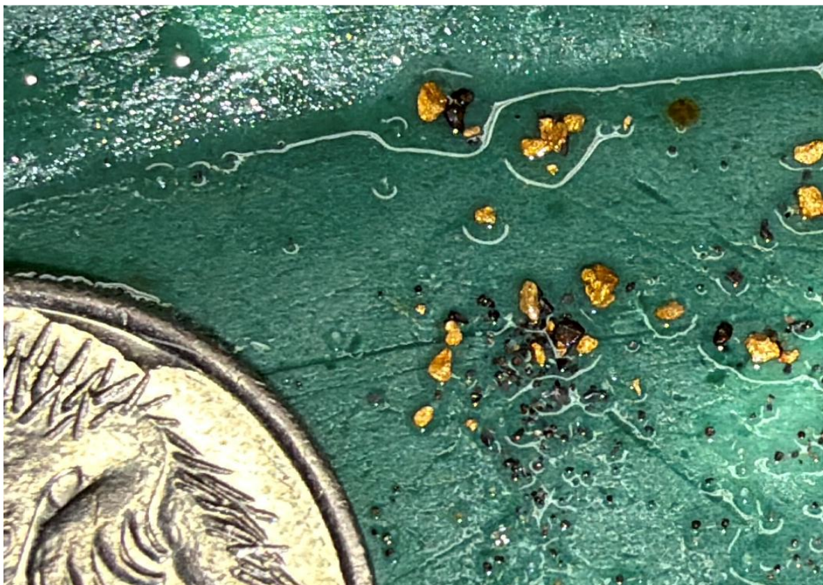
Figure 19 Gold in panned concentrate of interval PHAC2563 from 103-104m with a 5¢ coin for scale
