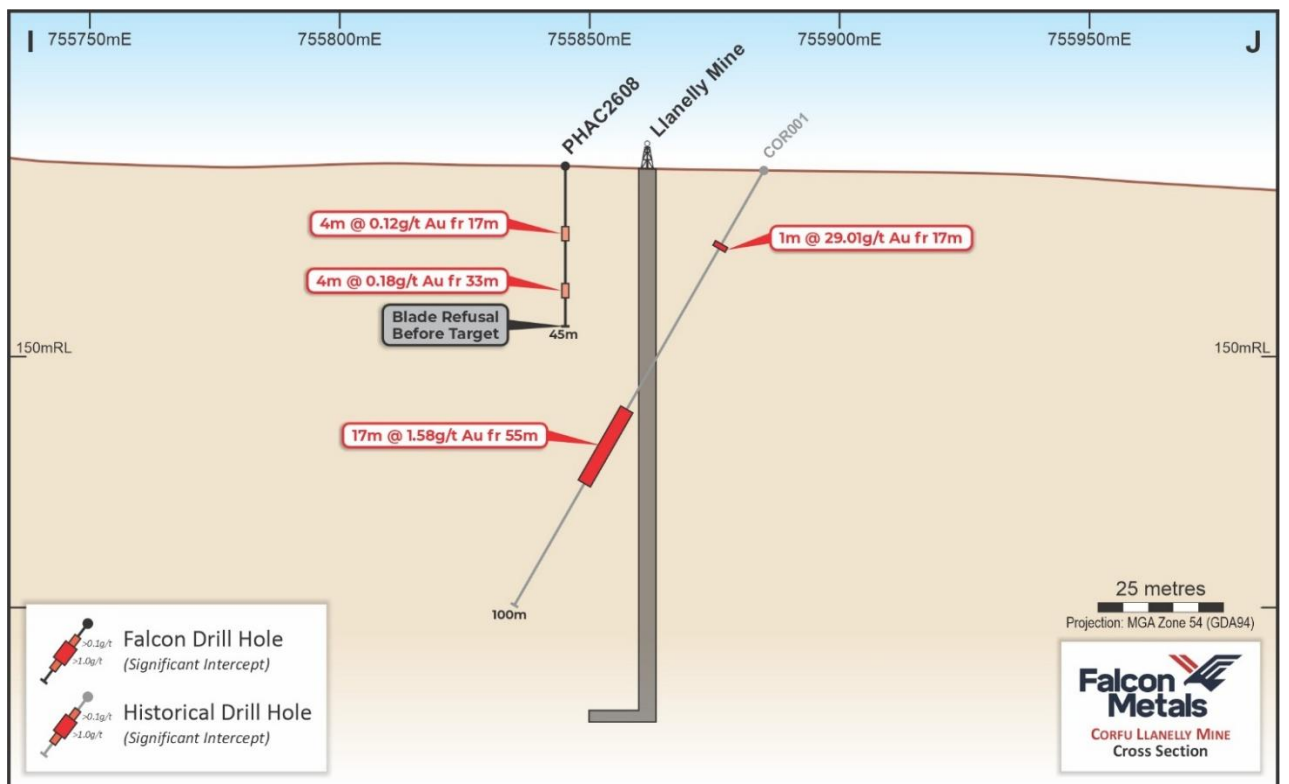
Figure 16 Cross section of I-J at the Corfu Reef showing historical and Falcon drilling
