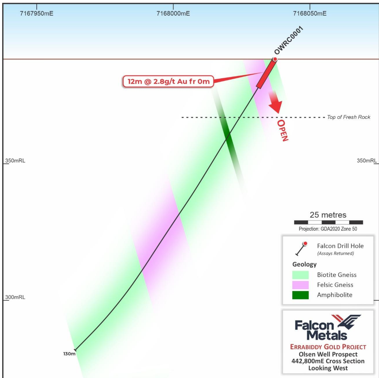
Figure 23 Cross section of OWRC0001 looking west
