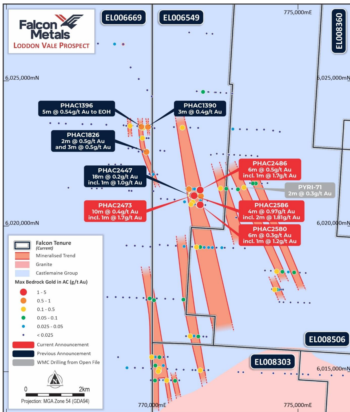
Figure 17 Location of Loddon Vale drilling and maximum gold in bedrock 11
