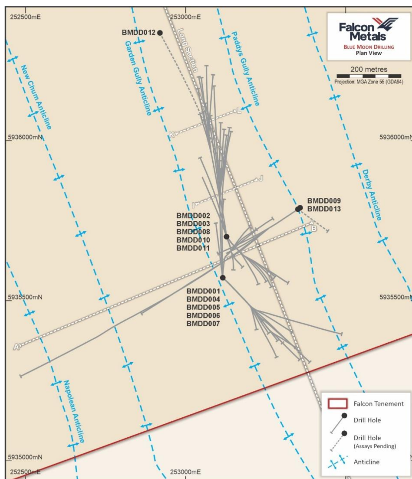
Figure 9 Plan map showing the collar positions for Blue Moon
