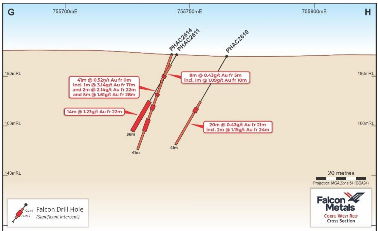
Figure 15 Cross section of G-H at the Corfu West Reef showing Falcon drilling
