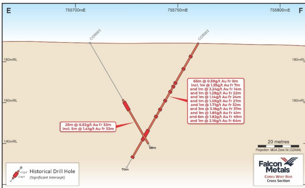
Figure 14 Cross section of E-F at the Corfu West Reef showing historical drill results
