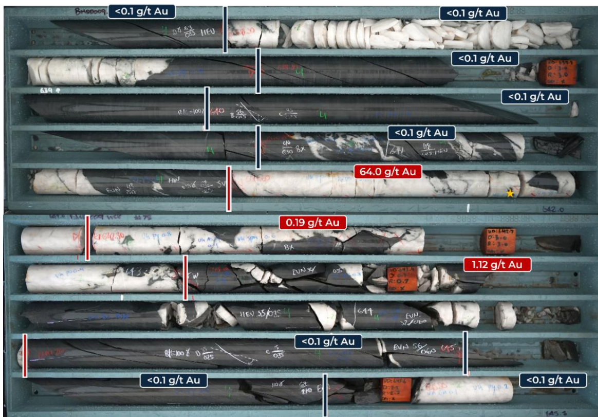
Figure 7 BMDD009W02 drill core with the yellow star highlighting occurrence of visible gold in Lotus Zone
