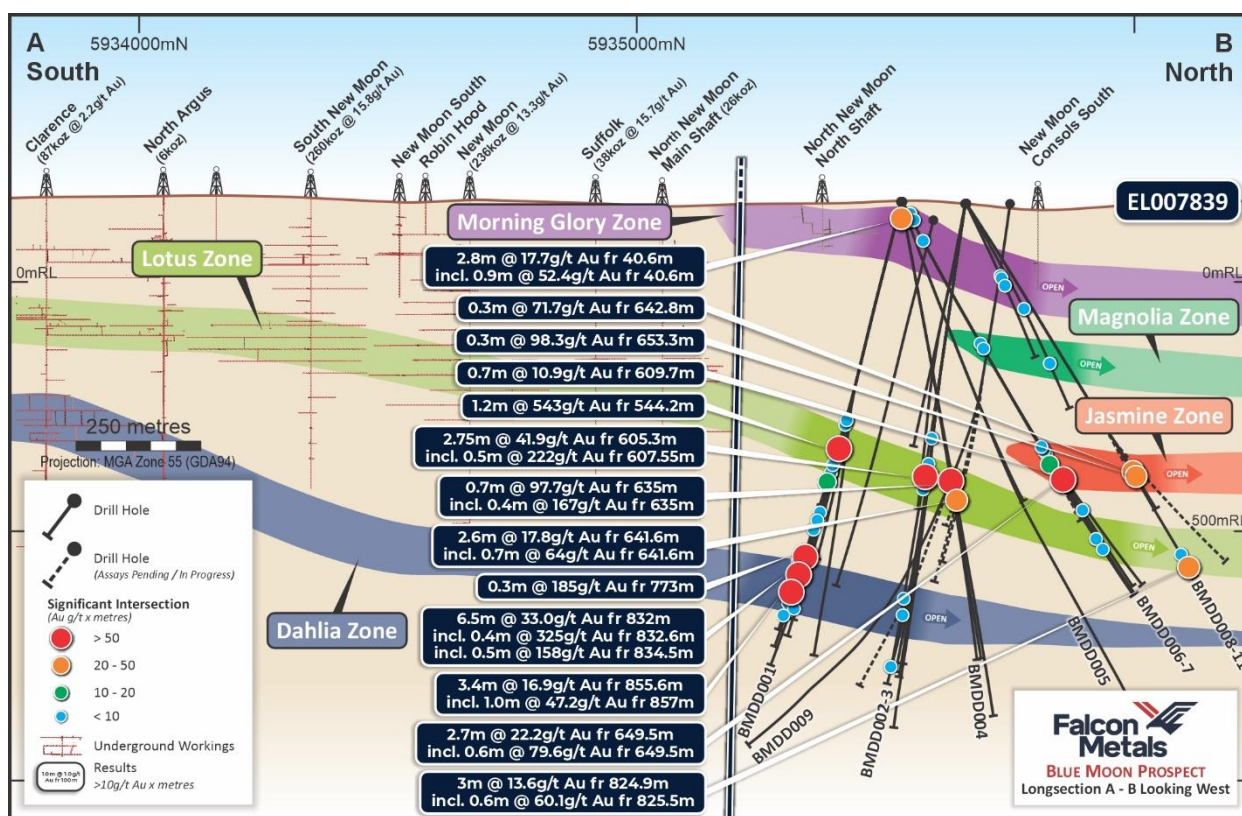
Figure 1 Long section of the Blue Moon drilling
