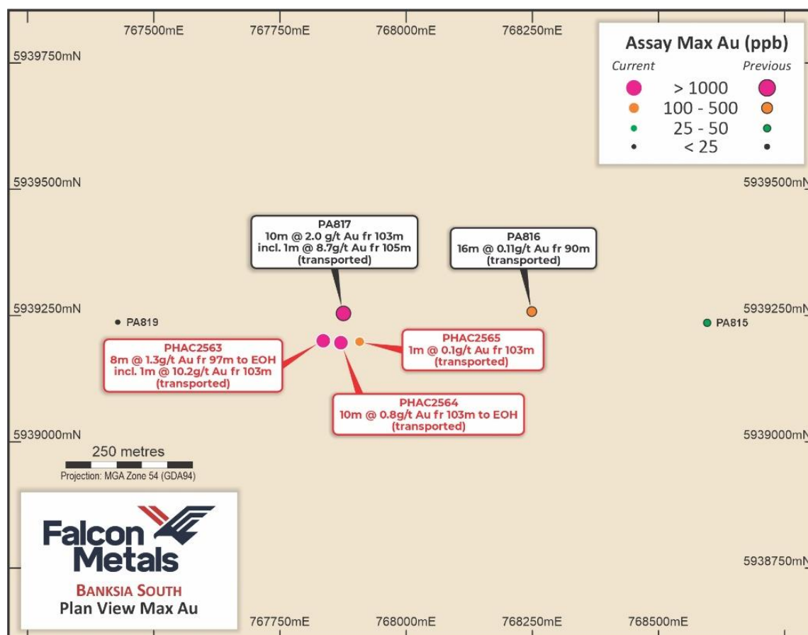
Figure 18 Plan view of maximum gold in holes at Banksia South
