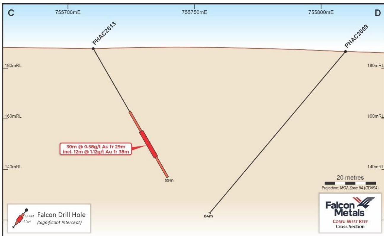
Figure 13 Cross section of C-D at the Corfu West Reef showing Falcon drilling
