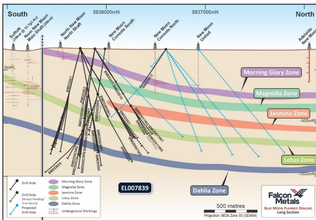
Figure 8 Current progress and planned step out drilling to the north showing interpreted target zones
