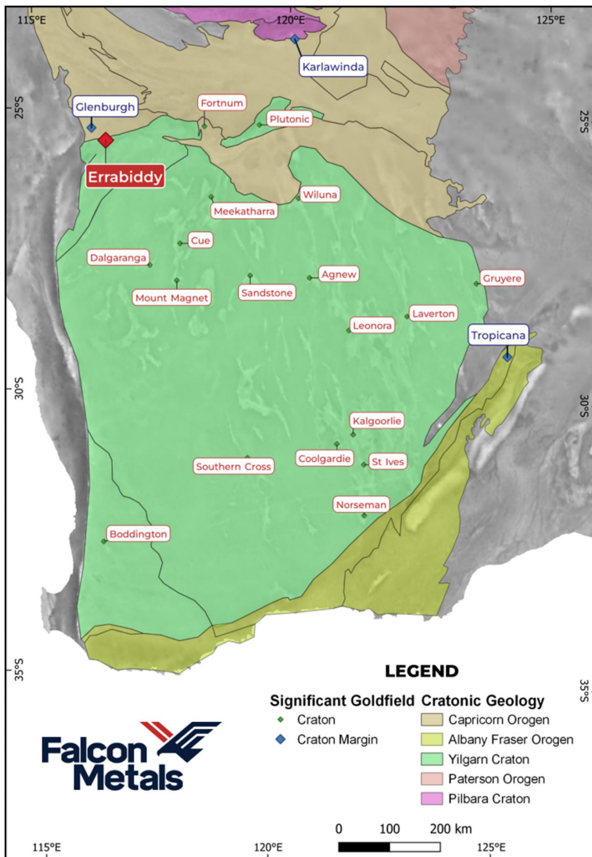
Figure 21 Geological setting of the Errabiddy Gold Project
