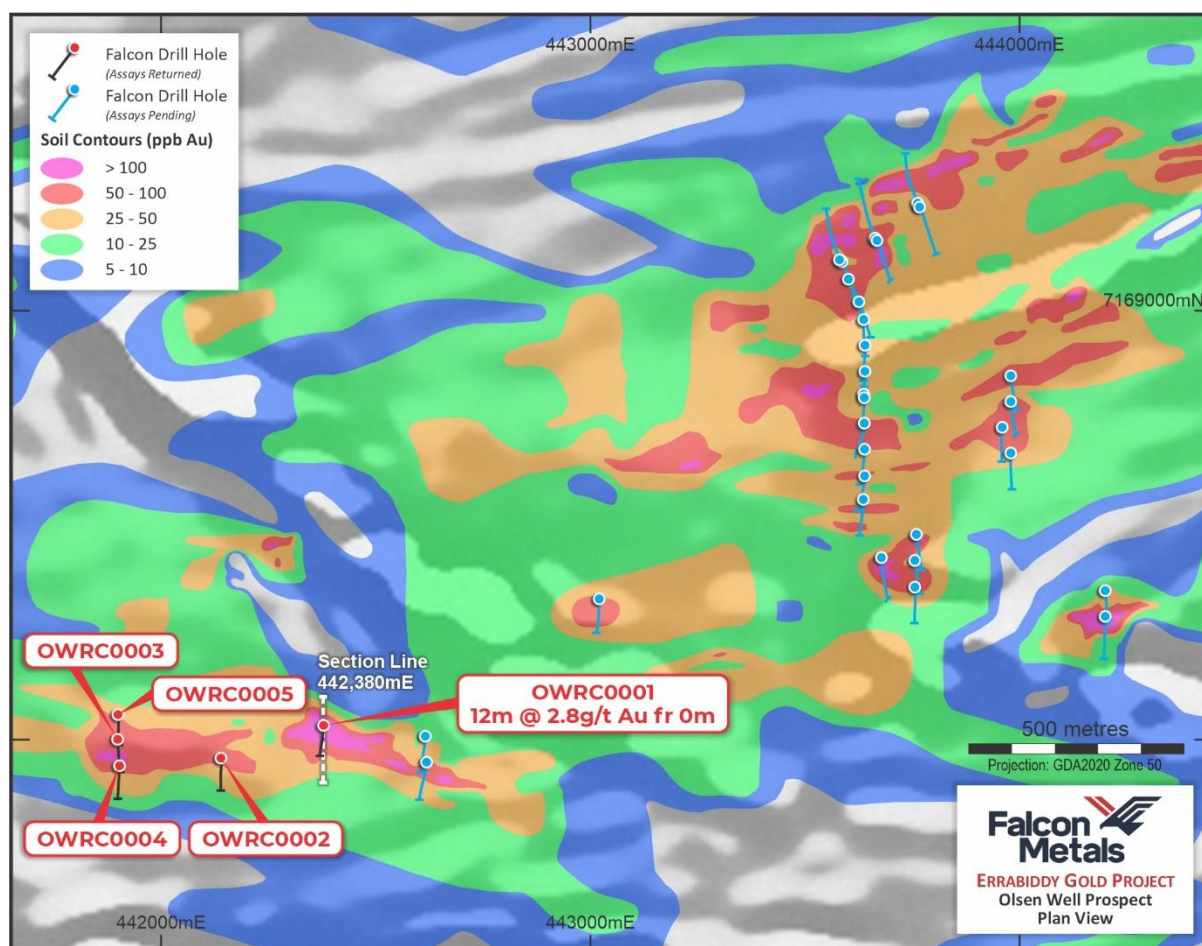
Figure 22 Plan map of drilling to date at Olsen Well with gold-in-soil contours on 2VD RTP magnetics
