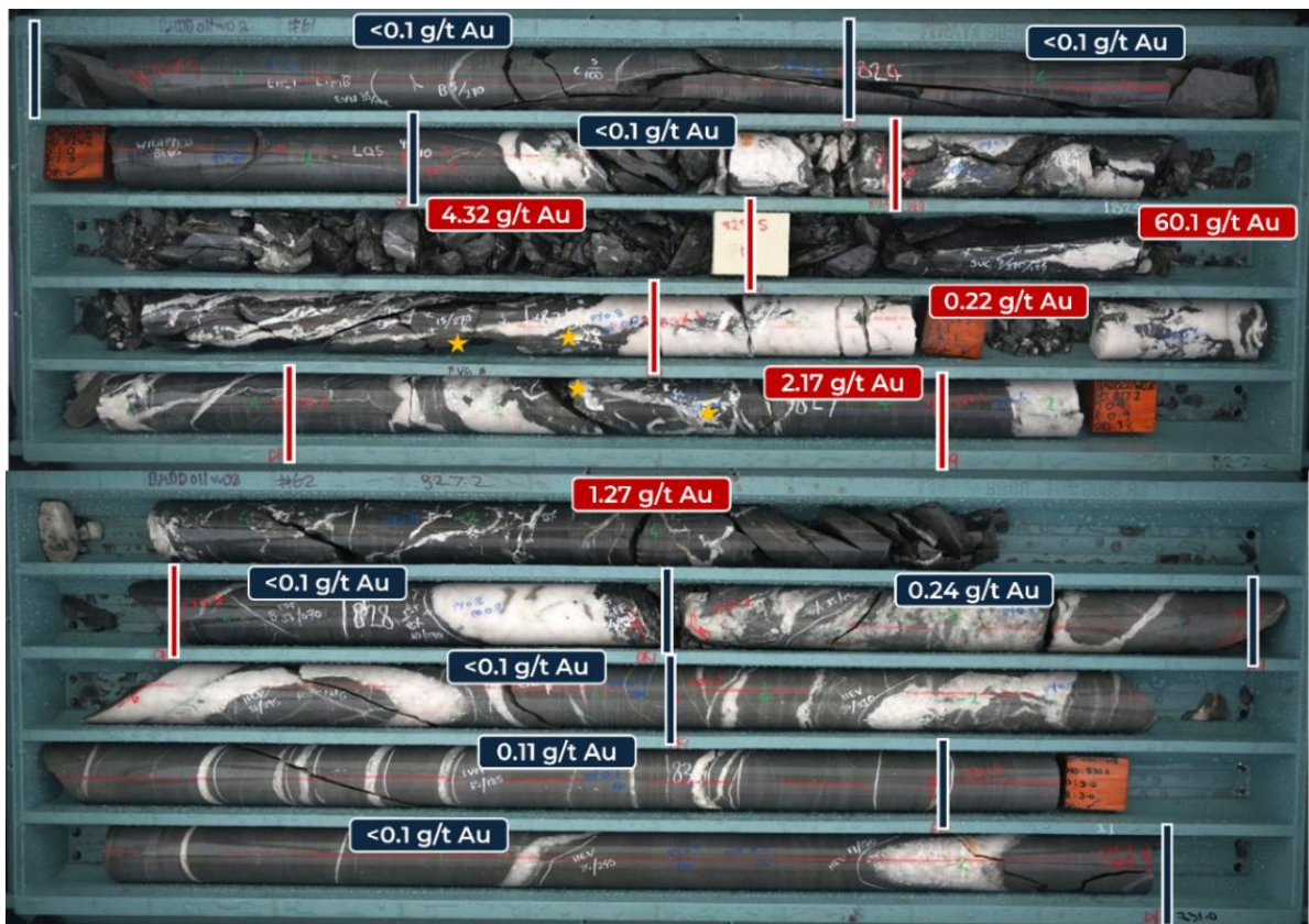
Figure 6 BMDD011W08 drill core with the yellow stars highlighting occurrences of visible gold in Lotus Zone
