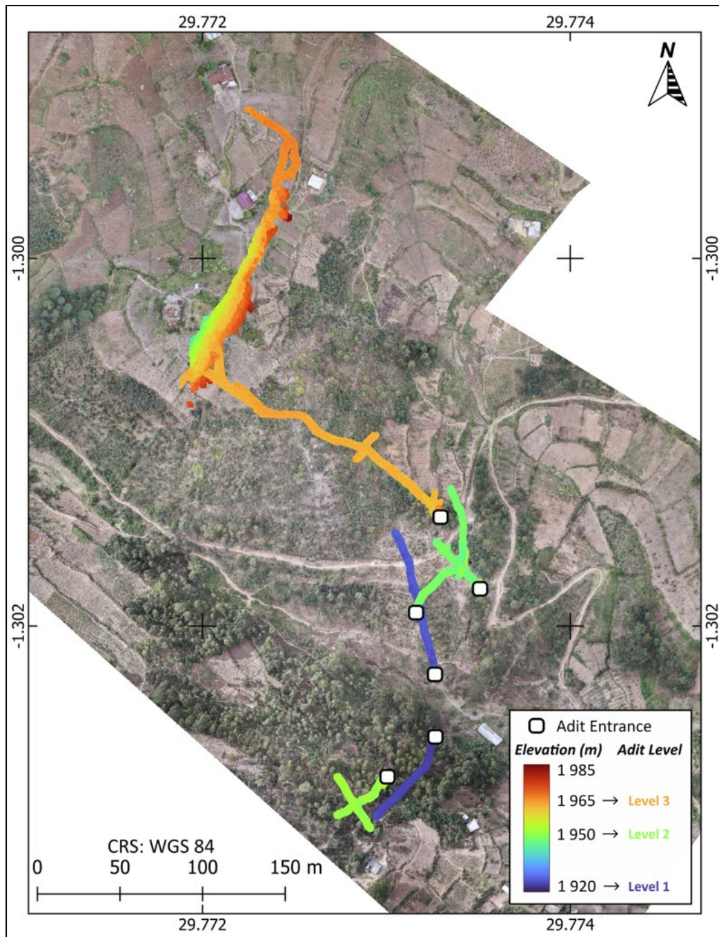
Figure 2: Plan view map showing the different adits that were scanned with the LiDAR. Note that the colour of the adit correlates to its actual elevation as per the legend.
