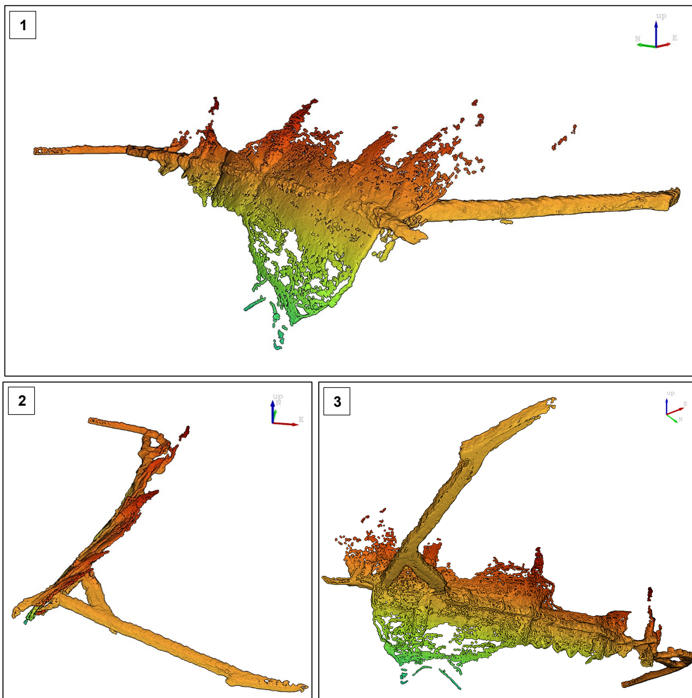
Figure 3: LiDAR images showing the geometry of the stoped-out section of the main Bahati vein in level 3 adit from various perspectives:
