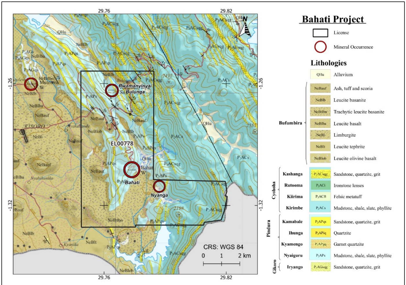
Figure 4: Geological map of the Bahati Project showing the historical Bahati, Nyanga, and Bulunga mines.
