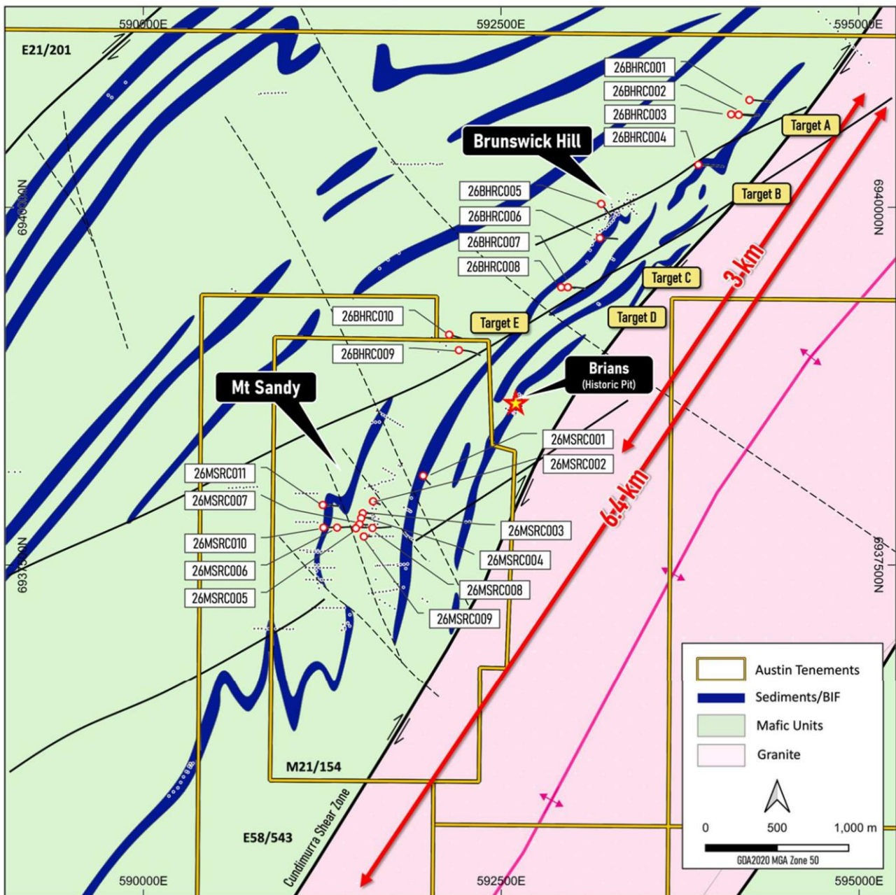
Figure 2. Austin Gold Project drillhole location plan showing the Brunswick Hill and Mt Sandy drilling areas.
