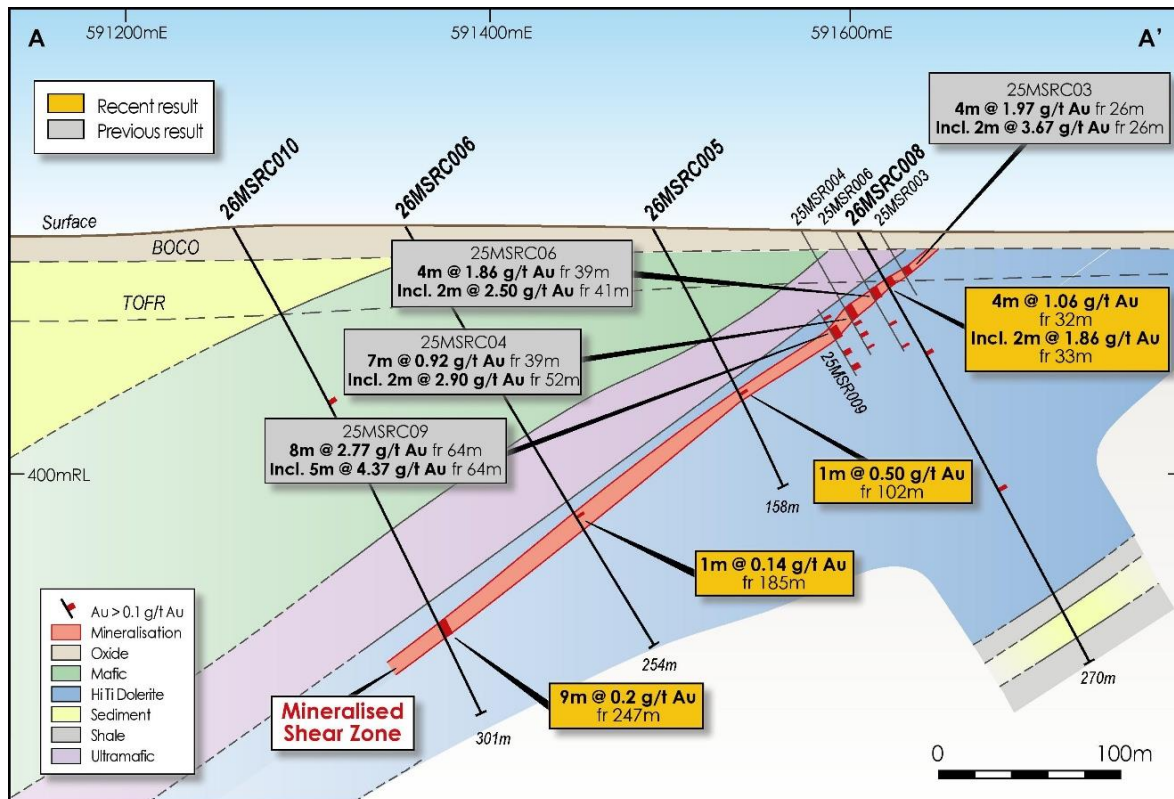
Figure 4. Mt Sandy schematic cross-section A–A' showing recent and previous drilling and the interpreted west-dipping mineralised shear along the hanging-wall contact of the high-titanium dolerite sill.
