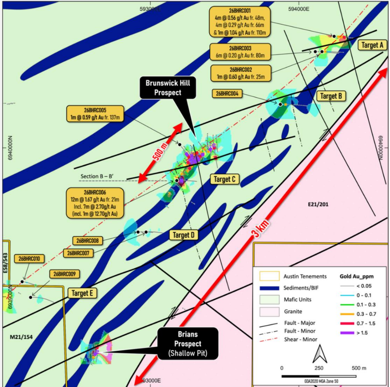
Figure 5. Brunswick Hill drill plan showing recent RC collars, interpreted BIF stratigraphy, the Cundimurra Shear Zone and selected significant gold results.
