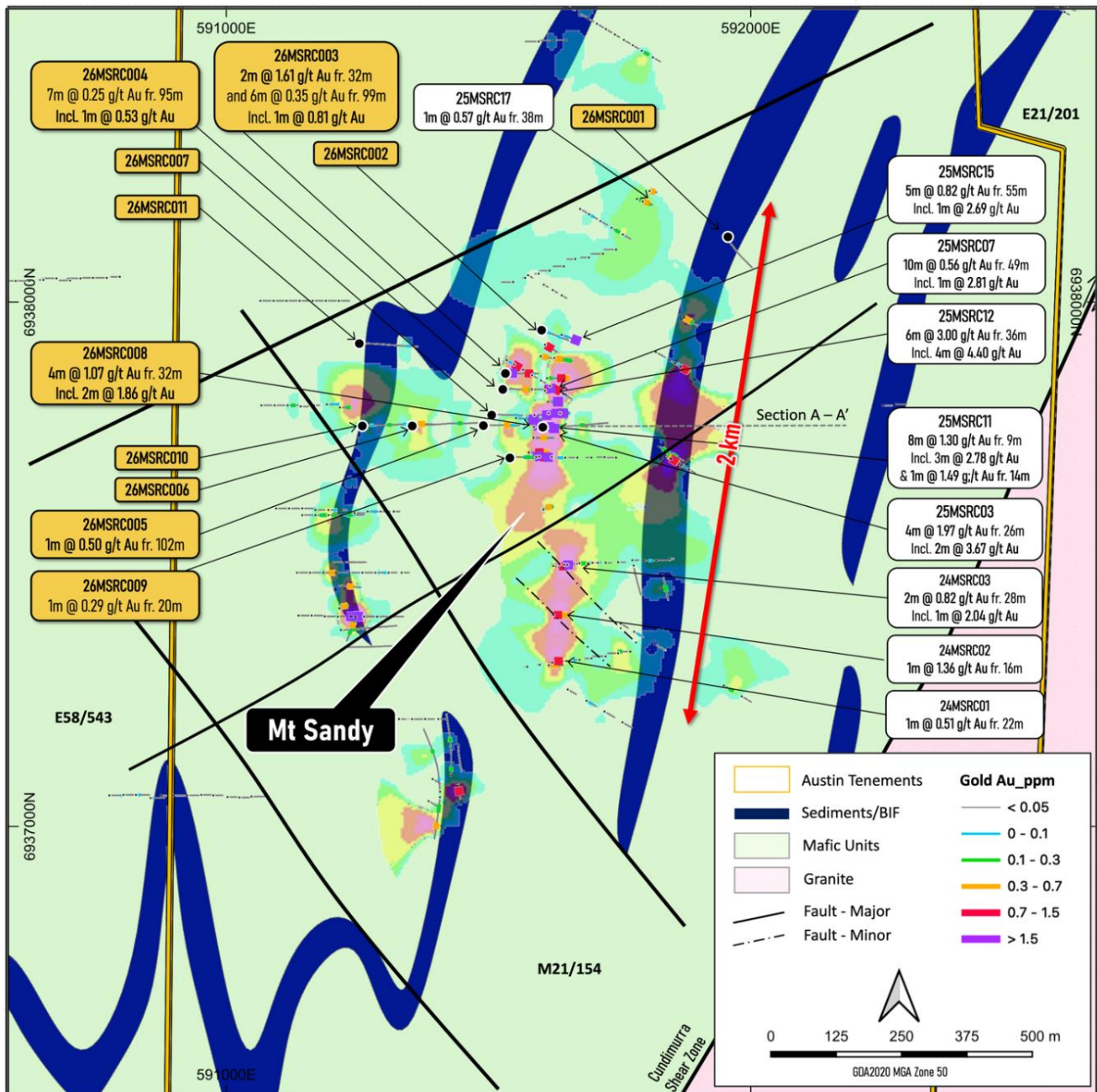
Figure 3. Mt Sandy plan showing extent of gold mineralisation (shown as a gridded drillhole gold image overlying the BIF/mafic stratigraphy). A potential association between gold mineralisation and interpreted northeast- and northwest-trending cross-structures has been observed both within the mafic sequence and bounding BIF units.
