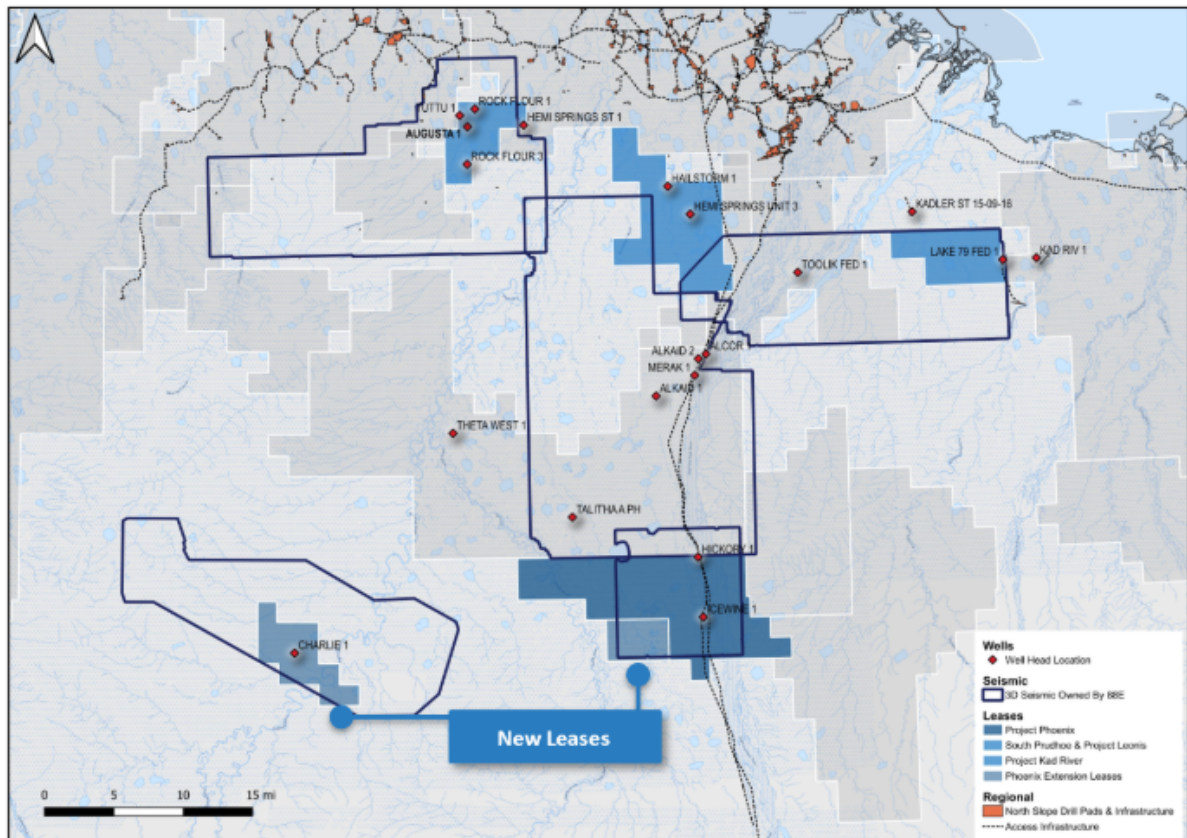
Figure 1: Project Phoenix Extension leases are located immediately South and West of the existing Project Phoenix leases. The leases are covered by the Franklin Bluffs and Icewine West 3D seismic data set, with historical 88E prospectivity identified under review.
