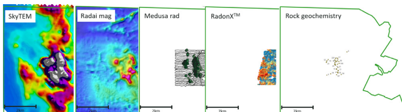
△ Figure 6 Example of the various new exploration datasets collected and integrated over the Storvallfön Project.
