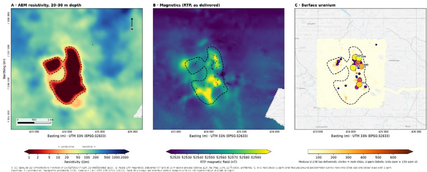
△ Figure 4 Coincident AEM, magnetic and uranium anomalies.
