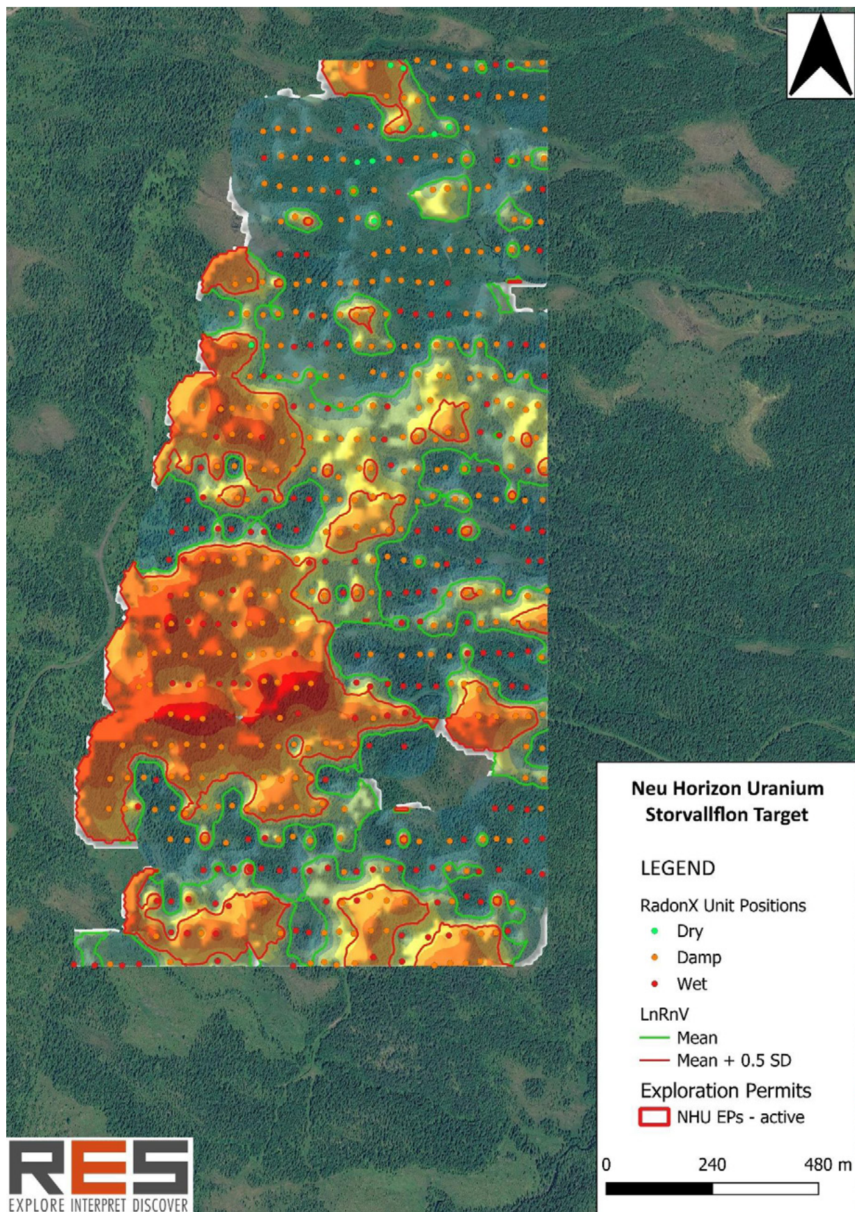
Figure 1: Gridded image of the LnRnV data for the Storvallflon target delineating zones of radon flux. Image taken from RES report RES26/010R.
