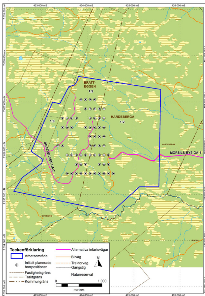
Figure 2: Phase 1 idealised drill collar positions over the Storvallflon Prospect.
