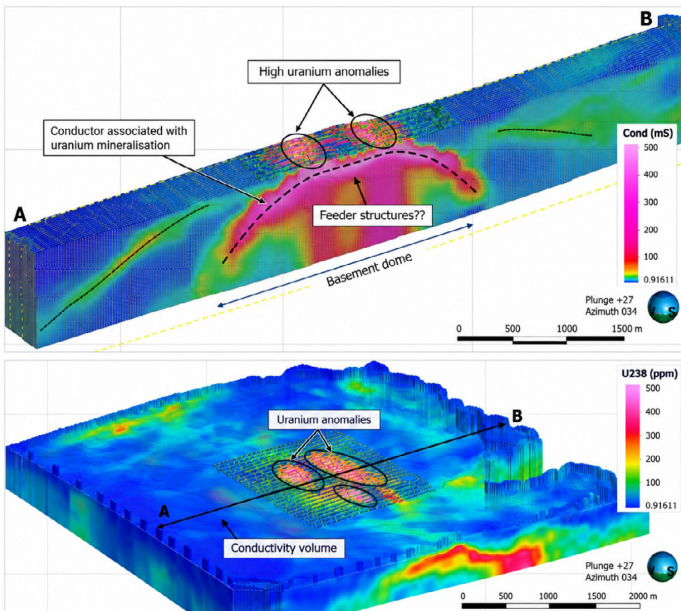
△ Figure 2 Conductivity section across the conductive target highlighting the geometry and association with uranium anomalism on surface (note the uranium scale top-cut is at 500ppm).
