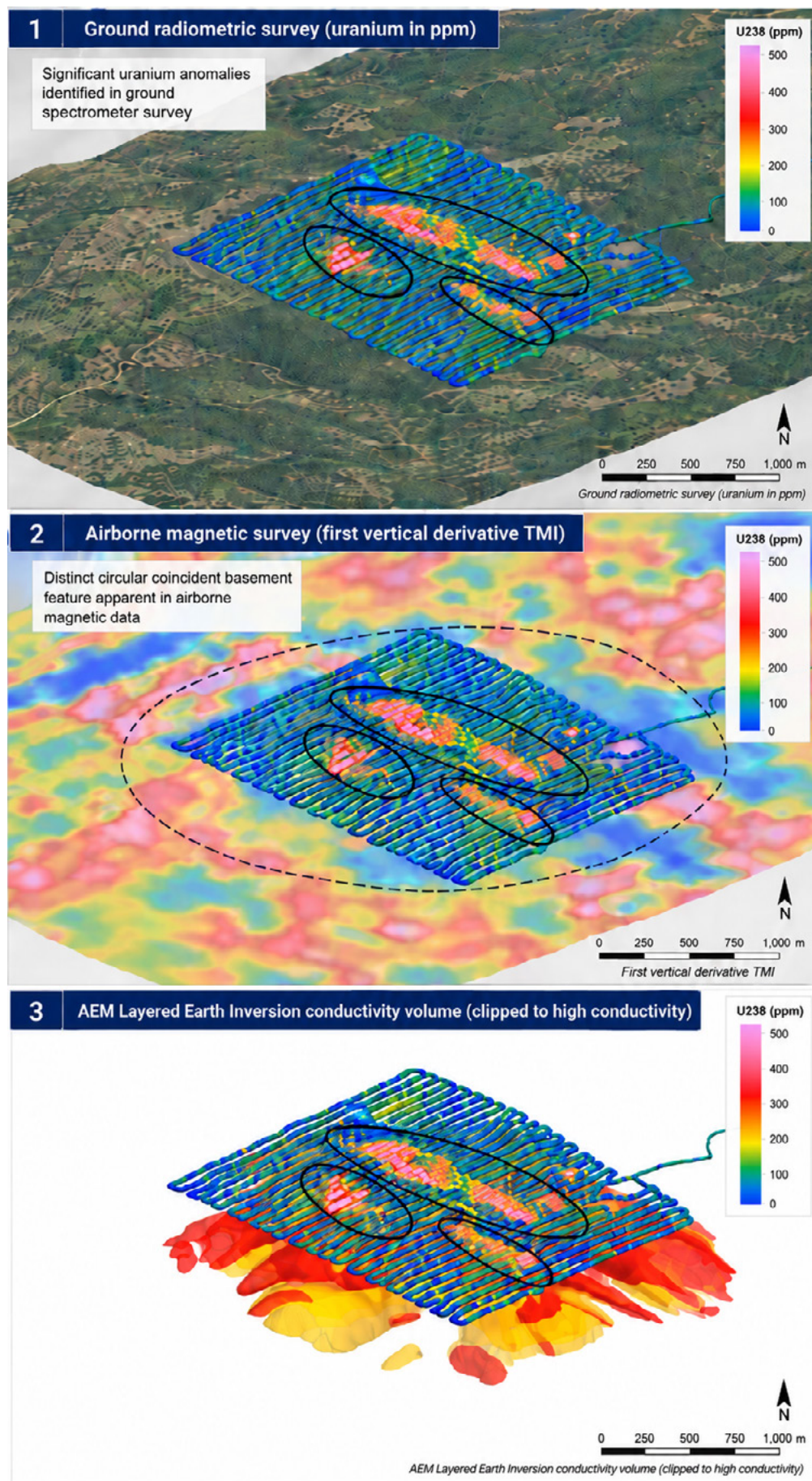
◁ Figure 1 Integration of the ground radiometric, drone magnetic and heliborne EM data delineates highly compelling coincident anomalies across all datasets.
