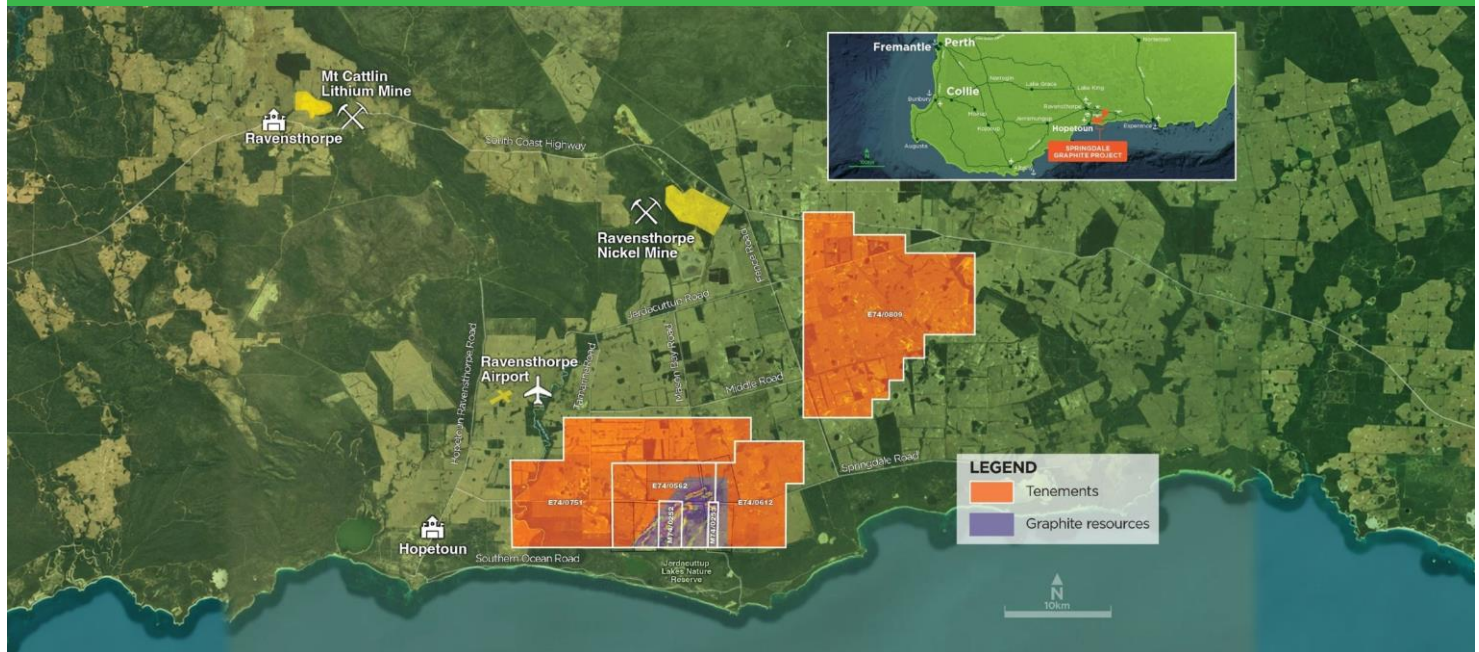
Figure 6: Springdale tenements and graphite resource areas
