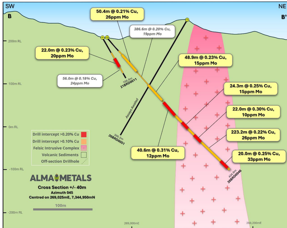
Figure 3 Cross-section for hole 26BRD0046. Location of section depicted as dashed line BB' on Figure 2.
