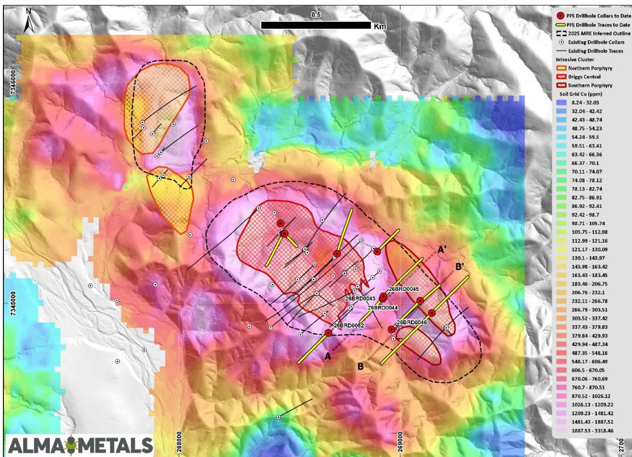
Figure 2 Briggs drill status plan showing holes drilled to date in 2026. Location of cross-sections (Figures 2 and 3) depicted by lines AA' and BB'. Background image is gridded copper in soil sampling overlaid on DEM derived from LIDAR. Interpreted intrusive bodies shown projected to surface.
