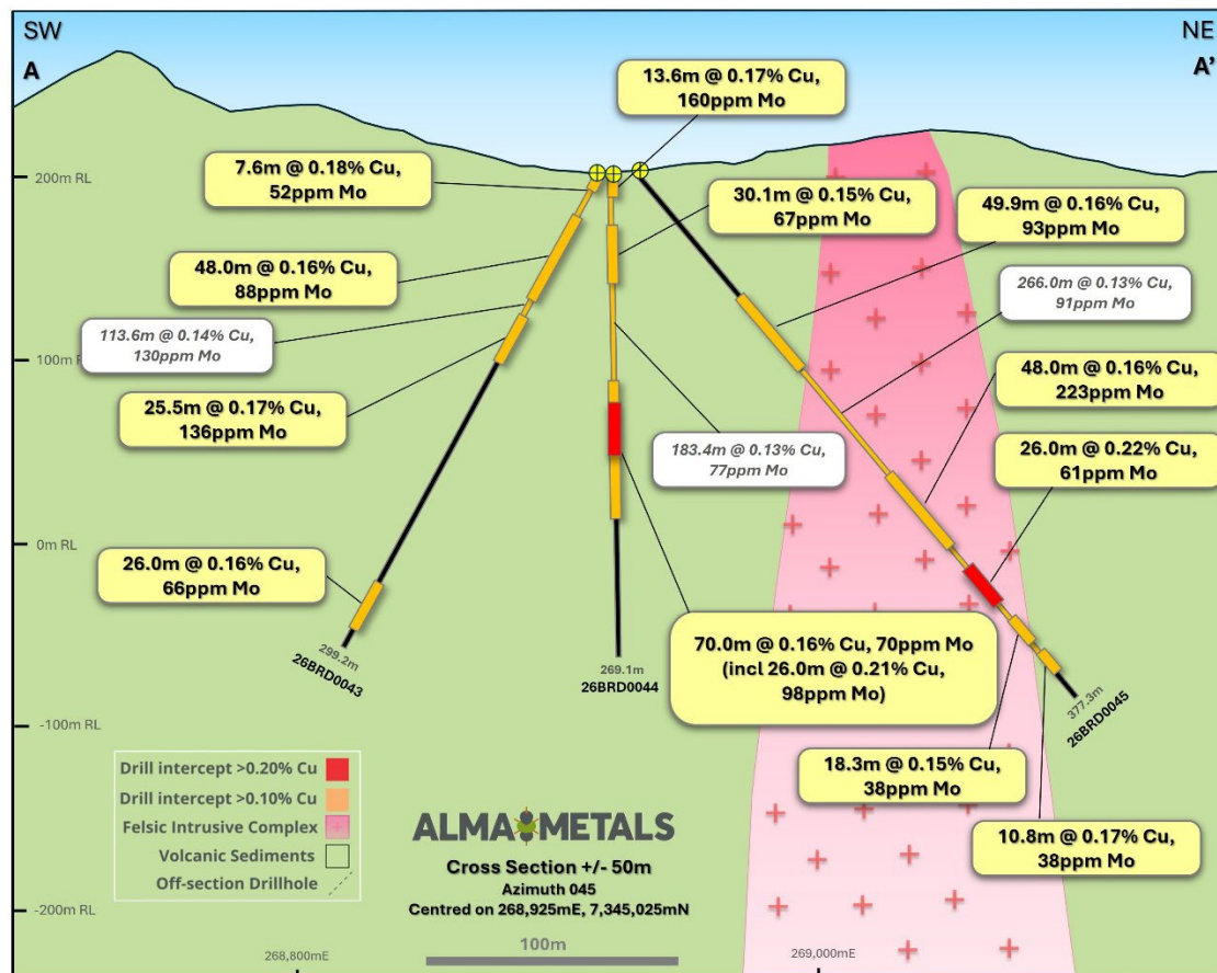
Figure 4 Cross-section for hole 26BRD0046. Location of section depicted as dashed line AA' on Figure 2.
