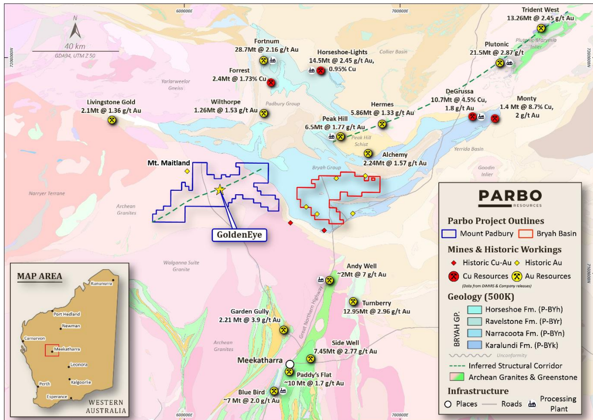
Figure 1 – Regional geology and major gold and copper operations, showing Parbo's Mount Padbury and Bryah Basin Projects
