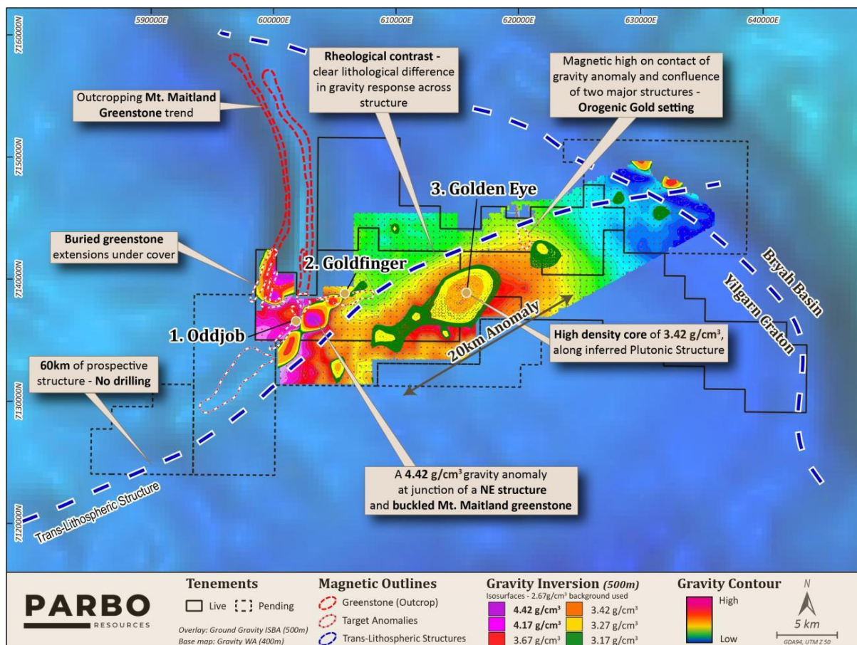
Figure 2 – Mount Padbury Project ground gravity with 500m inversion density isosurfaces, showing the GoldenEye, Oddjob and Goldfinger anomalies along the ~20km gravity corridor (refer ASX announcement dated 8 October 2026)
