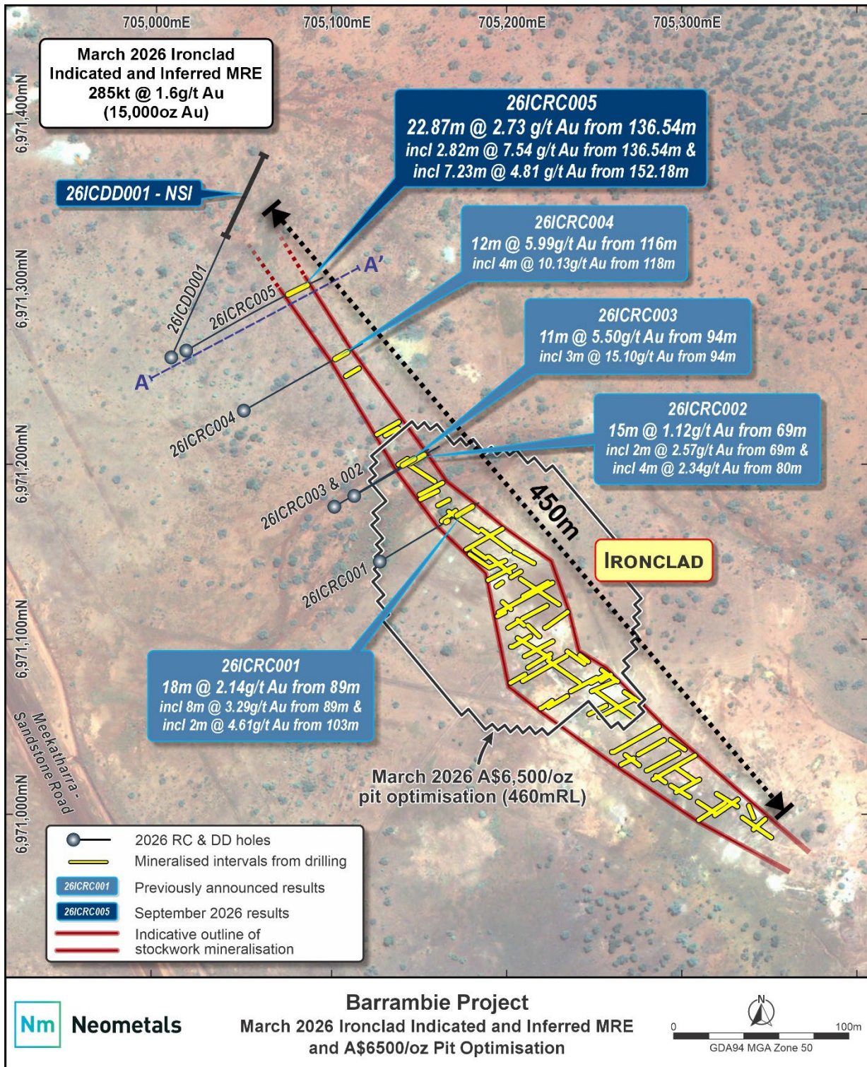
Figure 3: Ironclad plan view showing mineralised interval positions for the Ironclad Deposit. Mineralised intervals for the 2026 drill holes are labelled. Mineralised intervals are defined by a minimum downhole sample intervals of 1m at 0.5g/t Au or above, and maximum internal dilution of 3m. See Appendix 1 for further information regarding the collar locations and drilling details at Ironclad. See also Appendix 2 for further information regarding the significant intercepts at Ironclad
