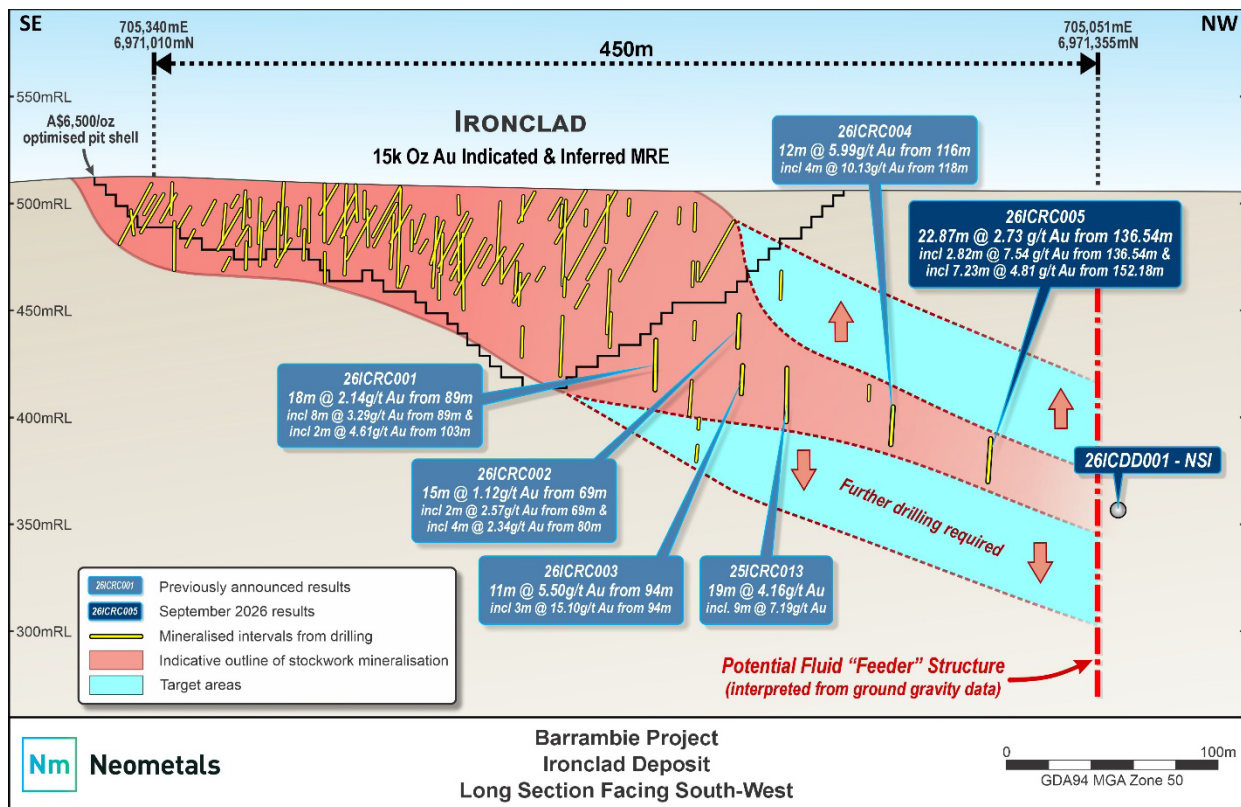
Figure 2: Ironclad long section view showing mineralised interval positions for the Ironclad Deposit. Mineralised intervals for the 2026 drill holes are labelled. Mineralised intervals are defined by a minimum downhole sample intervals of 1m at 0.5g/t Au or above, and maximum internal dilution of 3m
