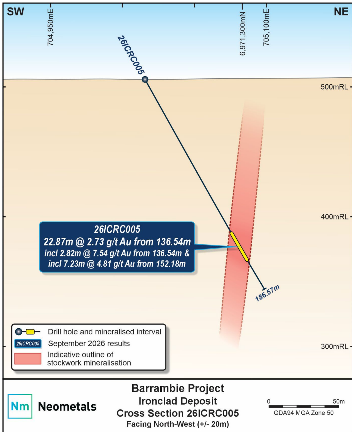
Figure 4: Ironclad Cross Section showing drill hole 26ICRC005 and its reported mineralised interval. The cross section has been provided as an example of the geological context for the drilling results reported in this announcement. See Appendix 1 for further information regarding the collar locations and drilling details at Ironclad. See also Appendix 2 for further information regarding the significant intercepts at Ironclad
