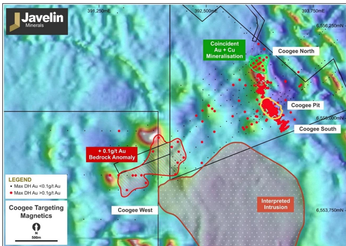
Figure 3: Coogee Project airborne magnetics with historic drilling – maximum downhole gold (>0.1g/t Au).
