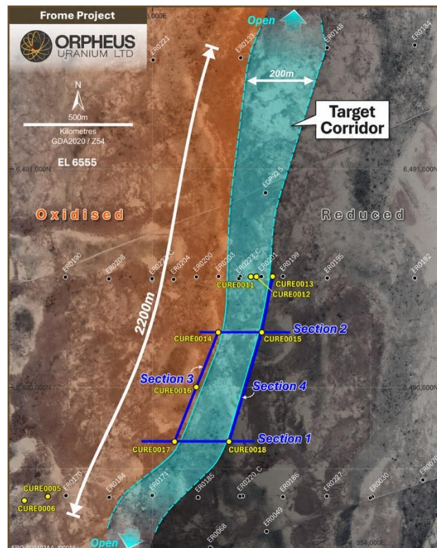
Figure 7: Siccus East Prospect target REDOX corridor with section locations.
