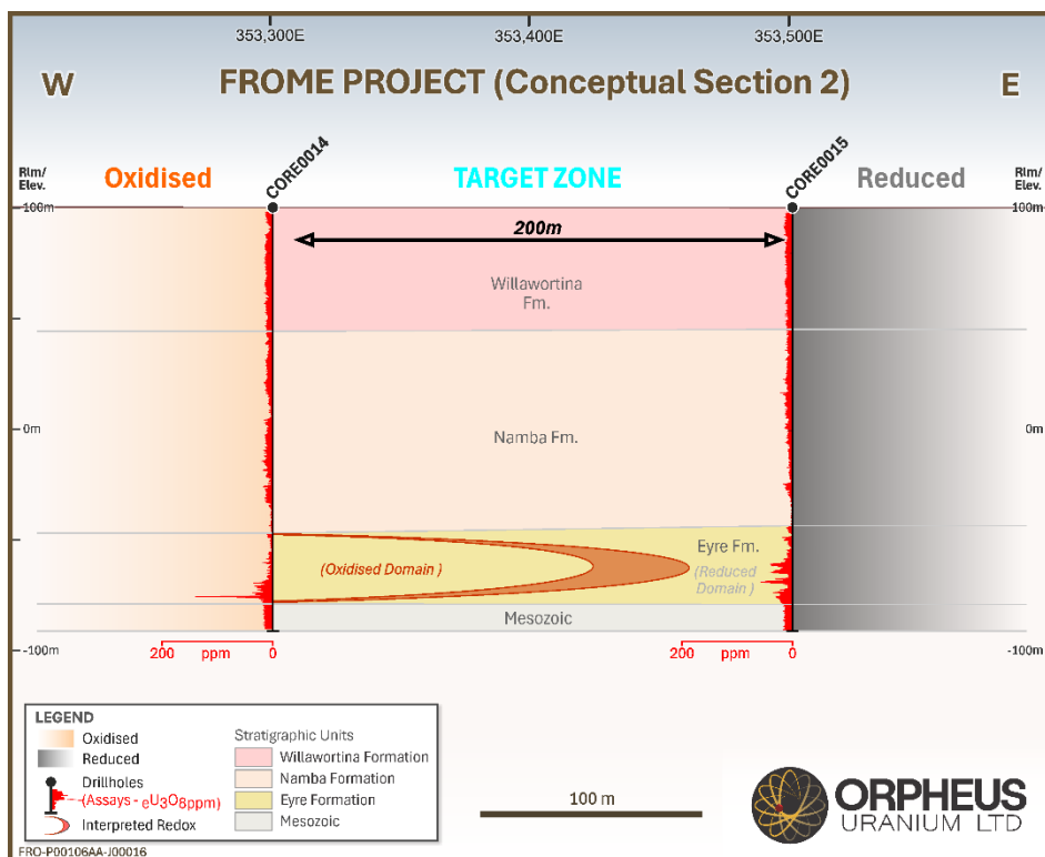
Figure 9: Siccus East Prospect SW-NE section identifying continuity of reduced domain.
