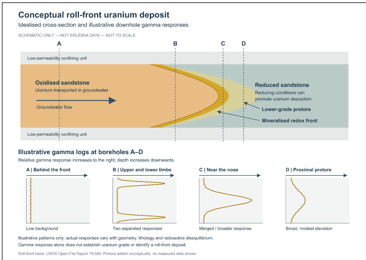
Figure 4: Conceptual cross-section of a sandstone-hosted uranium roll-front system.
