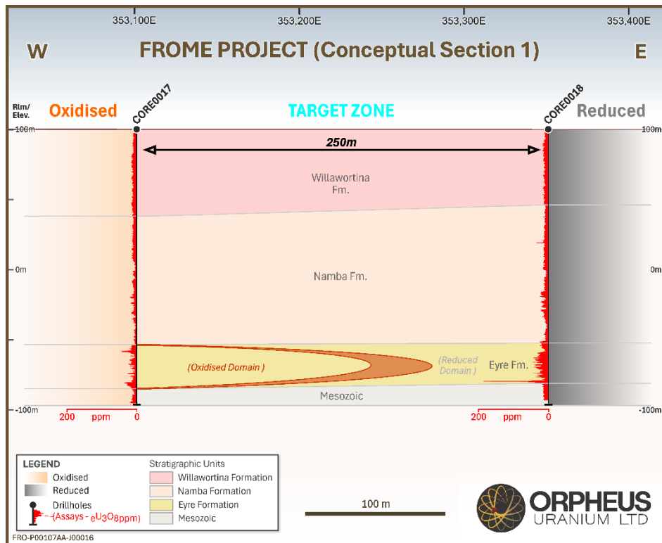
Figure 8: Siccus East Prospect Siccus East Prospect W-E section through REDOX corridor.
