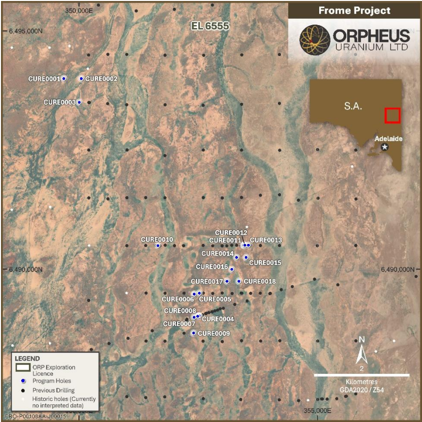
Figure 2: Location of drillholes completed during the program and historical holes at the Erudina Prospect.
