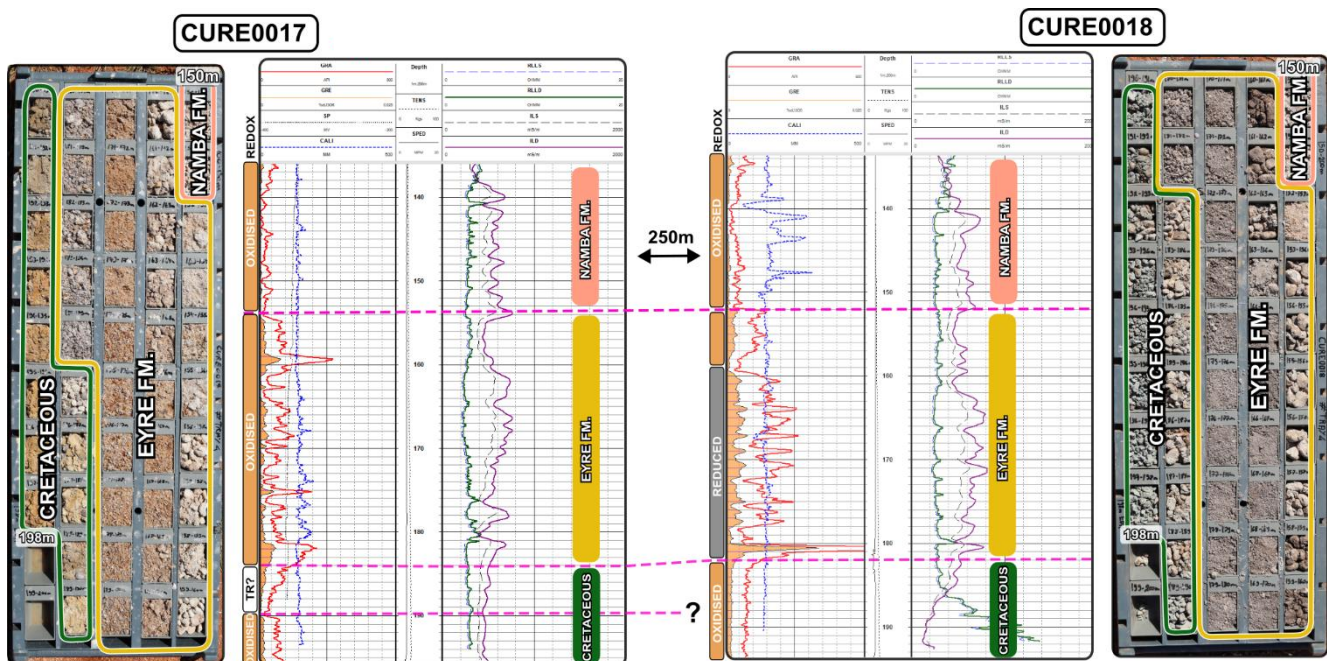
Figure 5: Initial field observations of the oxidised (Orange) Eyre Formation within CURE0017 (left) and reduced (Grey) Eyre Formation within CURE0018 (right), located within Siccus East and defining the extents of the REDOX corridor. The image contains 1m from 150m to total hole depth (198m), whilst the downhole geophysics logs including from top to bottom and left to right (GrA = Gamma in calibrated to API, GrE = Gamma calibrated to %eU 3 O 8 (scale = 0 to 0.025%), SP = Self Potential, CALI = Hole Diameter in mm; RLLS = Resistivity Short, RLLD = Resistivity Deep, ILS = Induction Short and ILD = Induction Deep).
