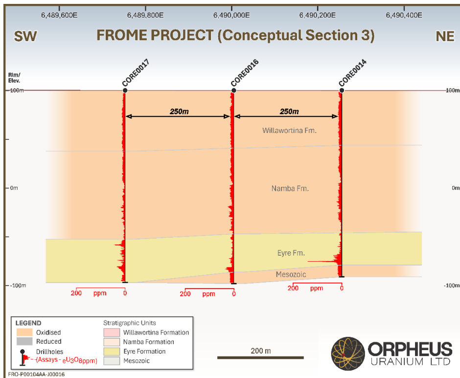
Figure 10: SW-NE section identifying continuity of oxidised domain.
