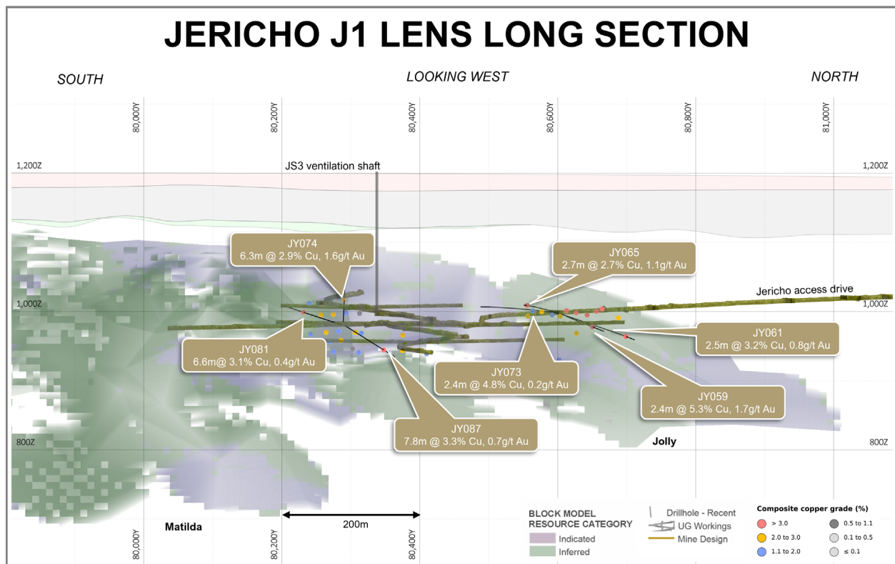
Figure 2. Jolly long section showing recent infill drilling results against Mineral Resource category and completed underground development.
