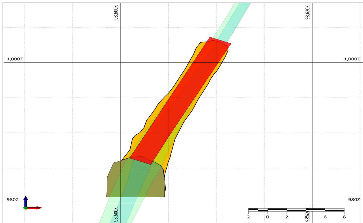
Figure 3: Cross section of Jolly 4975_655 stoping panel. Geology domains shown in green and light blue, stope design in red and Cavity Monitoring System void in orange.
