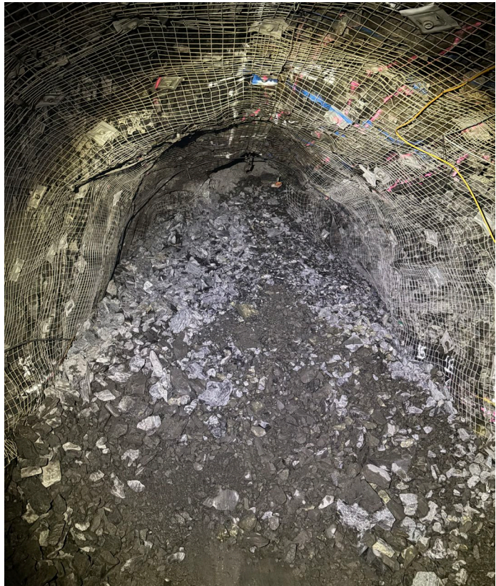
Photo 1. First production stope on 4975 Level (215m below surface) from Jolly shoot at Jericho. Underground drive is 5.5m wide by 5m high (photo area), stope is 19m high and 2.4m wide.
