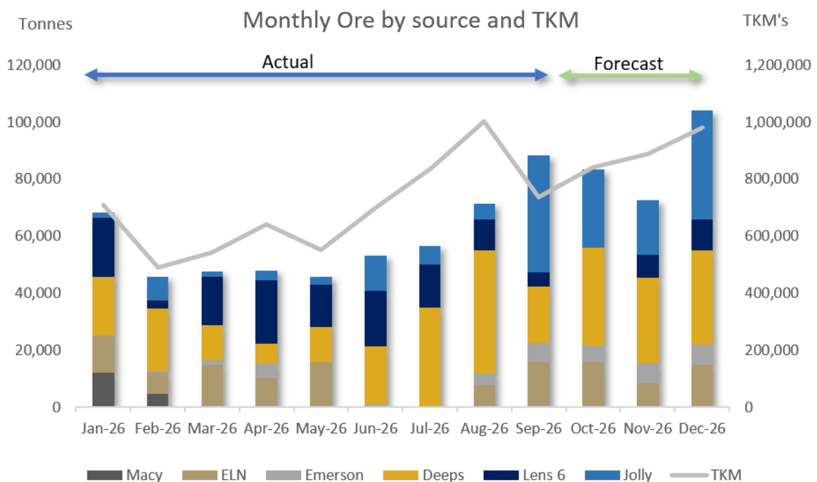
Chart 1. Ore production location and TKM (tonnes of material trucked multiplied by distance trucked).
