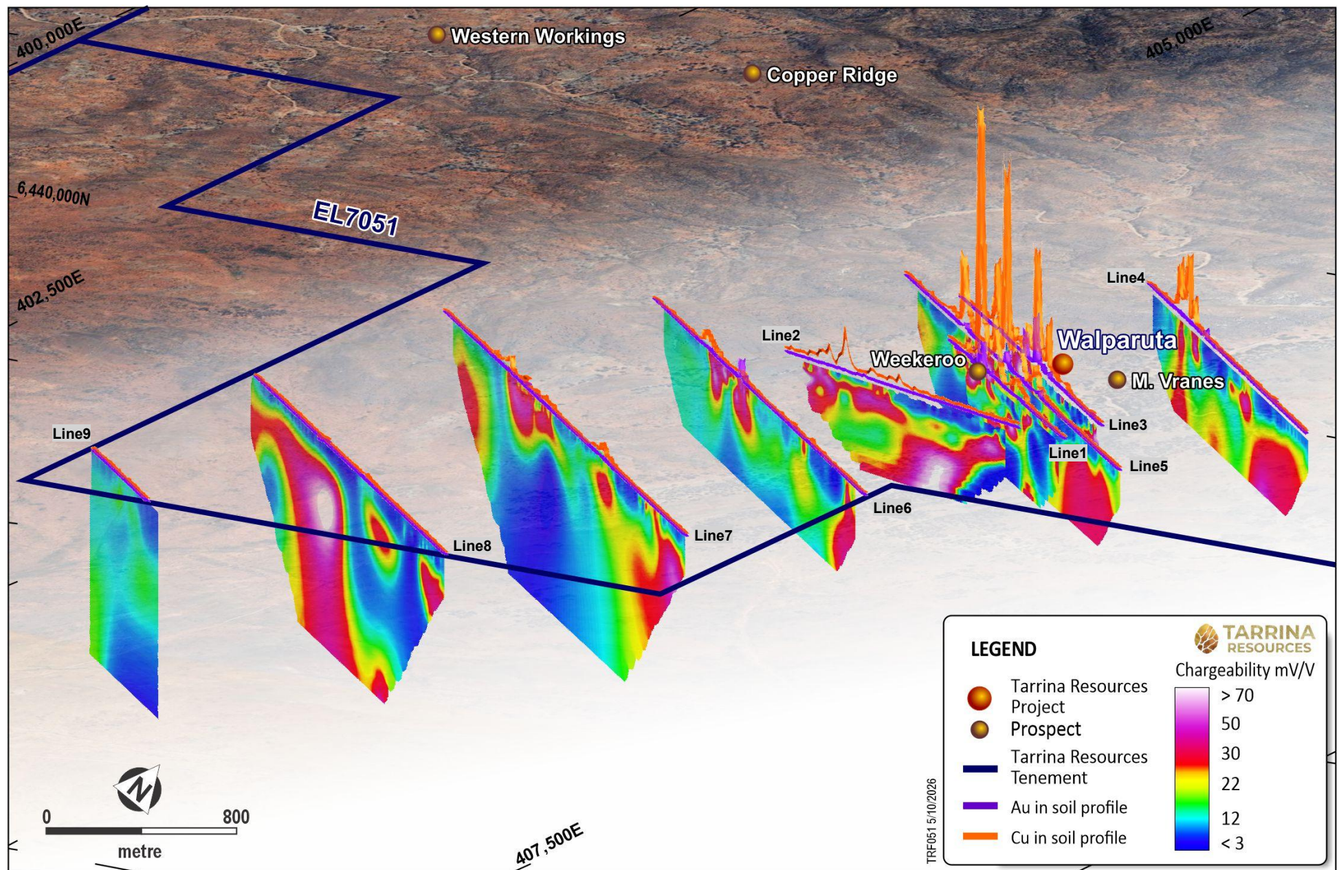
Figure 3. Chargeability anomalies on each IP Line relative to copper and gold anomaly profiles, historic mines and tenement boundary.
