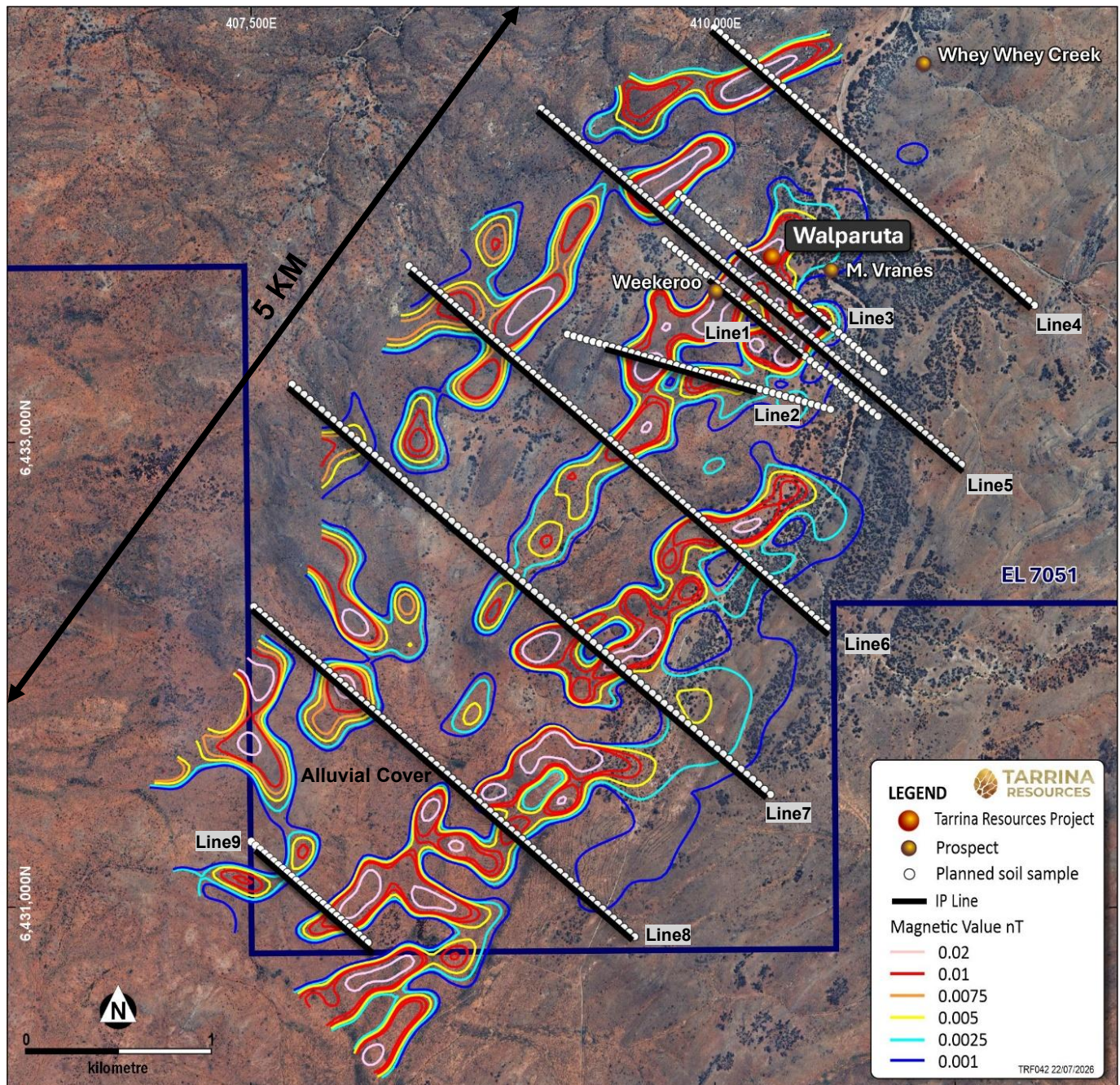
Figure 2. Location of 2D Pole-Dipole Induced Polarisation lines in relation to the 5km long magnetic anomalies and historic mines at Walparuta, showing the area of investigation and location of soil samples.
