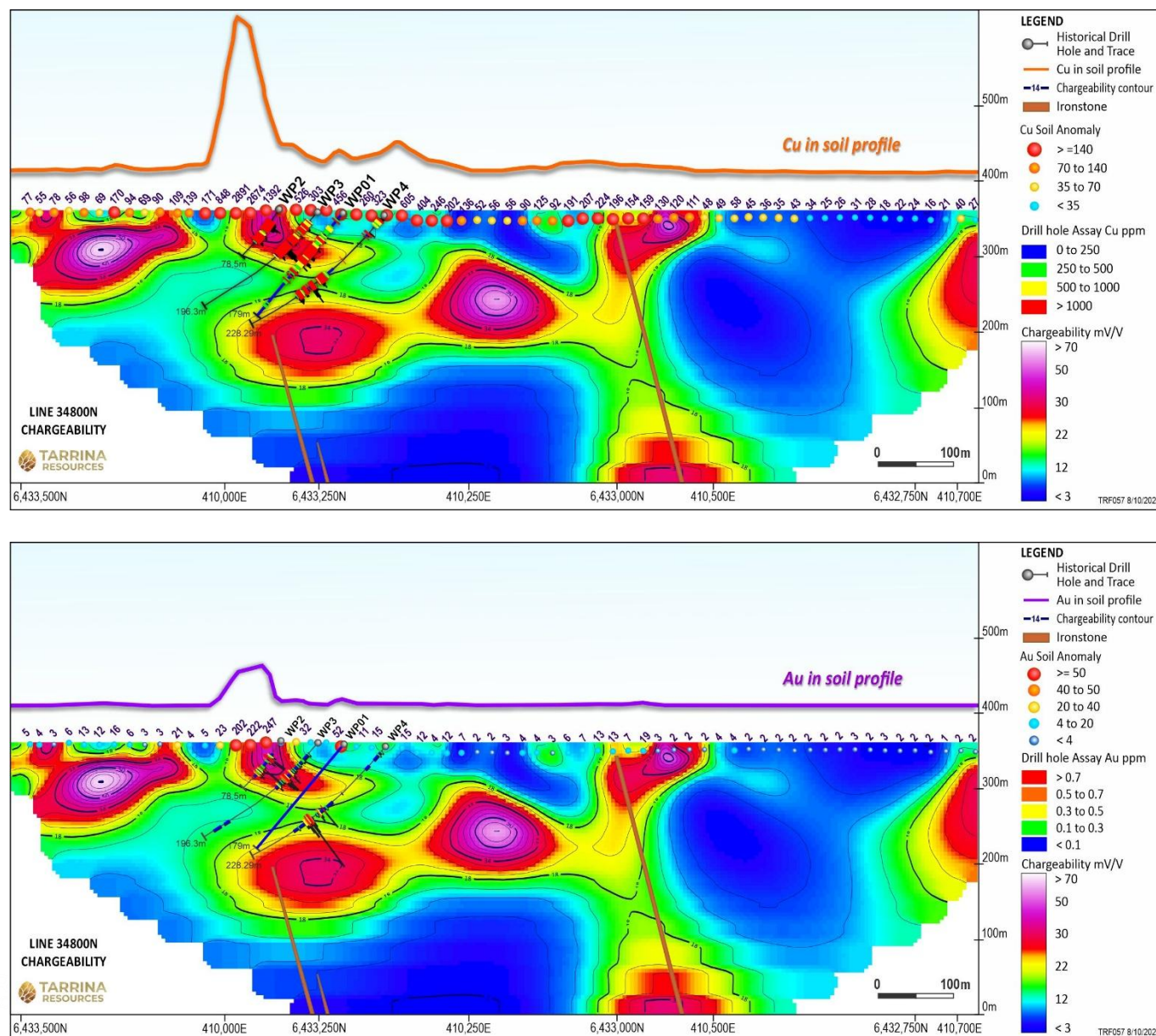
Figure 1. Profile sectional plots of the copper and gold soil geochemistry over the bedrock copper and gold in historic drilling relative to the chargeability anomalies and down dip projection of mapped ironstone units.
