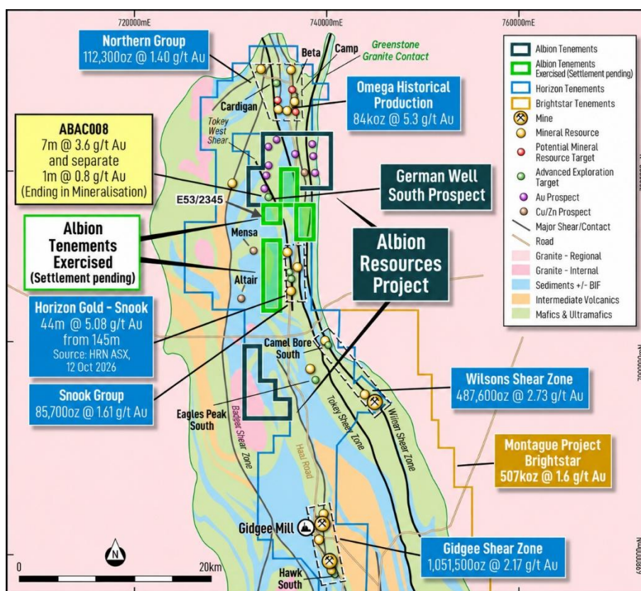
Figure 1: Location of the four exploration licences subject to Albion's exercised option, relative to the Company's existing Gidgee Gold Project, regional geological structures and nearby mineral deposits and prospects. 1,2
